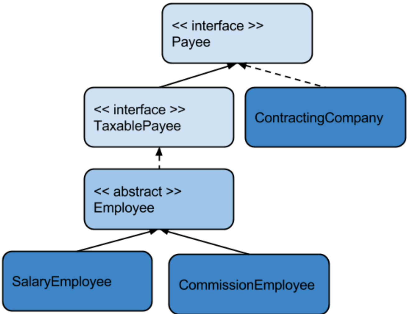
Figure 4.5: screenshot
