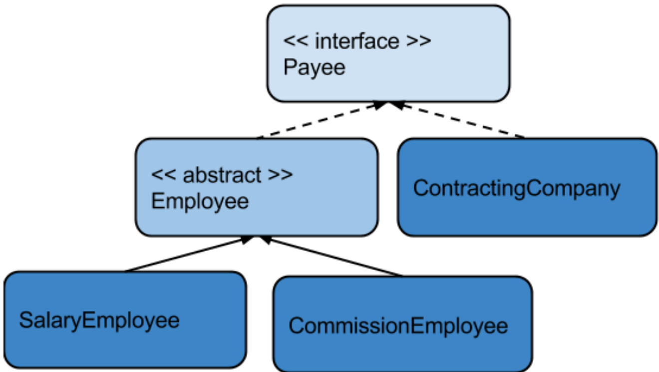
Figure 4.4: screenshot
