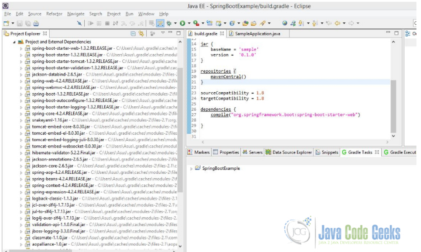
Figure 12.14: Project Dependencies added by Spring Boot.
