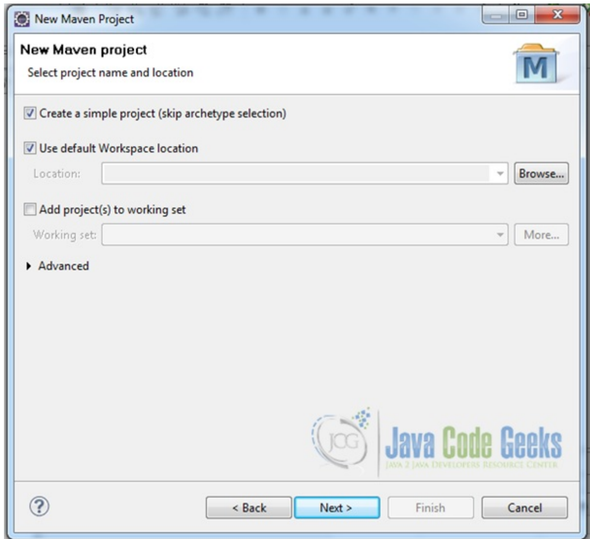
Figure 11.3: Skip ArcheType Selection
