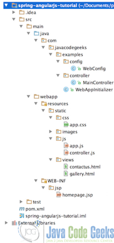
Figure 6.1: Web application directory
