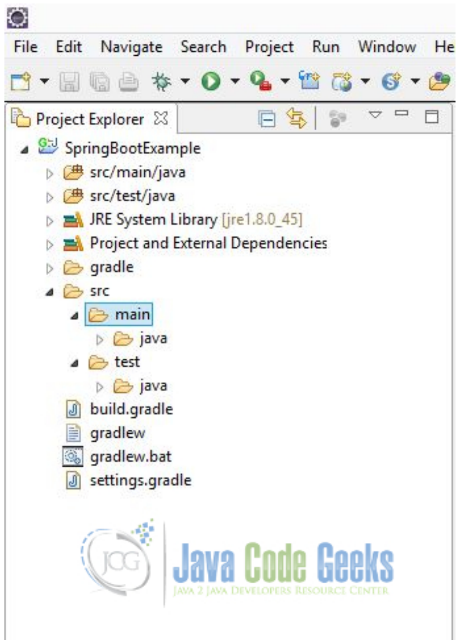
Figure 12.7: Gradle Project Structure
