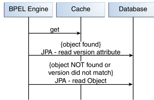
Figure 14–2 Rehydration Process
