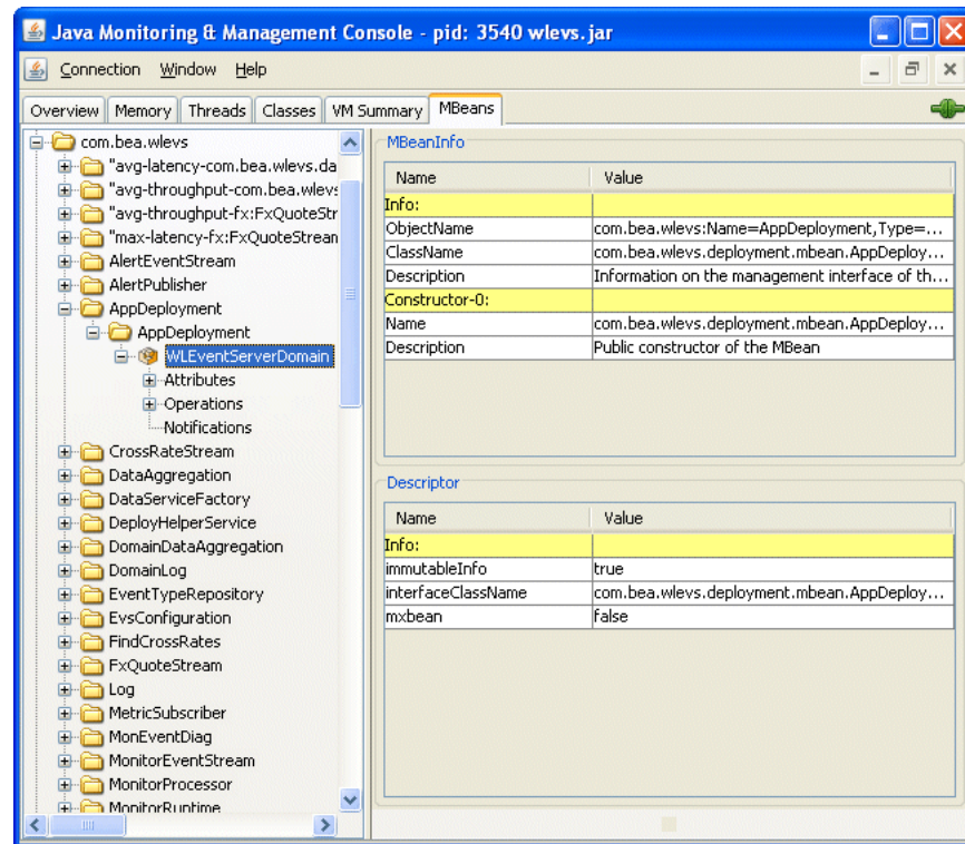
Figure 12–5 JConsole Browser
