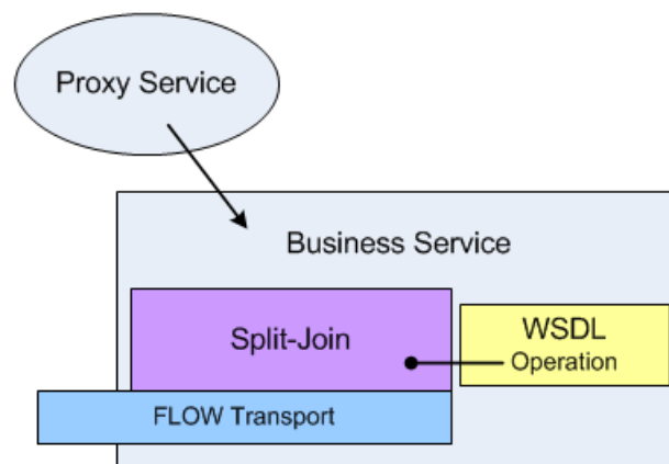
Figure 38–3 Split-Join framework
