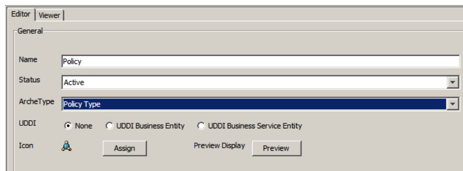
Figure 14–5 Type Manager
