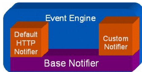
Figure 9–30 Notifier Plug-in
