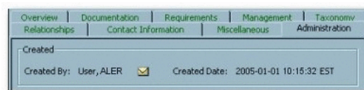
Figure 16–12 Administration Tab
