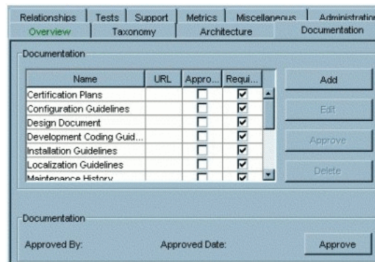
Figure 9–38 Documentation Tab
