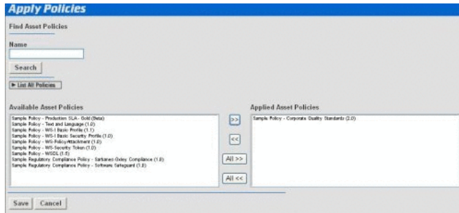
Figure 14–14 Apply Policies
