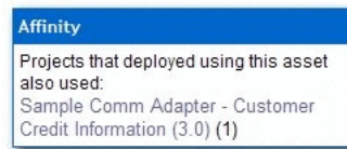
Figure 16–51 Affinity
