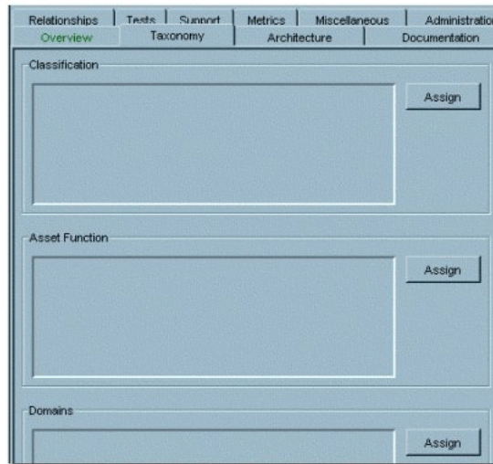
Figure 9–36 Taxonomy Tab
