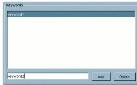
Figure 9–37 Keywords List
