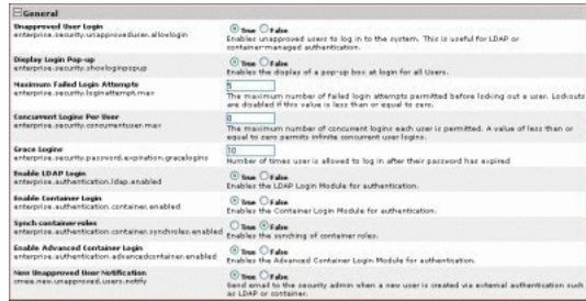
Figure 16–59 General
