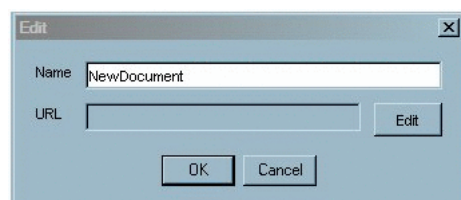
Figure 9–39 Edit Dialog
