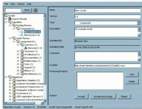
Figure 9–32 Asset Editor
