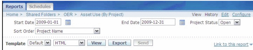
Figure 14-25 Reports Tab
