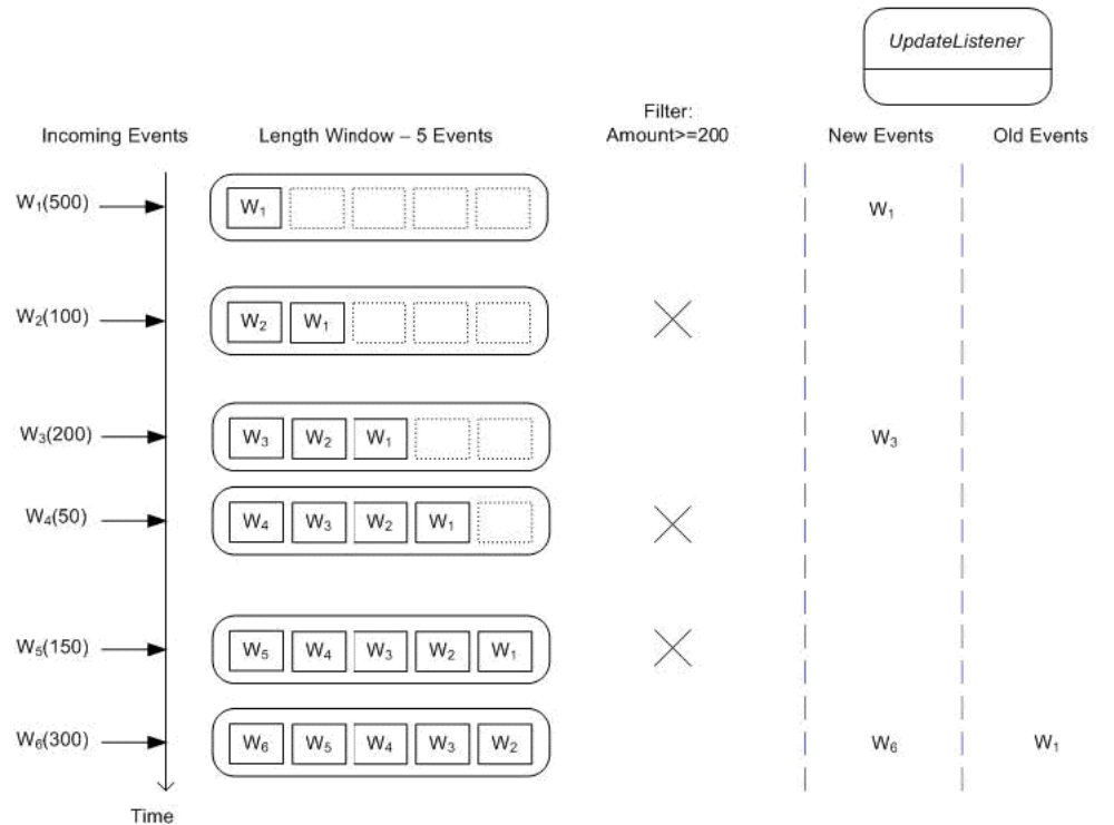
Figure 1–6 Events Arriving in a Row-Based Sliding Window
