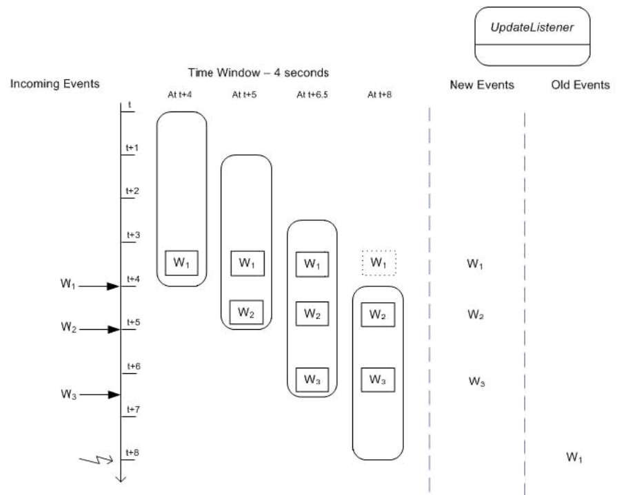
Figure 1-3 Example Time-Based Sliding Window
