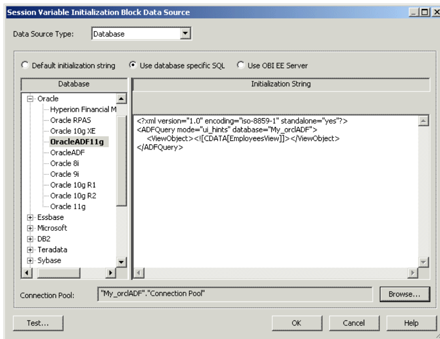
Figure 6–3 Setting Up a Session Variable Initialization Block Data Source with an Oracle ADF UI Hints Query
