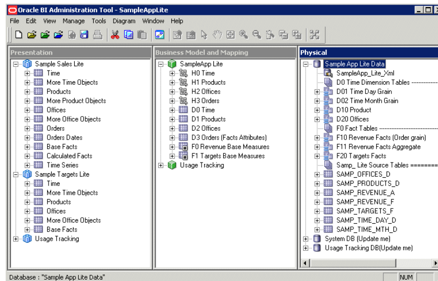
Figure 2–1 Example Administration Tool Main Window
