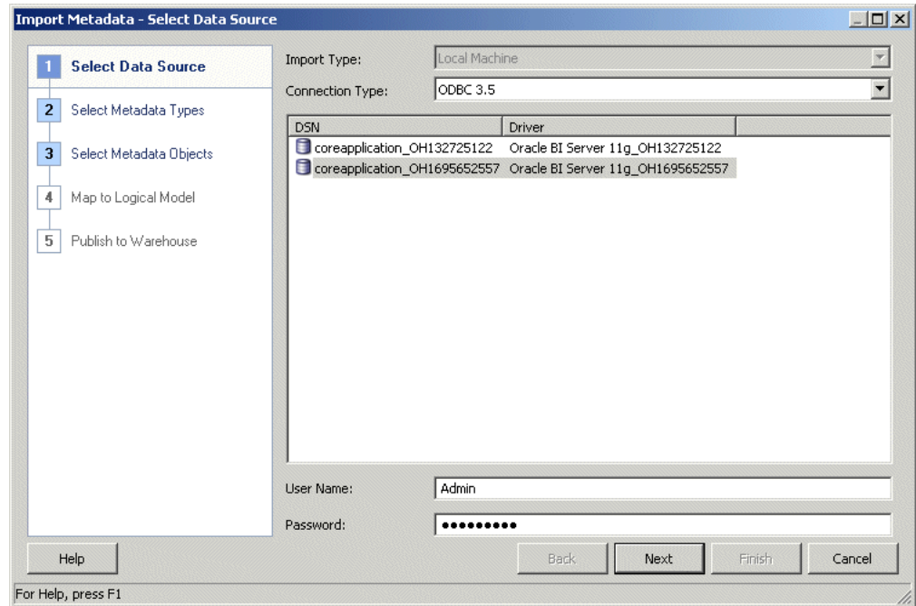
Figure 5–1 Import Metadata Wizard: Relational Data Source
