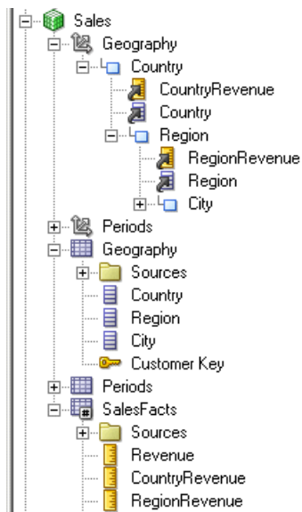
Figure 10-3 Example of Business Model in the Business Model and Mapping Layer
