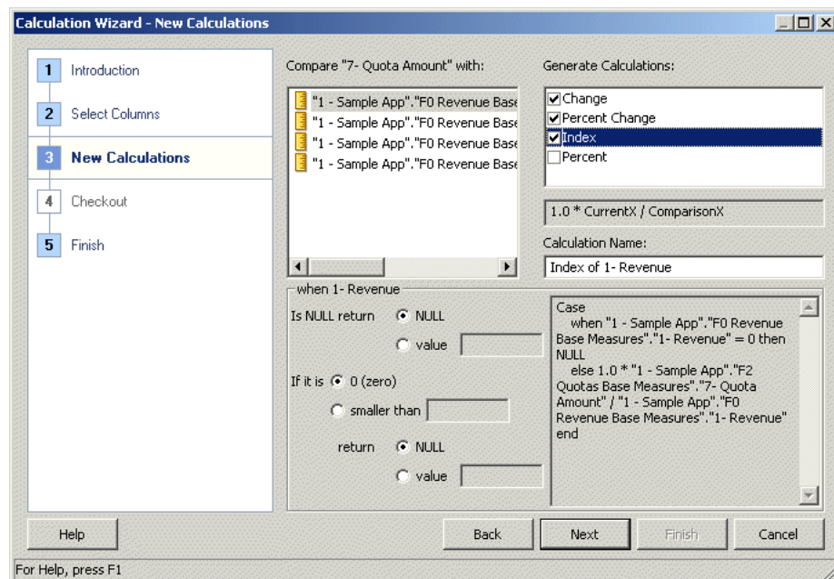
Figure 18–6 New Calculations Screen of Calculation Wizard
