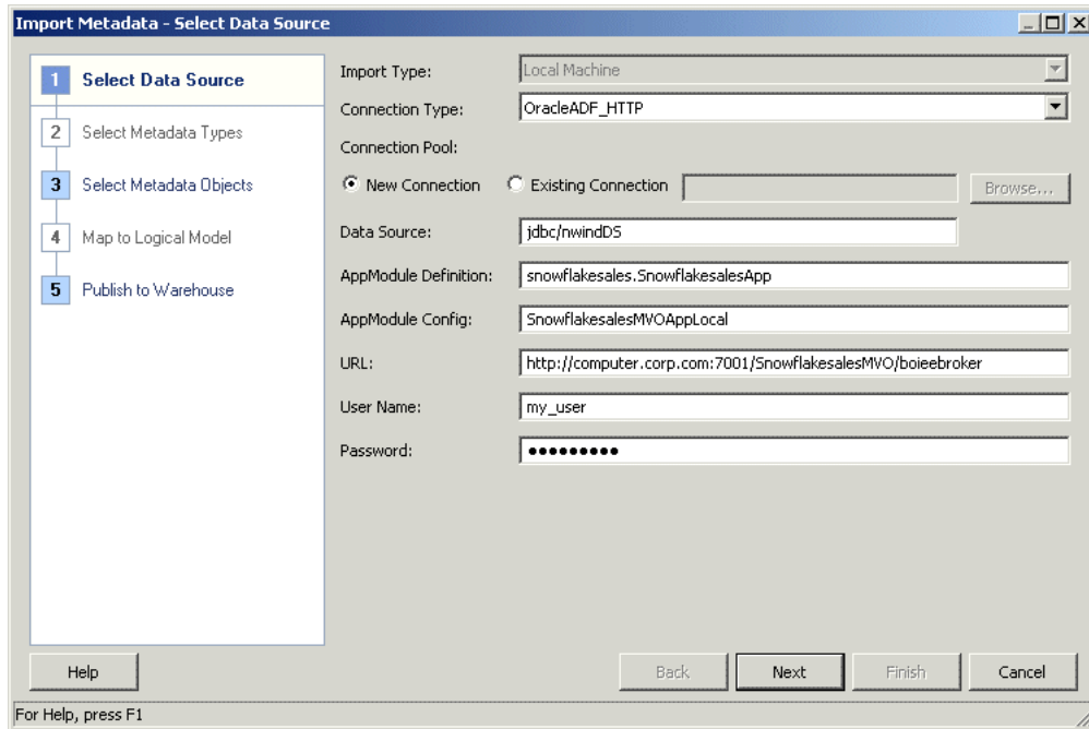
Figure 6–1 Import Metadata Wizard: ADF Business Component Data Source
