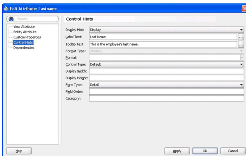
Figure 6–2 Edit Attribute Dialog in JDeveloper for Label and Tooltip Options
