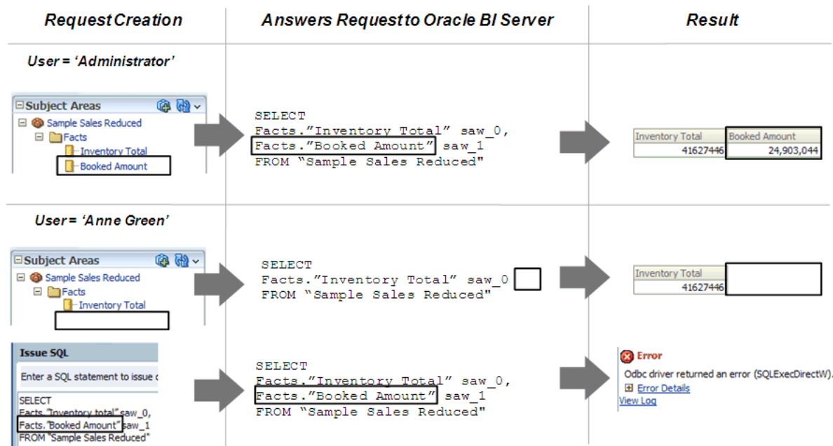
Figure 14–4 Object Permission Enforcement in the Oracle BI Server
