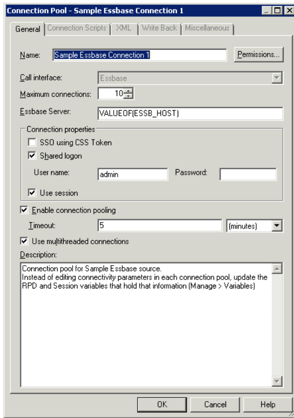
Figure 7–2 General Tab of the Connection Pool Dialog: Essbase Data Source
