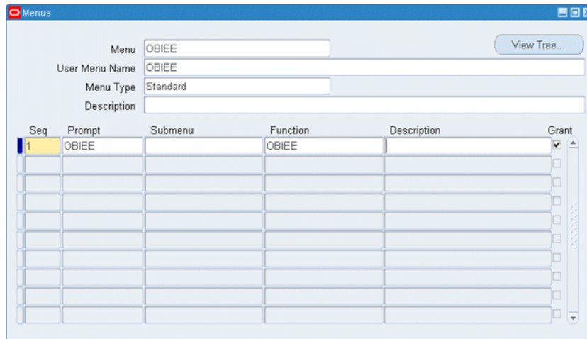
Figure 6–4 Menu Dialog
