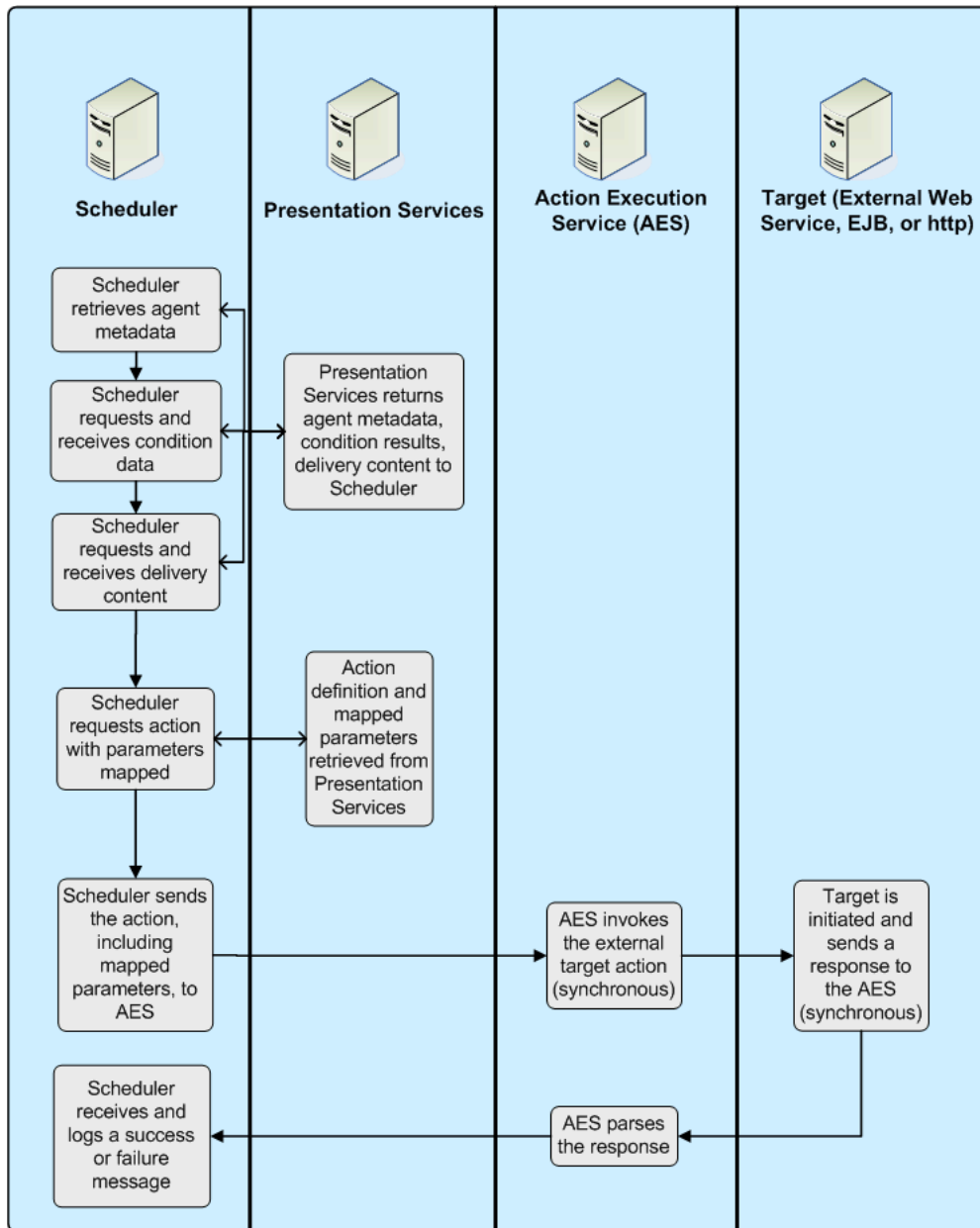
Figure 5–6 Invoke Agent Process Flow
