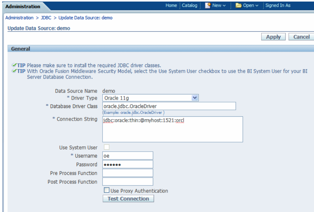
Figure 9–3 JDBC Connection Page
