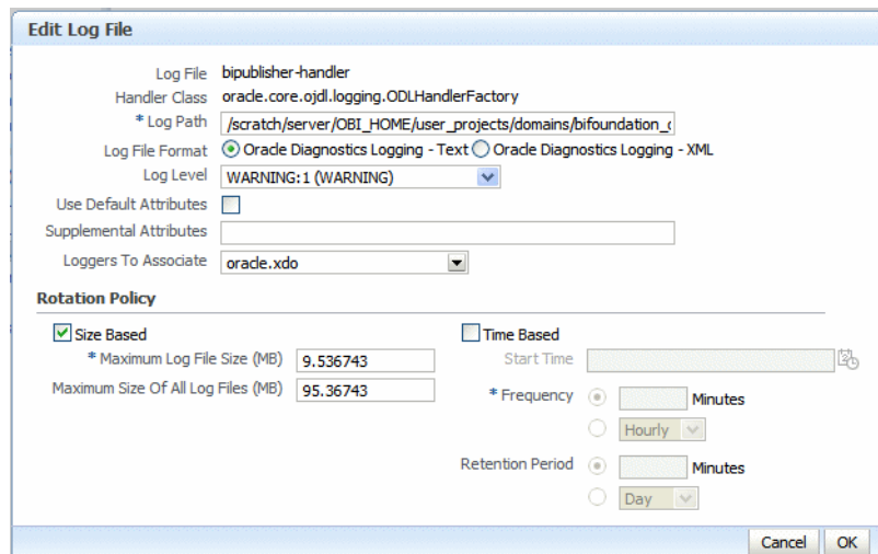
Figure 13–3 Edit Log File Dialog
