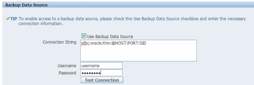
Figure 9–4 Backup Data Source Region
