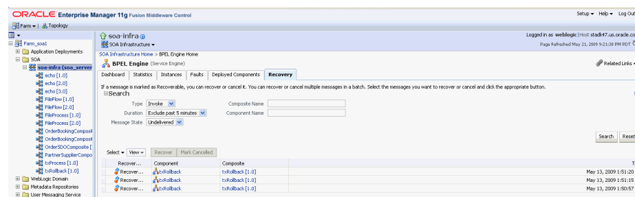
Figure 5–11 BPEL PM Instance Recovery using Oracle Enterprise Manager
