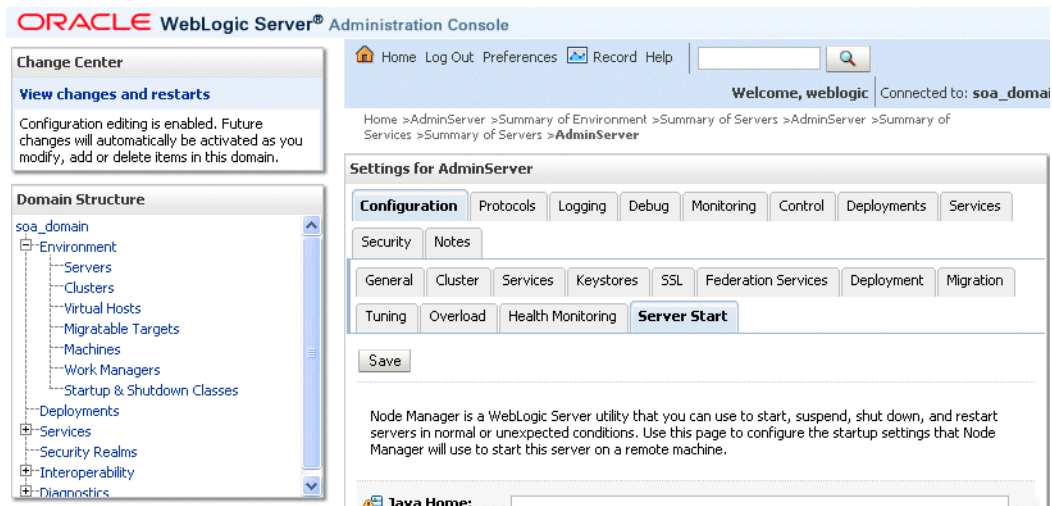
Figure 5–51 Setting the Hostname Using the Start Server Tab of Oracle WebLogic Server Administration Console
