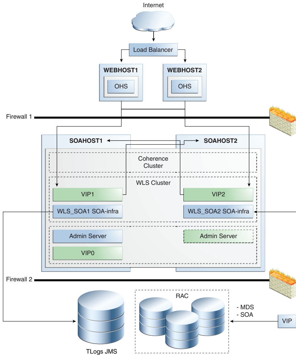
Figure 5–41 Oracle SOA Service Infrastructure High Availability Architecture
