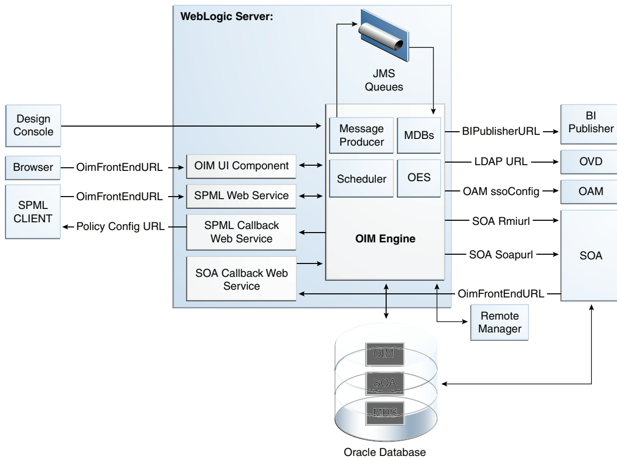
Figure 8–16 Oracle Identity Manager Component Architecture
