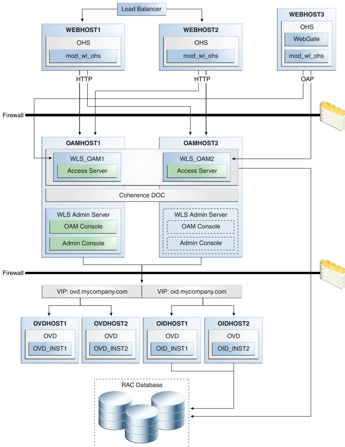
Figure 8–13 Oracle Access Manager High Availability Architecture
