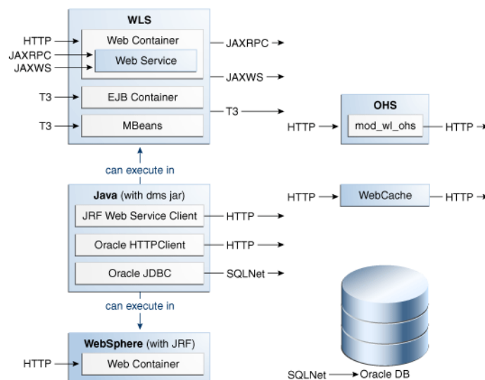
Figure 6–2 DMS Execution Context Communication Protocols
