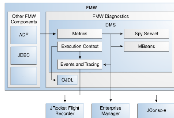
Figure 6–1 DMS Interactions with Oracle Fusion Middleware Components
