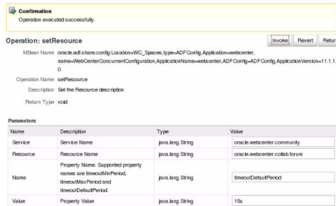
Figure 27-3 System MBean Browser - setResource
