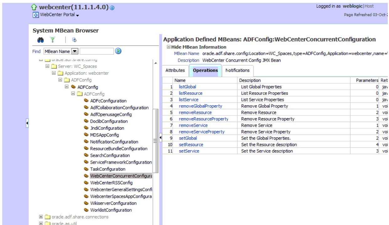
Figure 27–1 System MBean Browser - WebCenterConcurrentConfiguration
