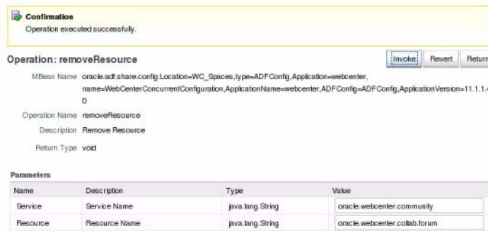
Figure 27-4 System MBean Browser - removeResource
