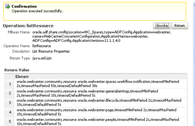
Figure 27-2 System MBean Browser - listResource
