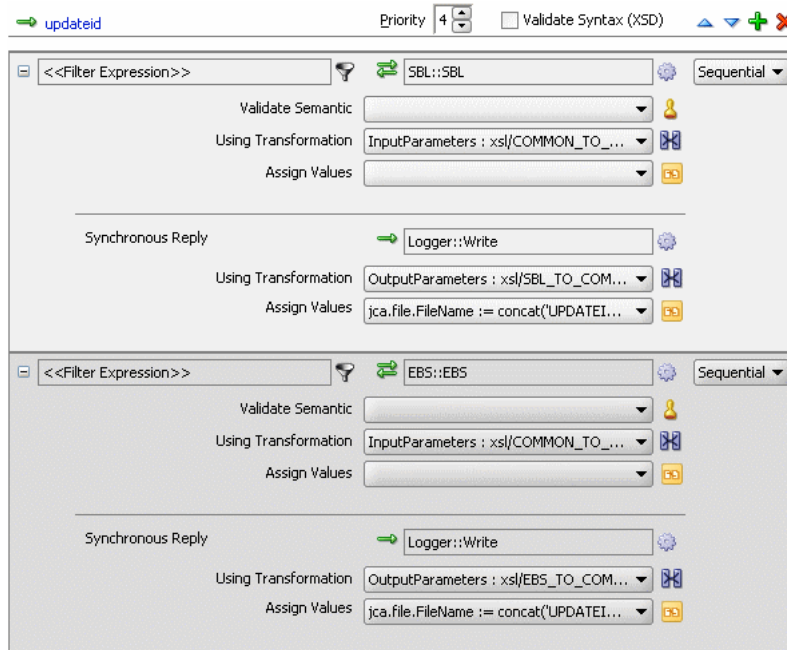
Figure 47–45 Updateid Operation with SBL and EBS Target Service
