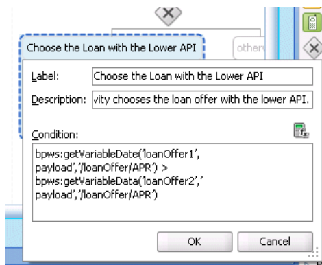
Figure 11-4 Completed Condition Dialog
