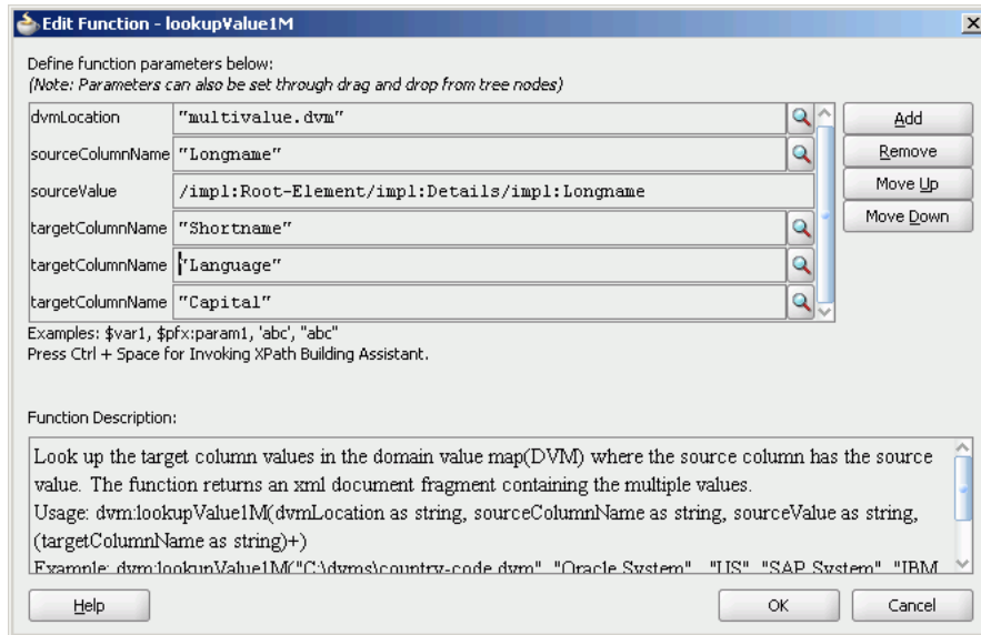
Figure 45–24 Edit Function-lookupValue Function Dialog: Multiple Value Lookup Use Case
