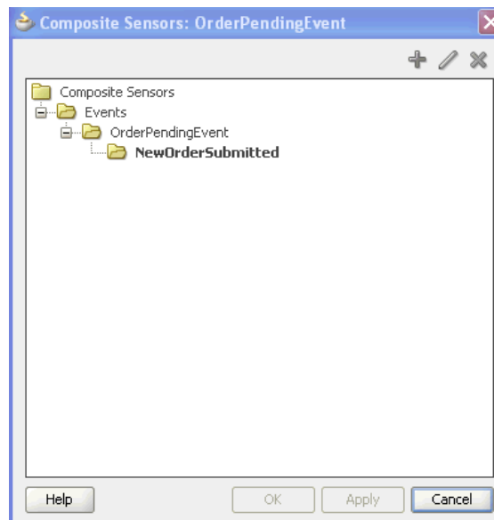
Figure 48-2 Composite Sensors Dialog for the Selected Service Component
