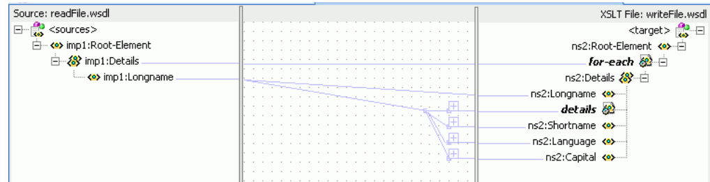
Figure 45–22 imp1:Root-Element To ns2:Root-Element Transformation
