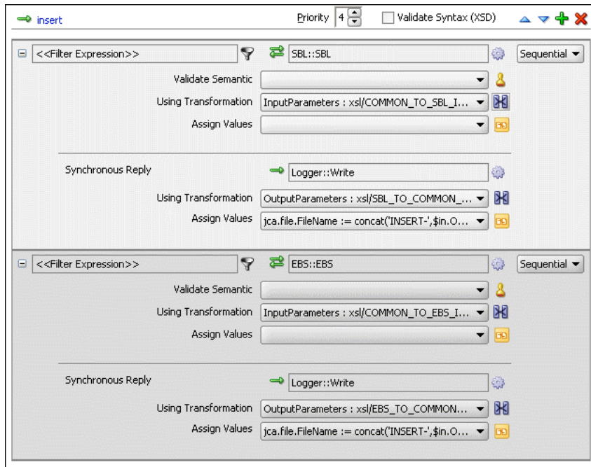
Figure 47–38 Insert Operation with SBL and EBS Target Services
