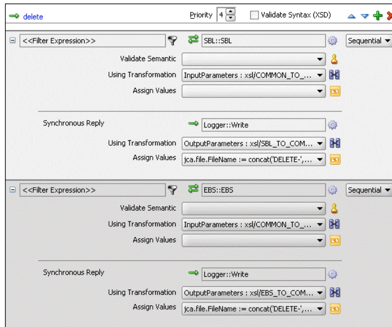
Figure 47–41 Delete Operation with SBL and EBS Target Service
