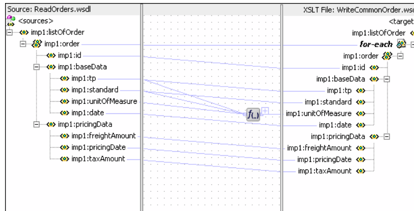
Figure 45–16 Complete imp1:listOfOrder To imp1:listOfOrder Transformation
