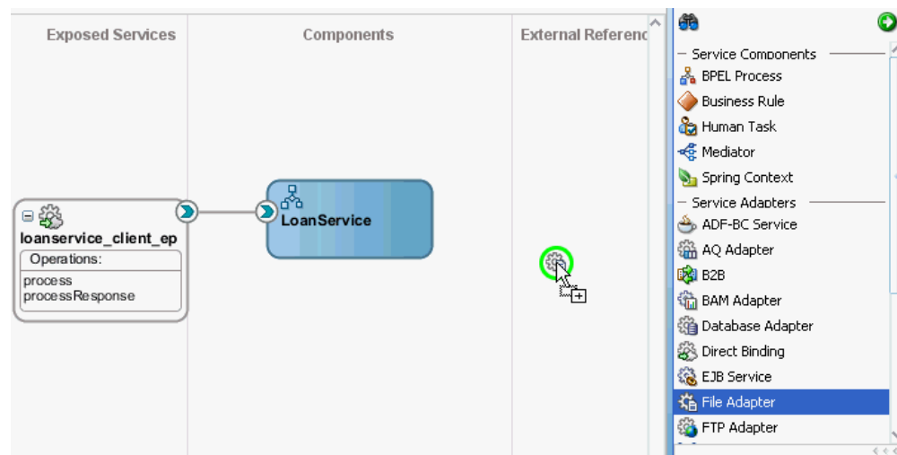
Figure 35–6 Integration of a Web Service Binding Component into a Composite
