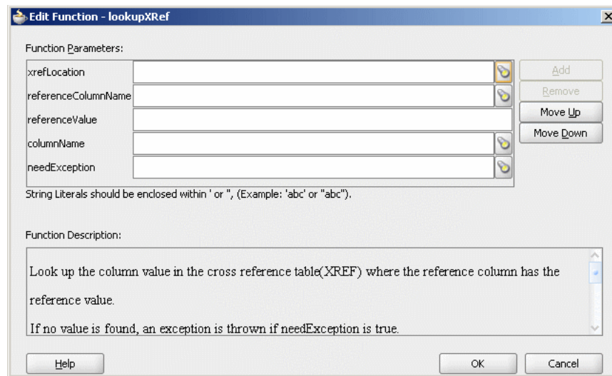
Figure 47–10 Edit Function – lookupXRef Dialog
