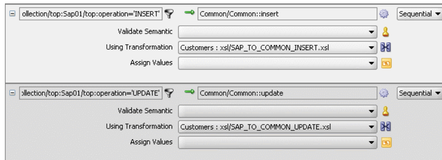
Figure 47-28 Insert Operation and Update Operation
