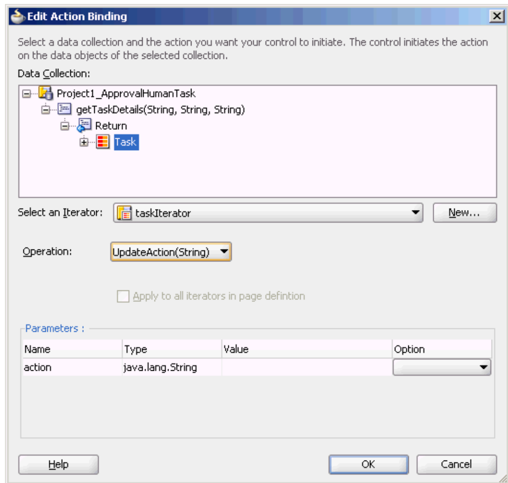
Figure 29–23 Select the Data Collection and Action
