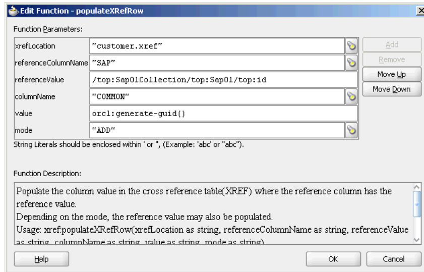
Figure 47–9 Populated Edit Function – populateXRefRow Dialog
