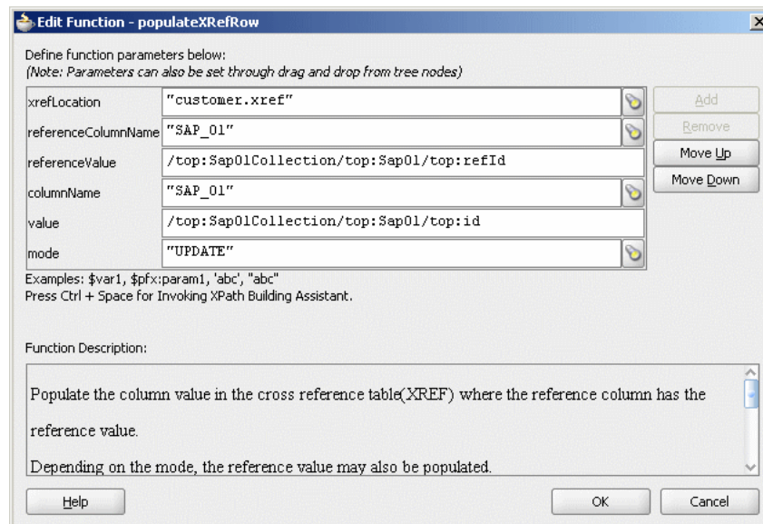
Figure 47–29 Edit Function – populateXRefRow Dialog: XrefCustApp Use Case
