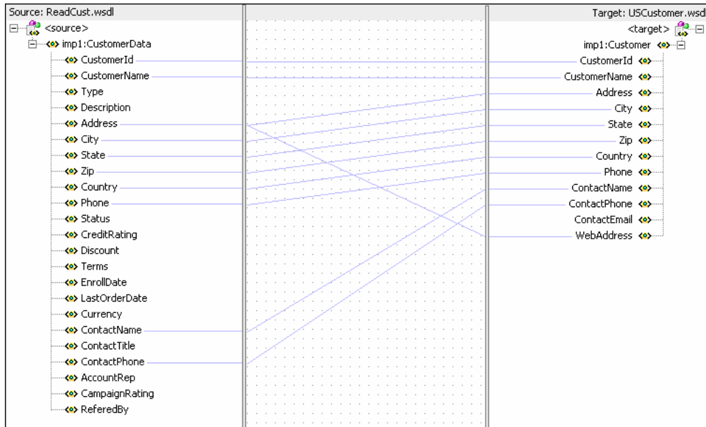
Figure 20–47 CustomerData_To_Customer.xsl Tab – Auto Mapped Connections
