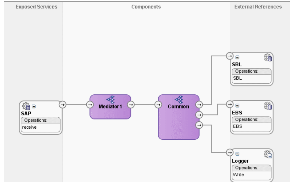
Figure 47-14 XrefCustApp Use Case in SOA Composite Editor
