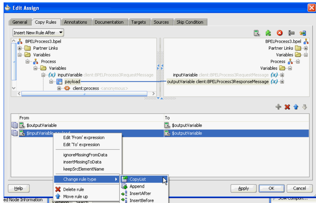
Figure A-5 Copy Rule Converted to bpelex Extension in BPEL 2.0
