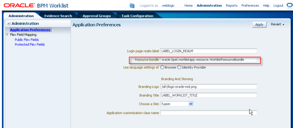
Figure 30–44 Specifying the Resource Bundle
