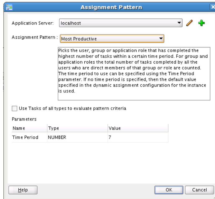
Figure 28–30 Selecting and Configuring an Assignment Pattern
