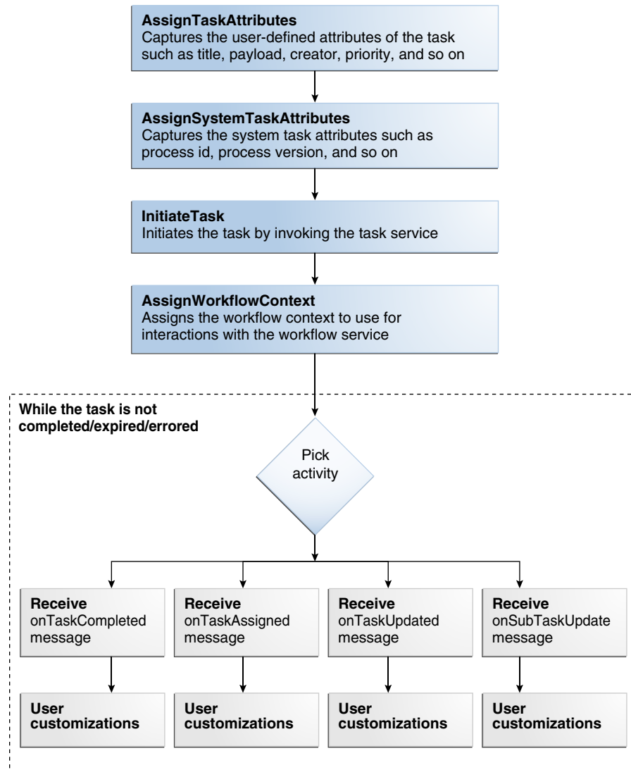
Figure 28–83 Workflow Interaction Modeling (with Callbacks)
