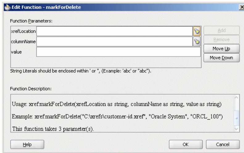
Figure 47–12 Edit Function – markForDelete Dialog
