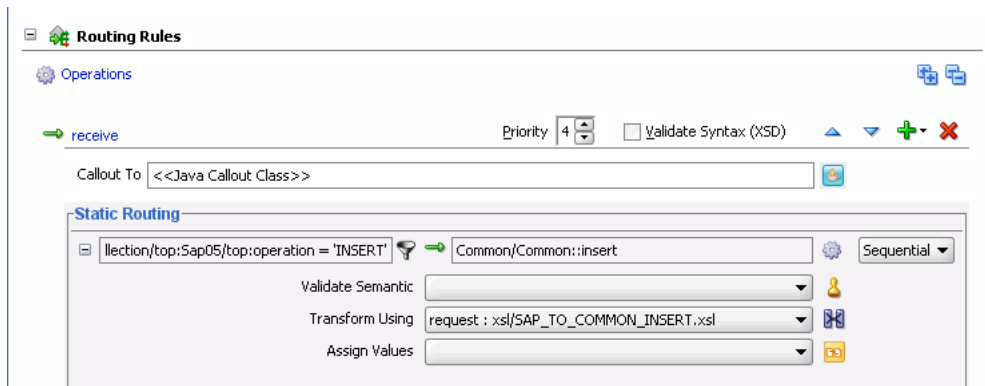
Figure 47–56 Routing Rules Section with Insert Operation
