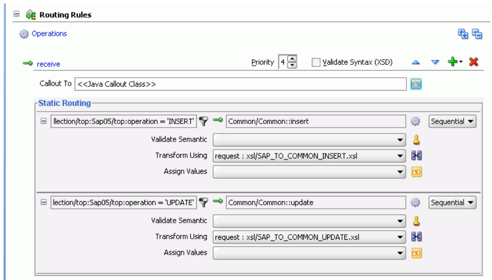
Figure 47–58 Insert Operation and Update Operation
