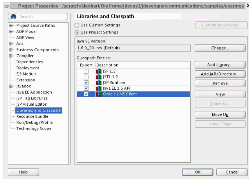
Figure 61–2 Verifying Libraries
