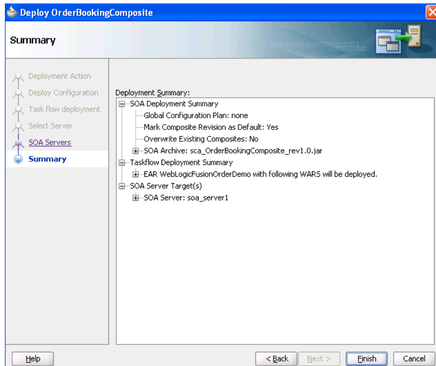
Figure 41–12 Summary Page
