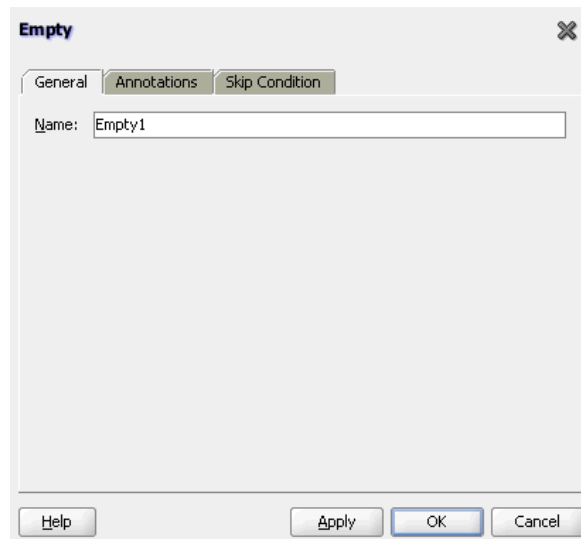
Figure 12–12 Empty Activity
