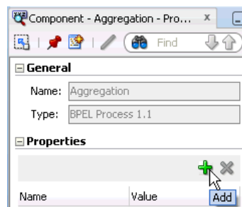
Figure 9–3 Property Inspector
