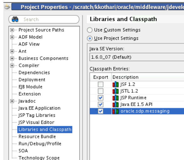
Figure 61–8 Verifying Libraries
