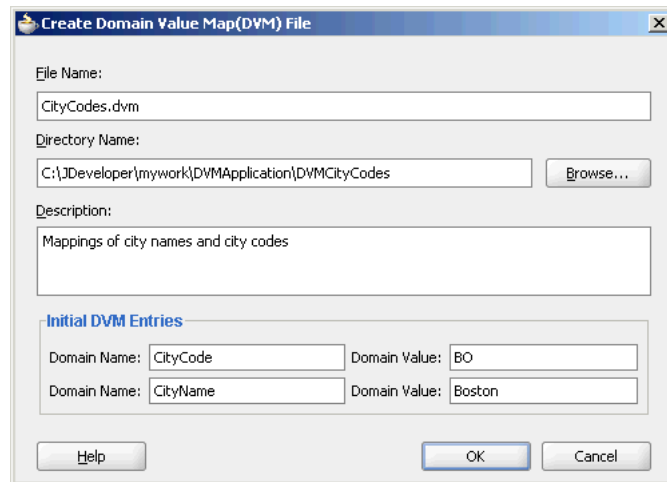
Figure 45-2 Populated Create Domain Value Map File Dialog
