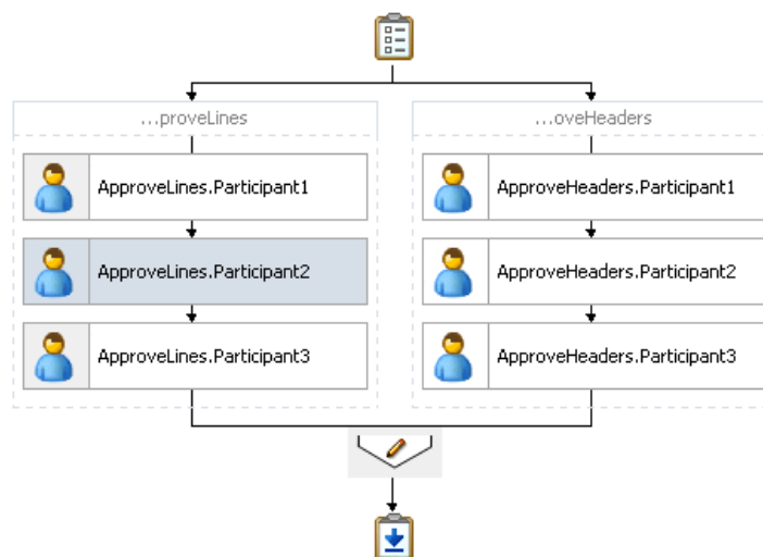
Figure 28–48 Early Completion of Parallel Subtasks
