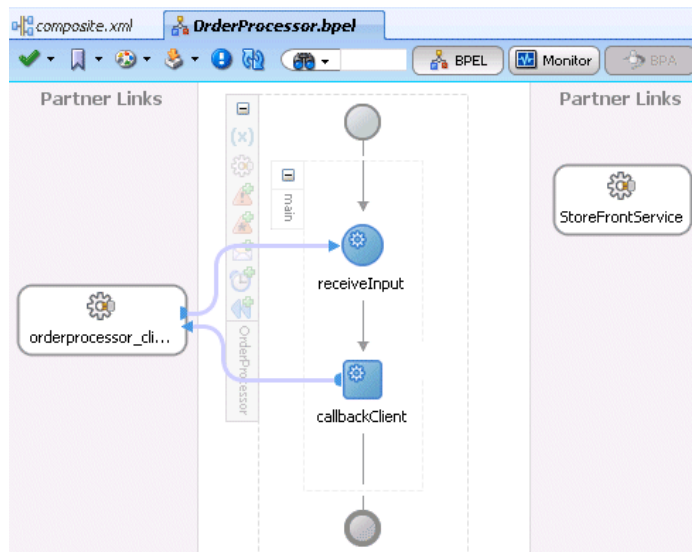
Figure 2–21 Display of the Reference as a Partner Link in the BPEL Process
