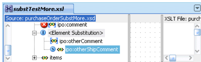
Figure 38–45 If the Element is in the Source Tree and Element Substitution is Selected
