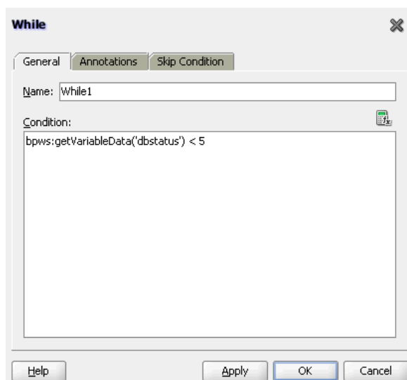
Figure A–48 While Dialog
