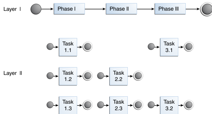
Figure 49–1 Two-Layer BPM
