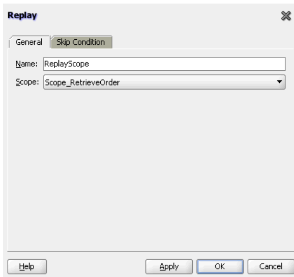
Figure 12-13 Replay Dialog
