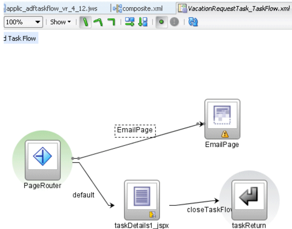
Figure 29–36 Completed Control Flow for an Email Notification
