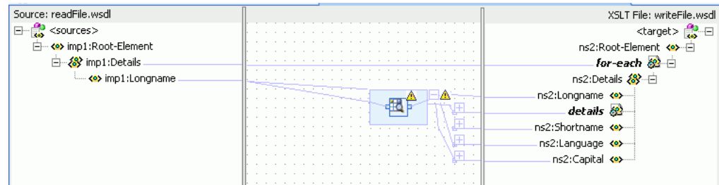
Figure 45–23 Adding lookupValue Function to imp1:Root-Element to ns2:Root-Element
