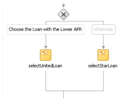
Figure 11-5 Switch Activity Design
