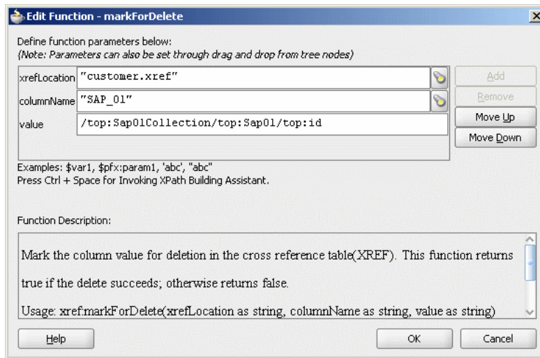
Figure 47–32 Edit Function – markForDelete Dialog: XrefCustApp Use Case
