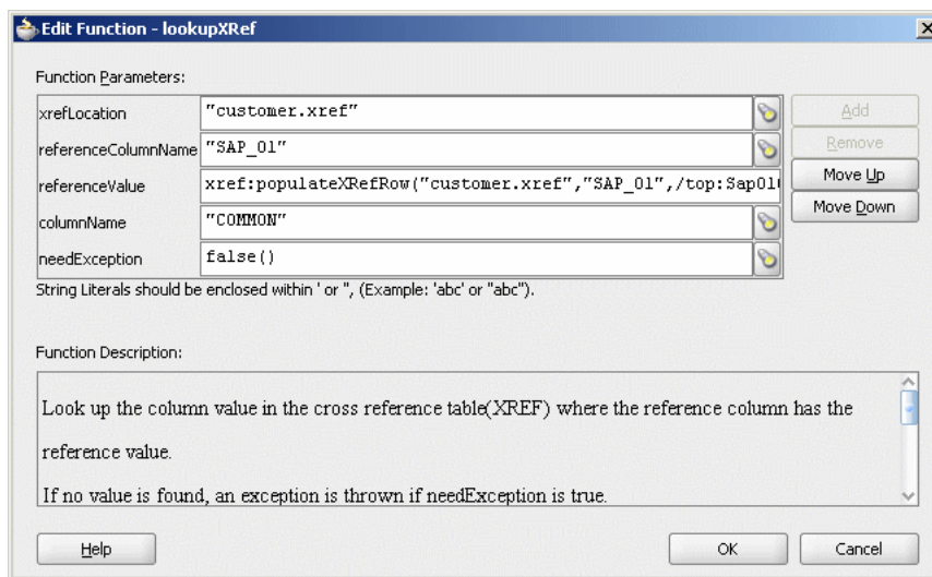
Figure 47–11 Populated Edit Function – lookupXRef Dialog
