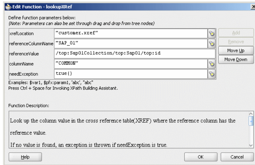
Figure 47-27 Edit Function – lookupXRef Dialog: XrefCustApp Use Case
