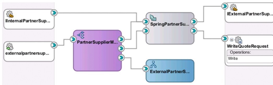
Figure 50–22 Partner Supplier Composite with Spring Service Component
