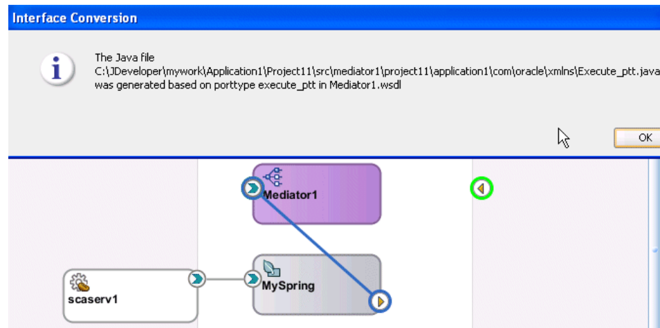
Figure 50–18 Java File Creation from the Oracle Mediator WSDL File
