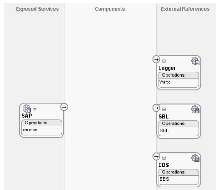
Figure 47–22 Logger Reference in SOA Composite Editor
