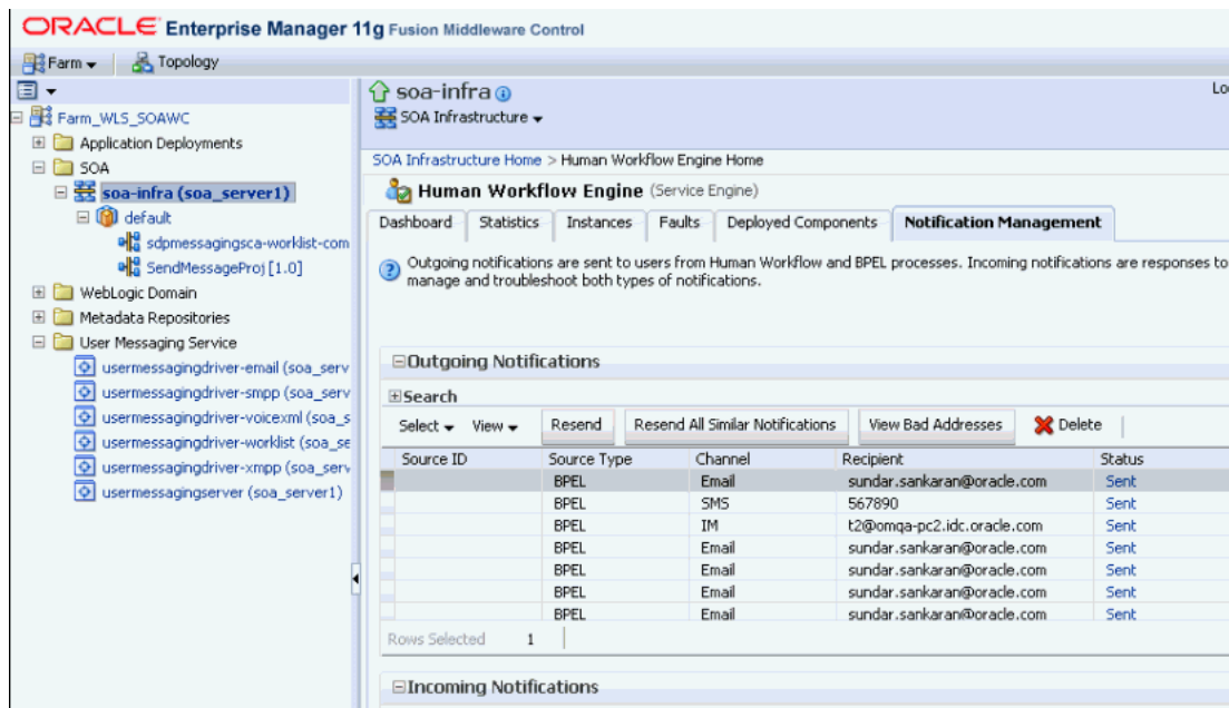
Figure J–19 Viewing Outgoing Notifications
