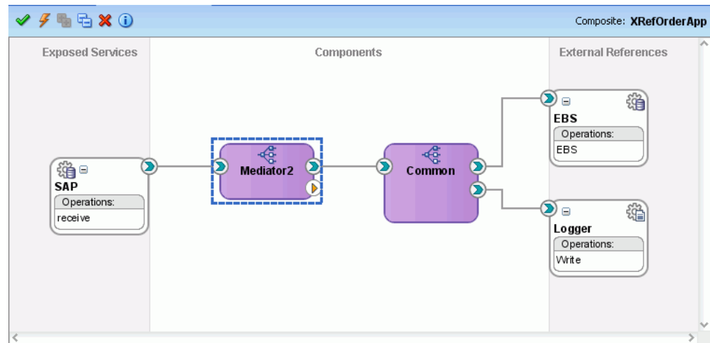
Figure 47-46 XrefOrderApp Use Case in SOA Composite Editor
