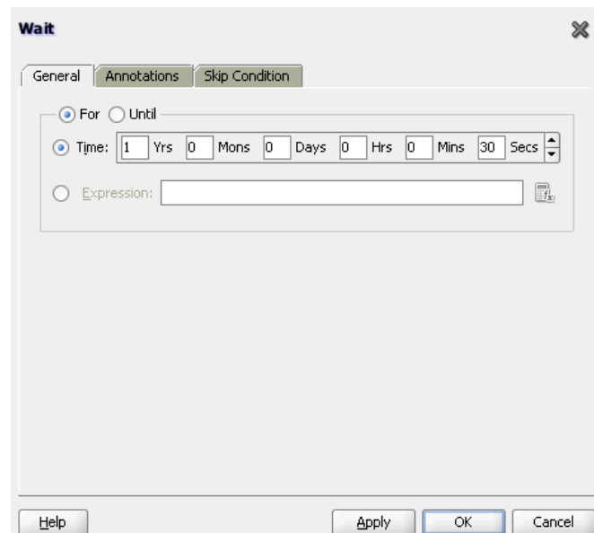
Figure 15-7 Wait Dialog
