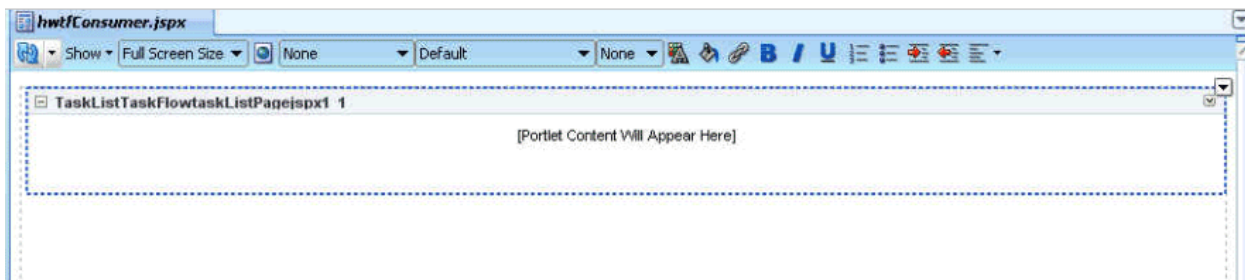
Figure 34–12 consumer.jspx
