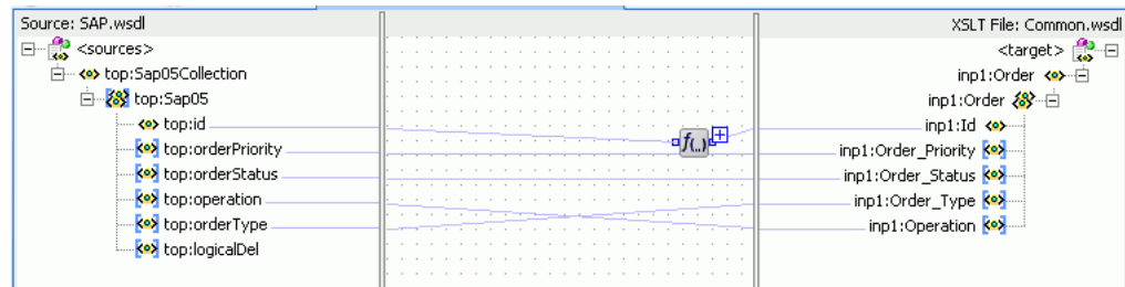
Figure 47-54 SAP_TO_COMMON_INSERT.xsl Transformation
