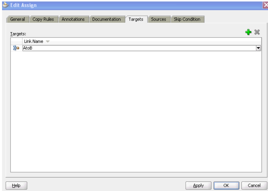
Figure 10-7 Target Activity
