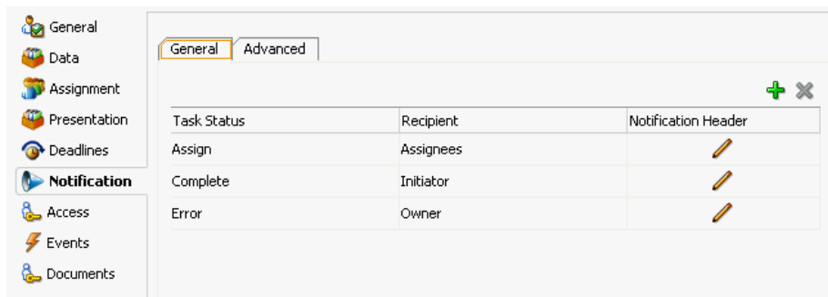
Figure 28–64 Human Task Editor — General Tab of Notification Section
