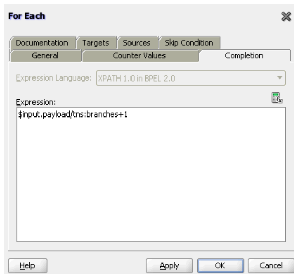
Figure 10–15 Completion Tab of the forEach Activity
