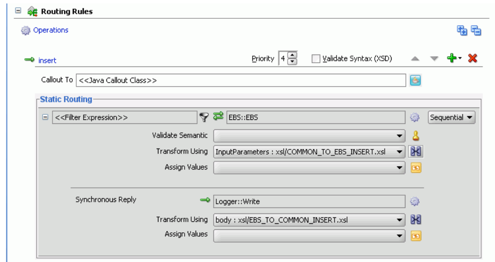
Figure 47–61 Insert Operation with EBS Target Service
