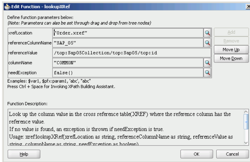
Figure 47–57 Edit Function – lookupXRef Dialog: XRefOrderApp Use Case
