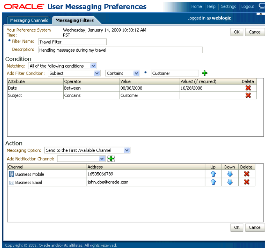
Figure 65–9 Creating a Filter
