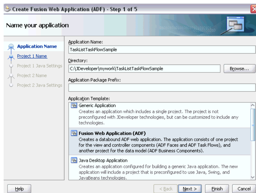
Figure 30–68 Creation of Application with an Embedded Reusable Worklist Region
