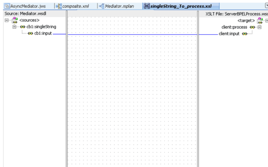
Figure 20–51 singleString_To_process.xsl Window
