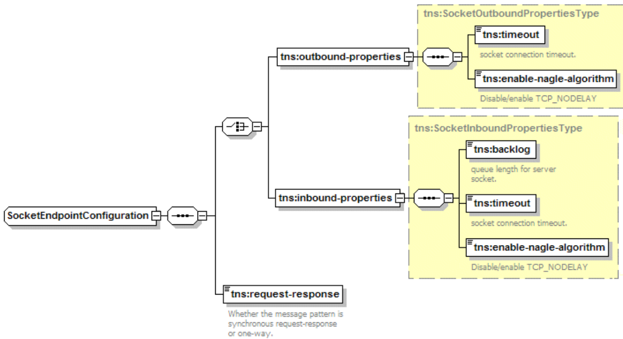
Figure 42–2 SocketEndpointConfiguration Properties
