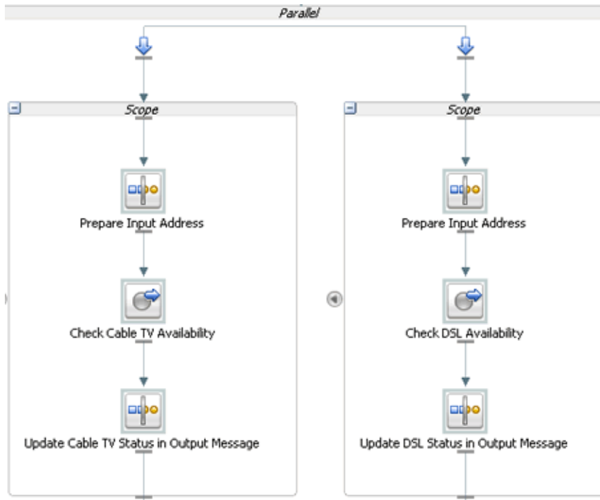
Figure 2–2 Parallel Node
