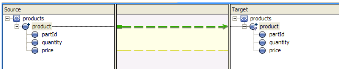
Figure 6–5 Repeating-Group-to-Repeating-Group Link
