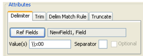
Figure 19–2 Reference Field
