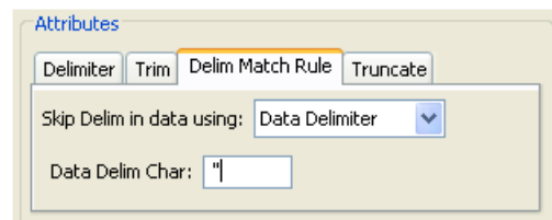
Figure 19–3 Data Delimiter
