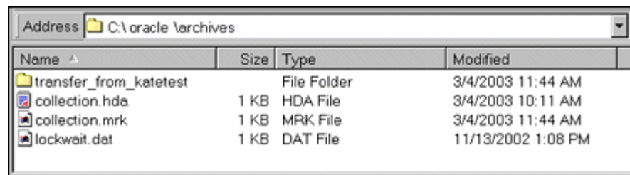
Figure 8–8 Collection Structure
