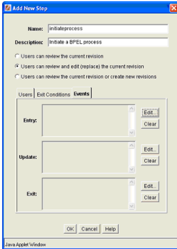
Figure C-8 Add New Step Dialog, Events Tab
