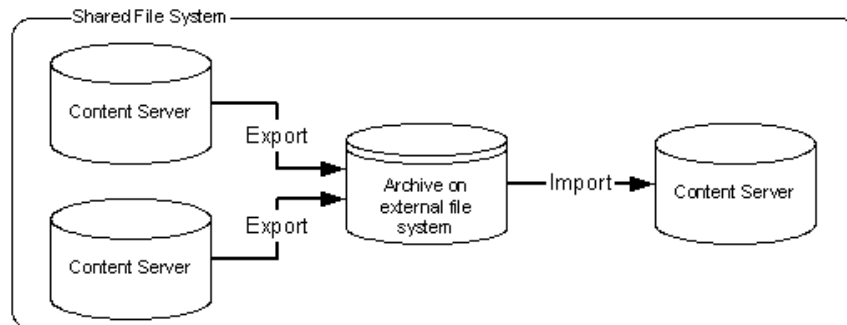
Figure 8-38 Many-to-One Archiving: On Shared External File System
