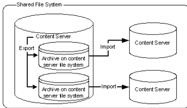
Figure 8–34 One-to-Many Archiving: Export to Collection and Import from Collection on Shared File System
