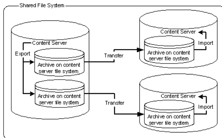
Figure 8–32 One-to-Many Archiving: On Shared File System
