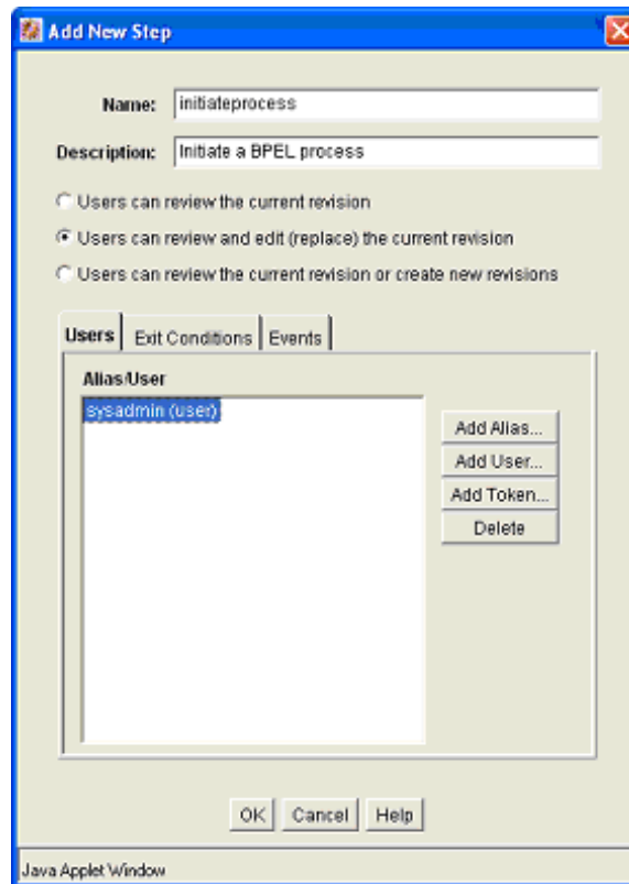
Figure C-5 Add New Step Dialog
