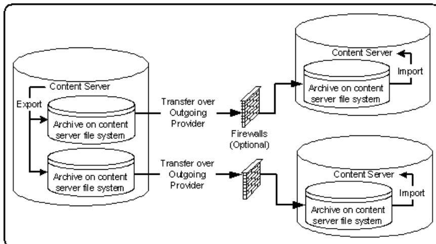
Figure 8–31 One-to-Many Archiving: Over Sockets
