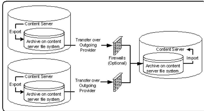
Figure 8-36 Many-to-One Archiving: Over Sockets
