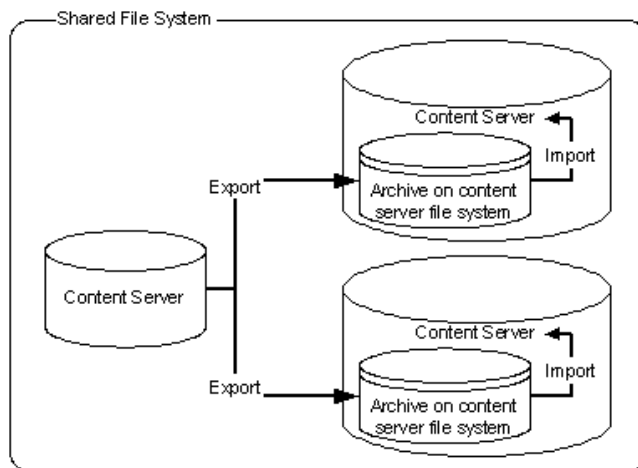
Figure 8–35 One-to-Many Archiving: Export from Source to Collections and Import from Collections on Shared File System
