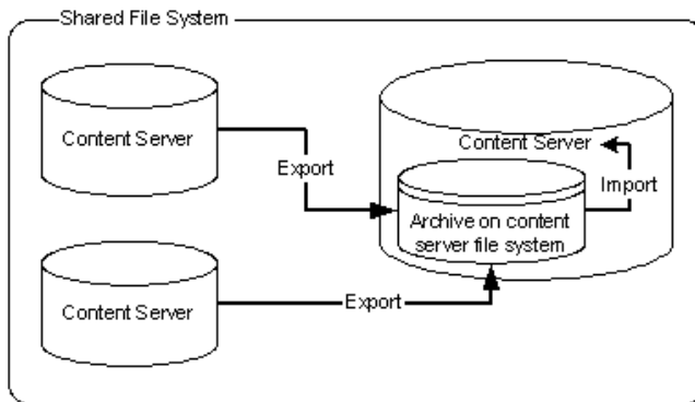
Figure 8–40 Many-to-One Archiving: Export From Sources to Collection and Import from Collection on Shared File System
