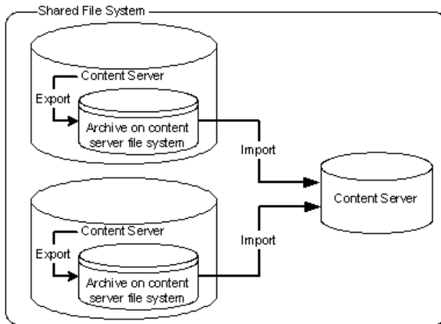
Figure 8–39 Many-to-One Archiving: Export to Collections and Import from Collections on Shared File System
