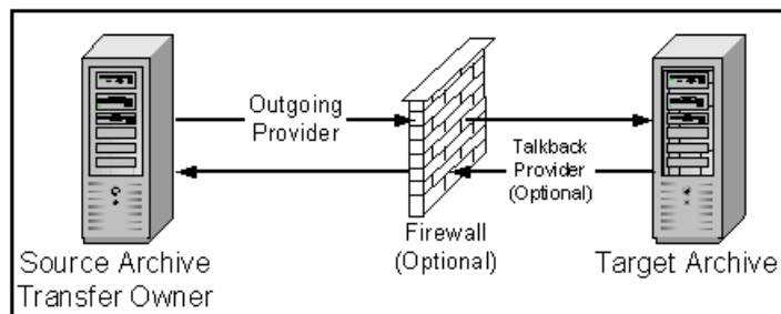
Figure 8–18 Push Transfer
