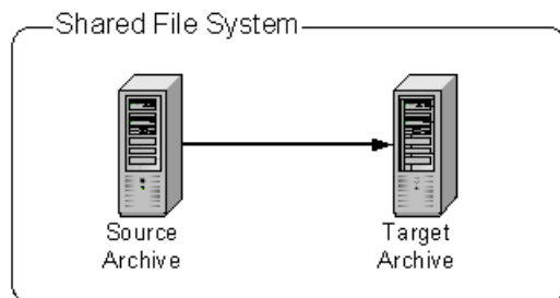
Figure 8–16 Local Transfer
