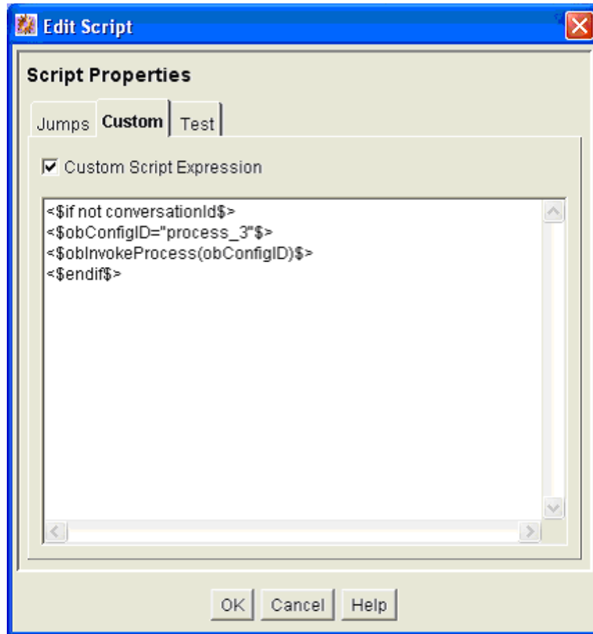
Figure C-9 Edit Script Dialog
