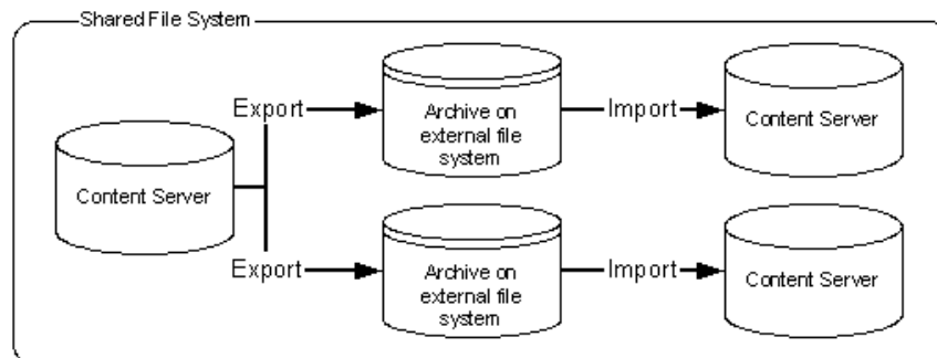
Figure 8–33 One-to-Many Archiving: On Shared External File System
