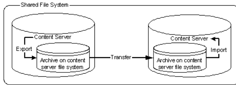
Figure 8–27 One-to-One Archiving: On Shared File System
