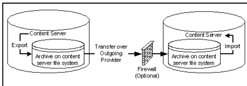
Figure 8-26 One-to-One Archiving: Over Sockets
