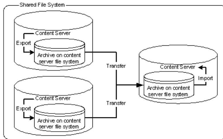
Figure 8-37 Many-to-One Archiving: On Shared File System
