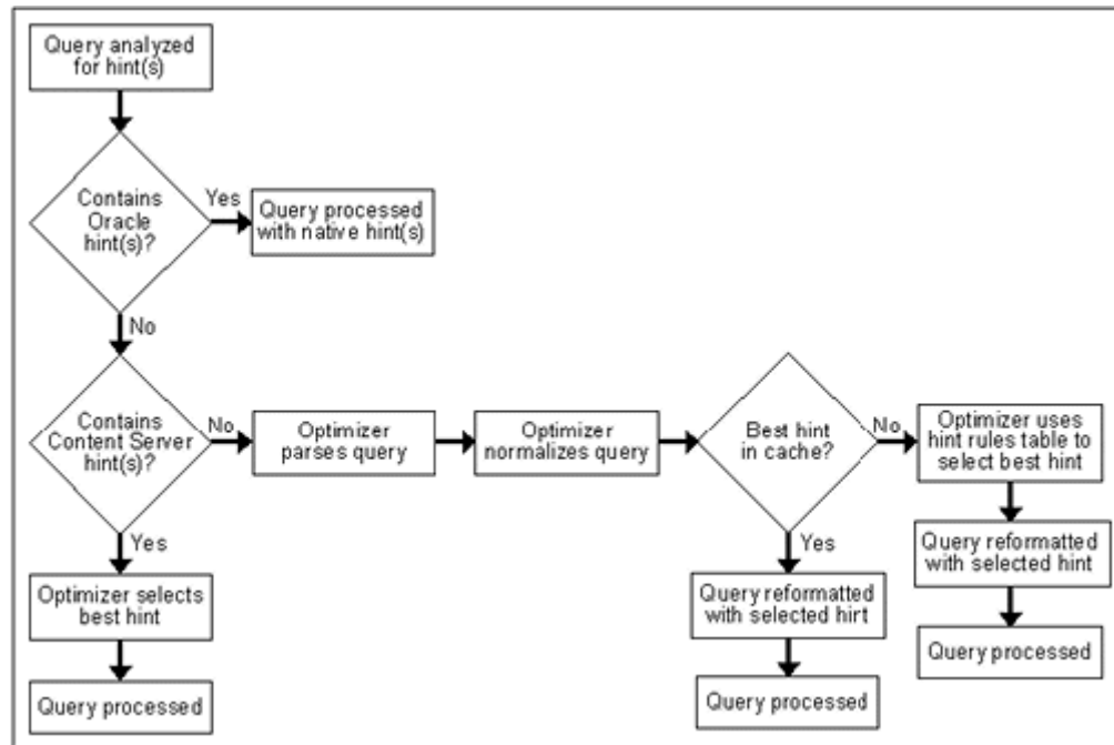
Figure 4–2 Optimization Process Sequence
