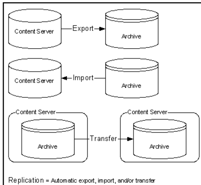
Figure 8–1 Archiver Functions
