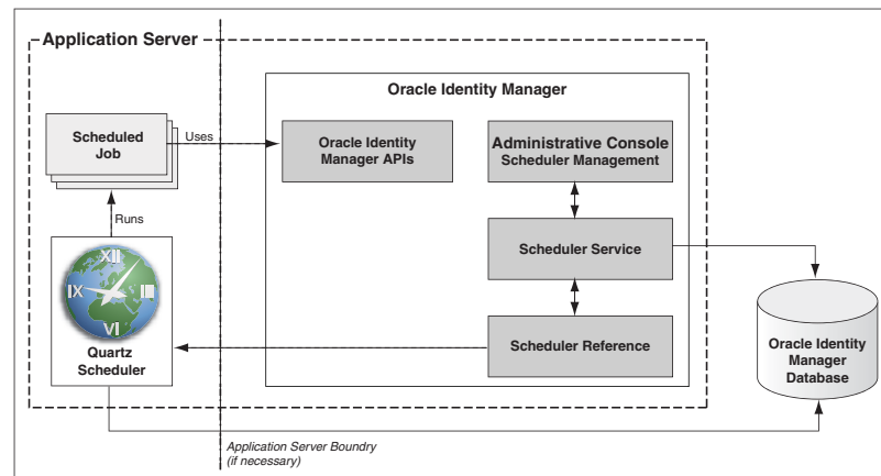
Figure 2-5 Oracle Identity Manager Scheduler Architecture
