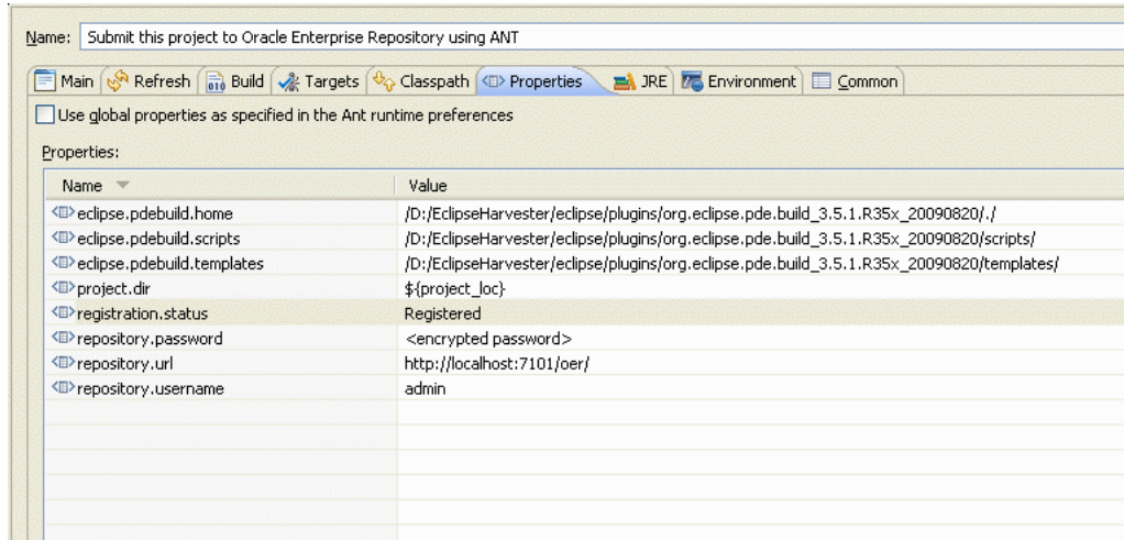
Figure 9-9 External Tools Dialog - Properties Tab
