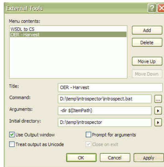
Figure 9–14 External Tools Dialog
