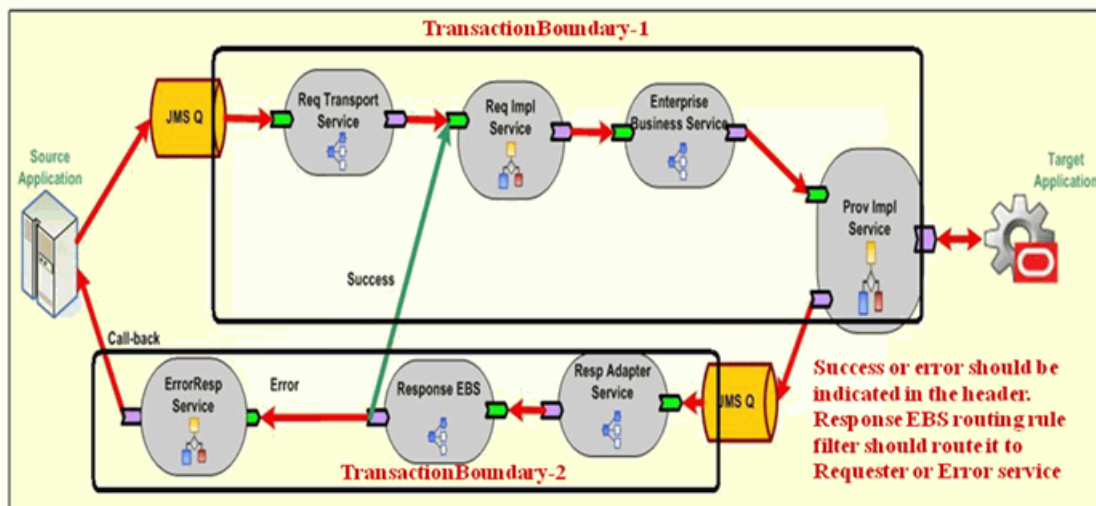
Figure 15–8 Programming Model 1: Using a Separate Service for Error Handling
