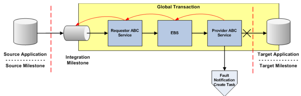
Figure 26-4 Transaction Rollback Flow
