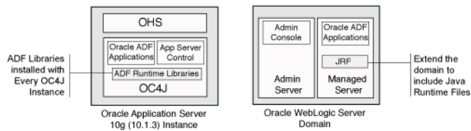
Figure 3–1 Support for Oracle ADF Applications in OC4J and Oracle WebLogic Server
