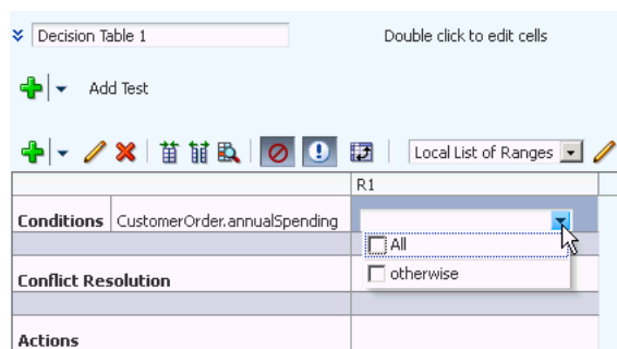
Figure 12-67 Unspecified Condition Value
