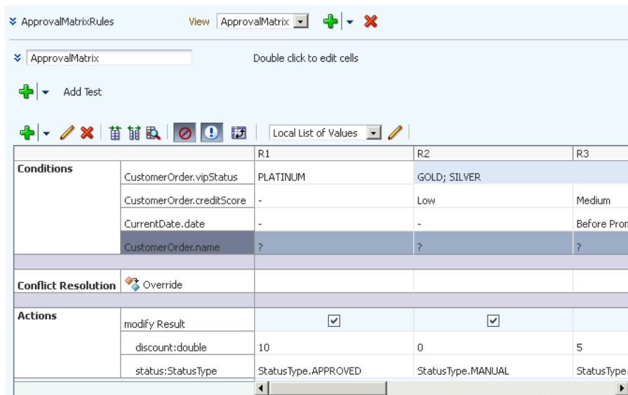
Figure 12-58 New Condition Row Added As Last Row in a Decision Table
