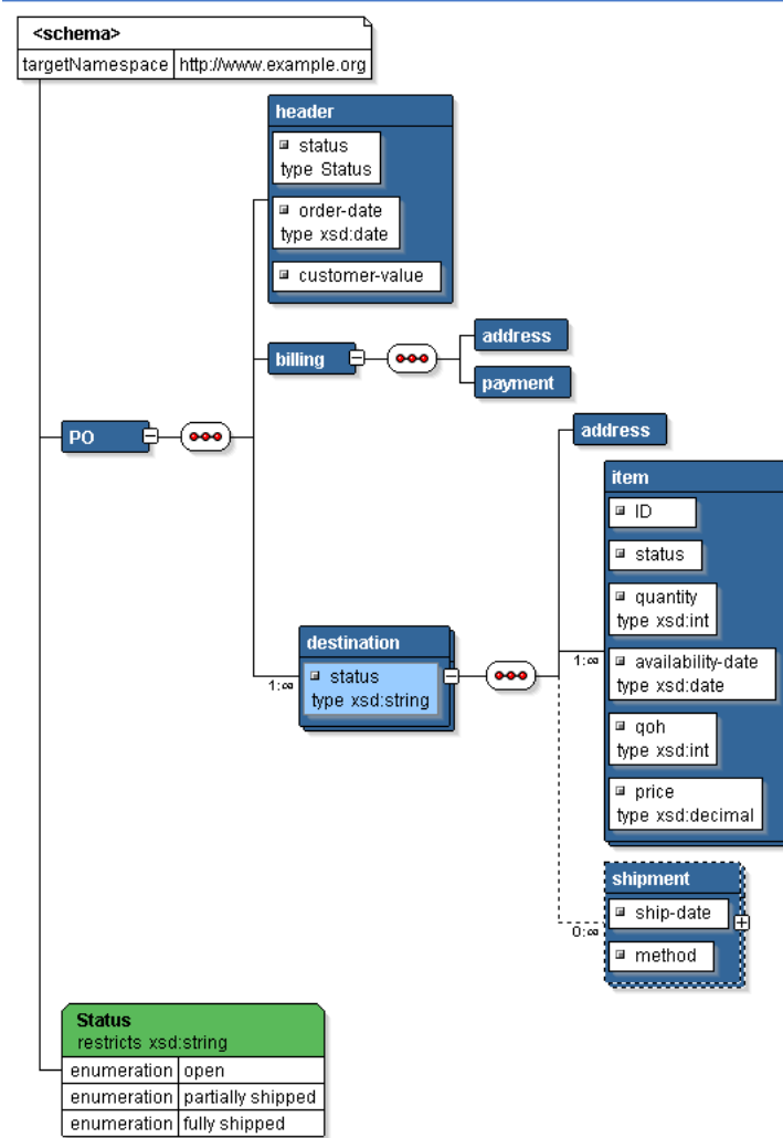
Figure 4–55 PO Schema for Tree Mode Rules Sample
