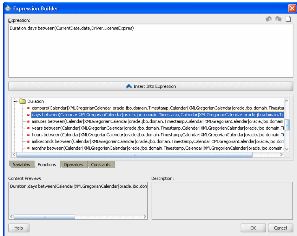
Figure 4–70 Using Duration Methods in a Rule
