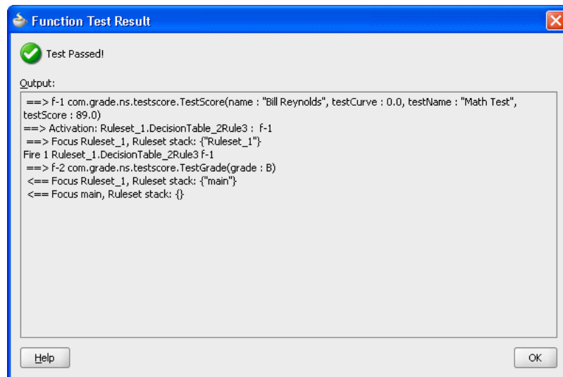
Figure 8–10 Test Passed Test Function Output
