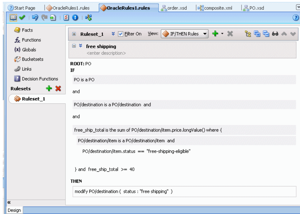
Figure 4–66 Advanced Tree Mode Free Shipping Rule
