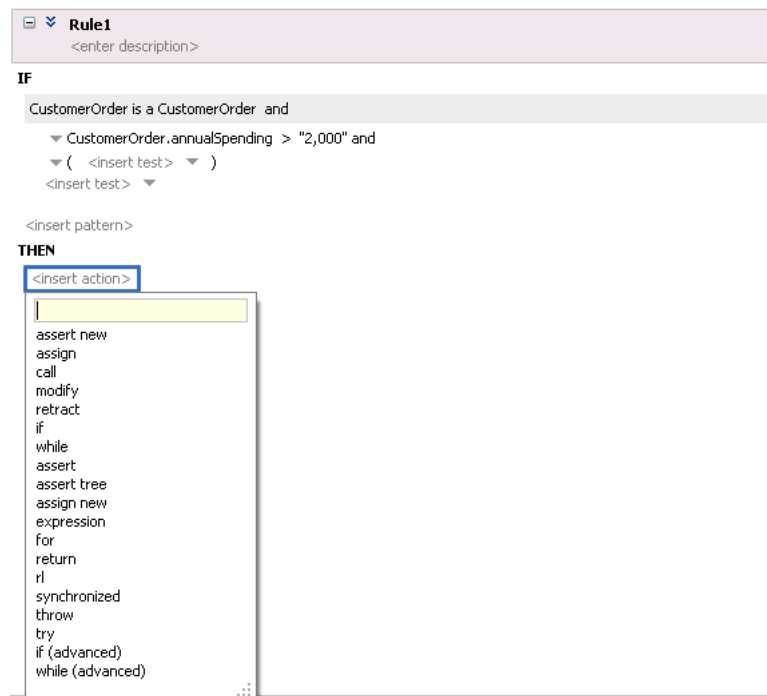
Figure 4–26 Adding a Modify Action to a Rule
