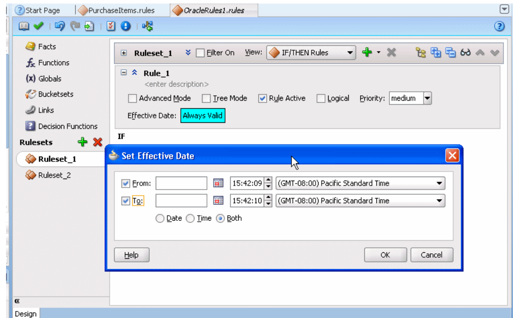
Figure 4–69 Setting the Effective Date for a Rule
