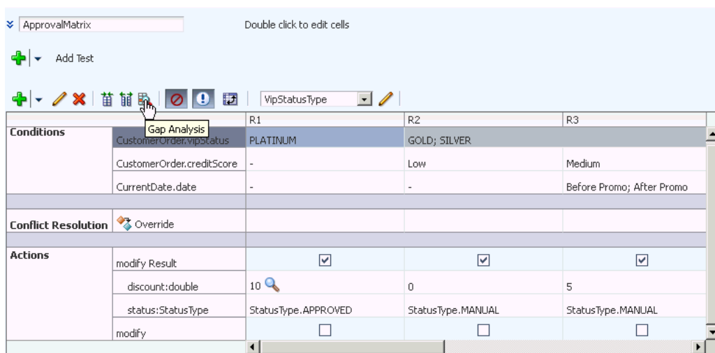
Figure 12-77 Checking for Missing Rules in a Decision Table
