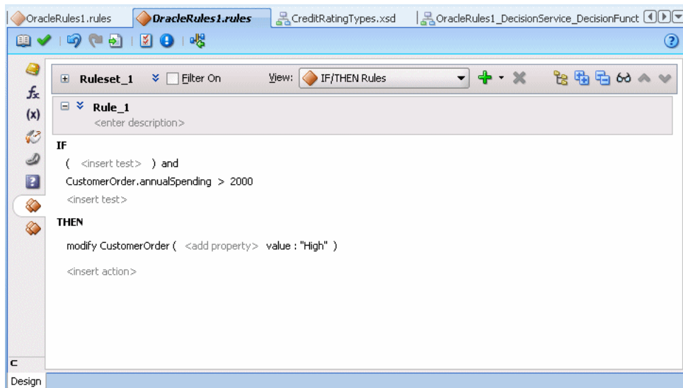
Figure 4–40 A Nested Test Added to a Rule
