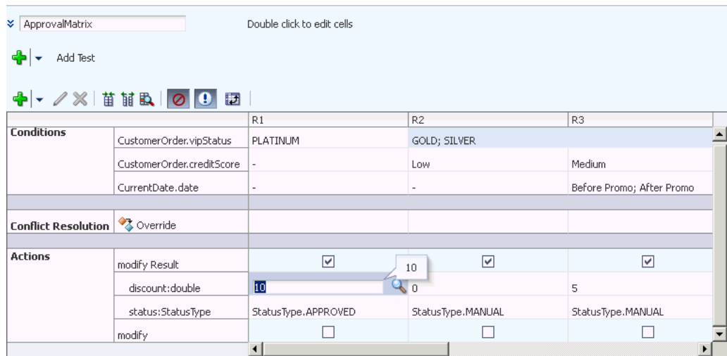
Figure 12–69 The Action Cells in a Decision Table
