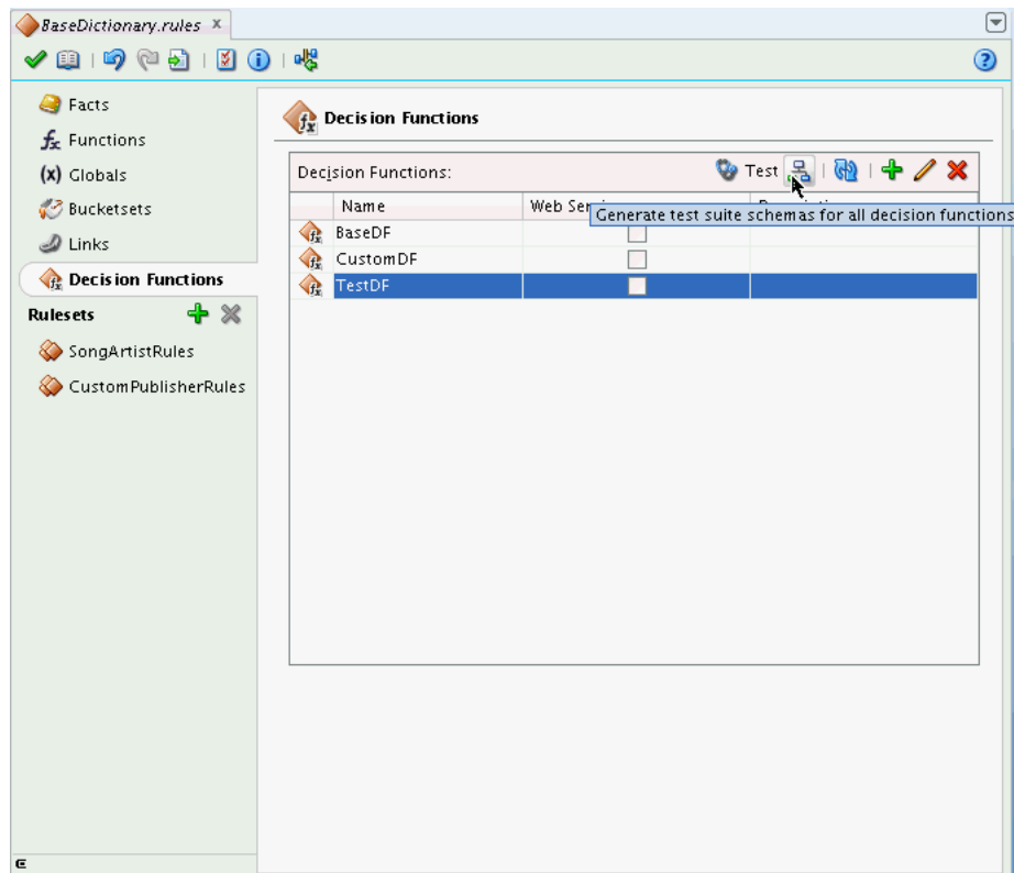
Figure 8-3 Manually Regenerating Test Suite Schemas
