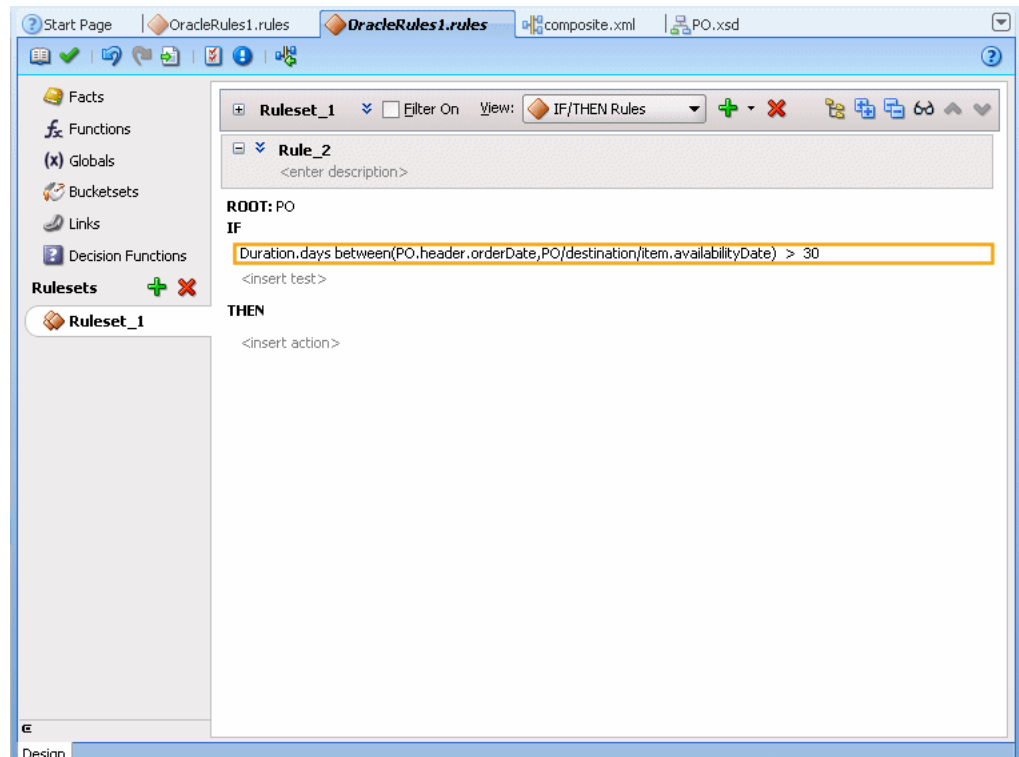
Figure 4–62 Simple Tree Mode: Right-Hand Operand with Value 30
