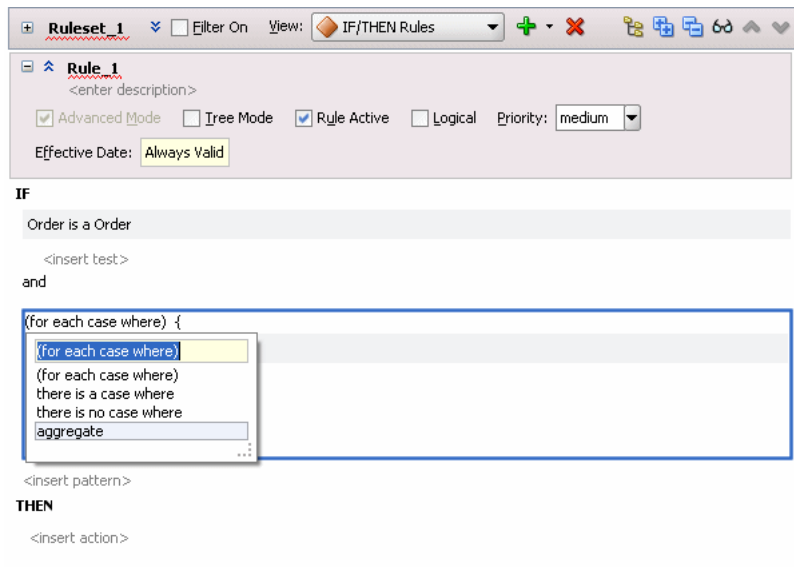
Figure 4–51 Adding an Advanced Pattern Match Option
