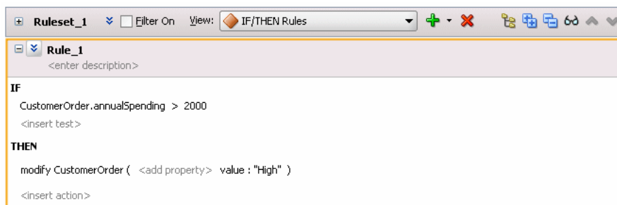
Figure 4–68 Showing Advanced Settings in a Rule
