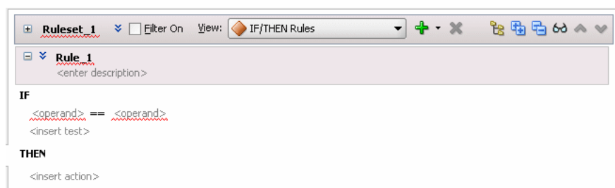
Figure 4–16 Rule Test with Left-hand-side operand and Right-hand-side operand
