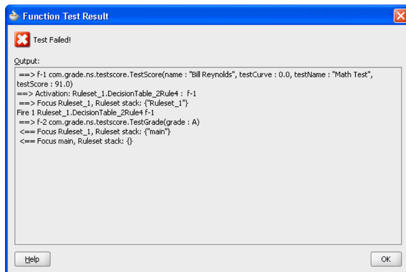
Figure 8–11 Test Failed Test Function Output
