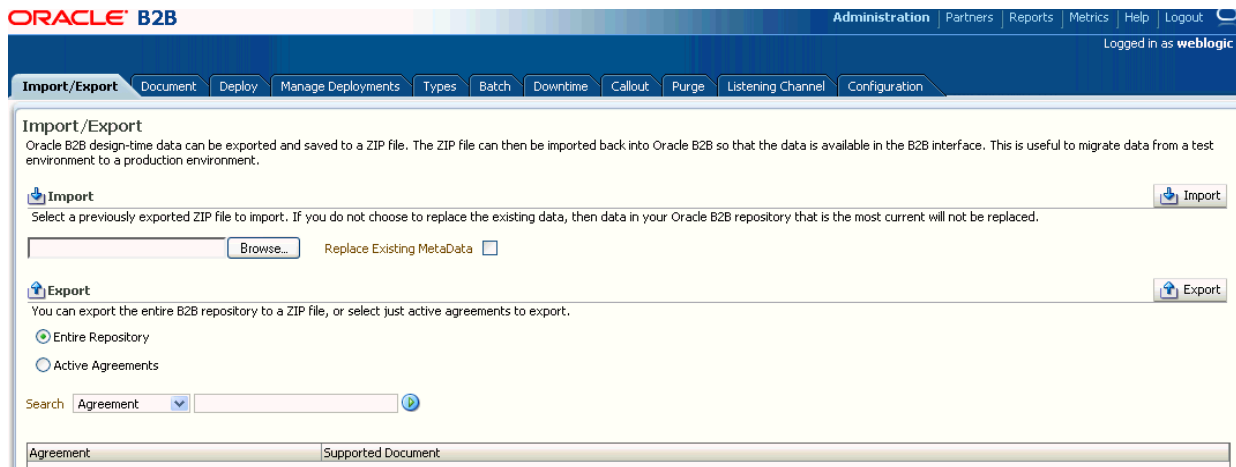
Figure 2–3 Administration Activities
