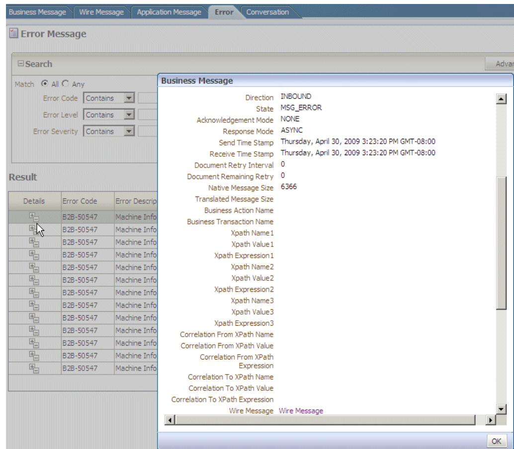
Figure 18-8 Error Reports
