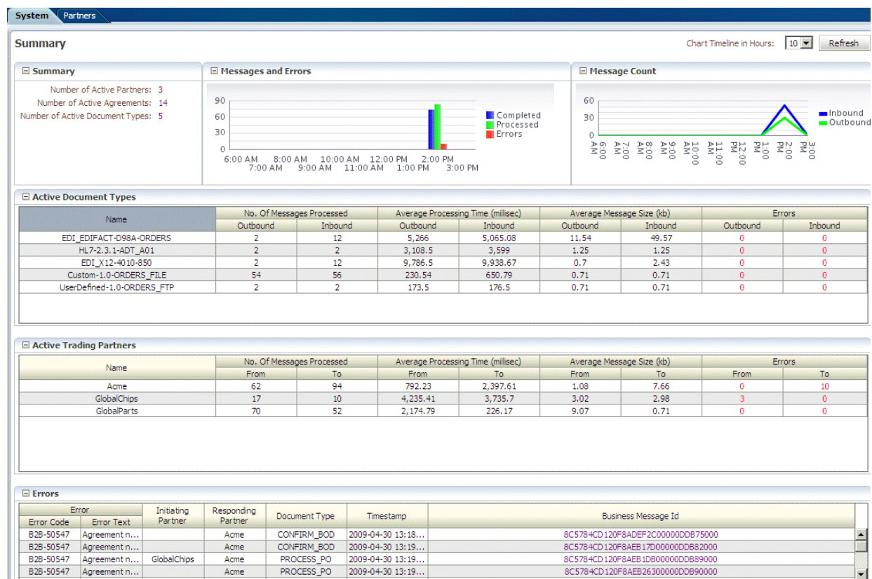
Figure 19–4 System Metrics
