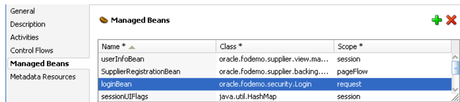
Figure 30-18 Login Bean Registered in adfc-config.xml File
