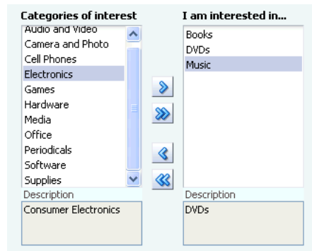
Figure 25–7 SelectManyShuttle Component
