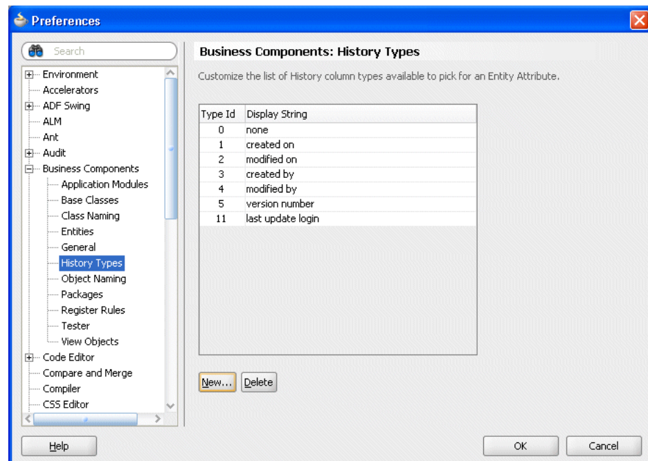
Figure 38–5 Creating New History Types
