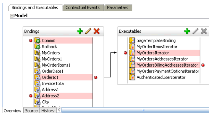
Figure 31-16 ADF Declarative Breakpoints on ADF Bindings in the Page Definition File
