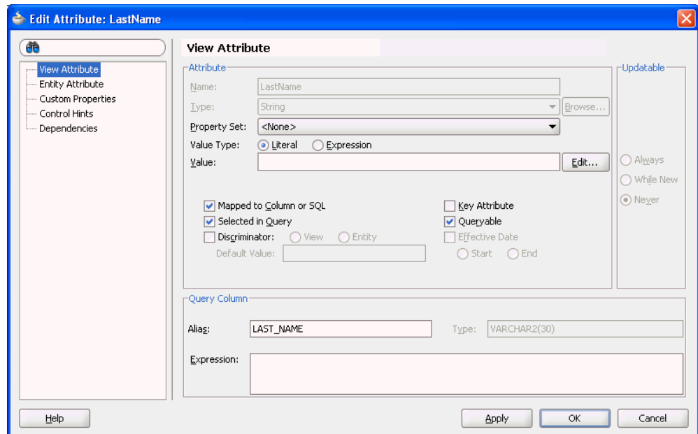
Figure 5–11 View Object Attribute Properties Inherited from Underlying Entity Object
