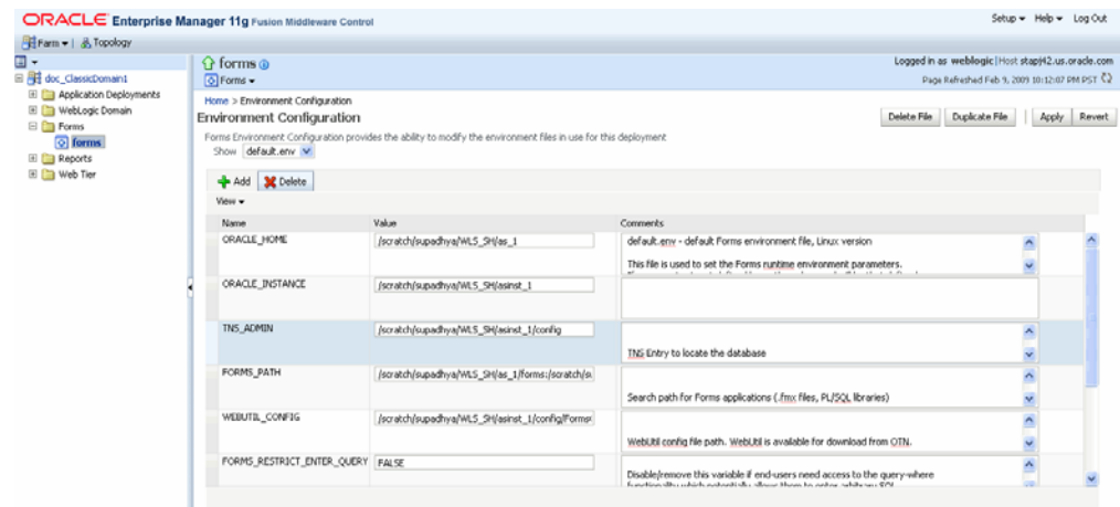
Figure 4–4 Environment Configuration page
