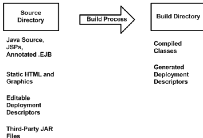
Figure 3–1 Source and Build Directories
