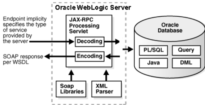
Figure 10–1 Web Service Calling in to the Database
