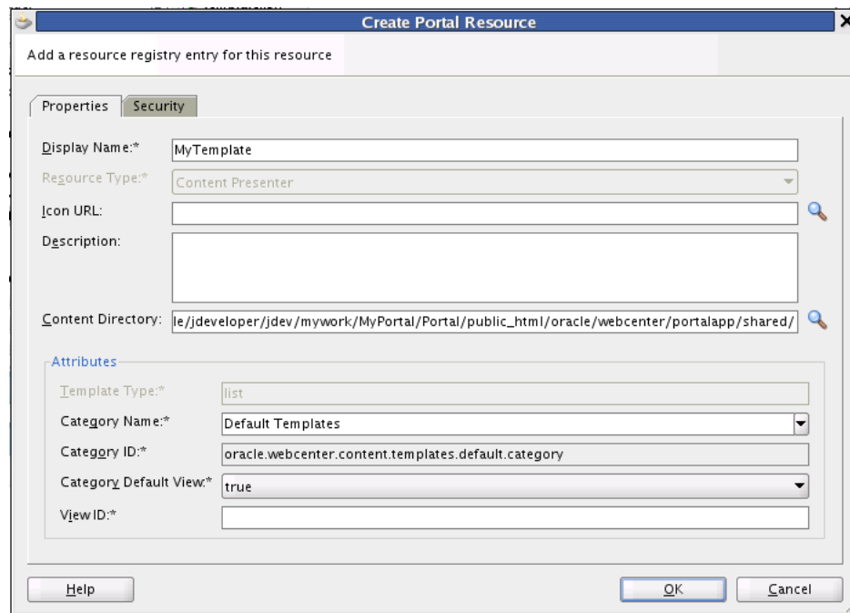
Figure 29–6 Create Portal Resource Dialog for a Multiple-Item Template
