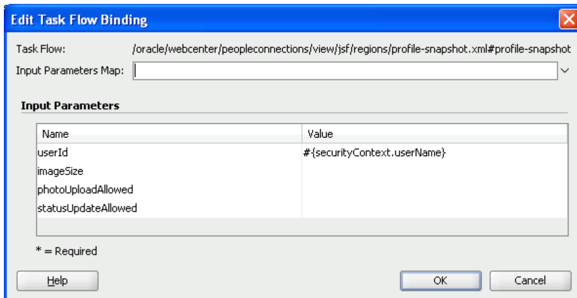
Figure 40–2 Edit Task Flow Binding Dialog
