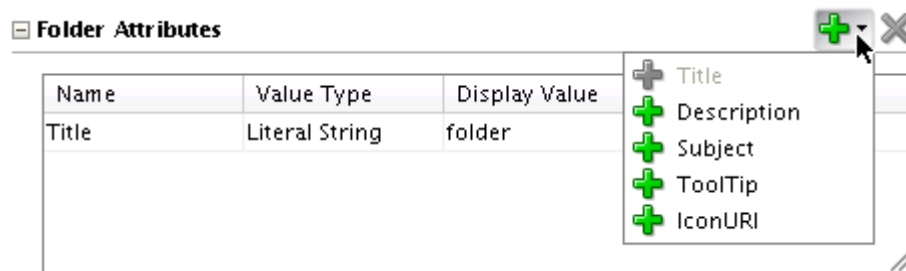
Figure 16-4 Folder Attributes
