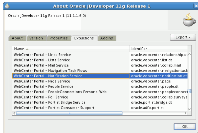
Figure 49–6 JDeveloper Extensions
