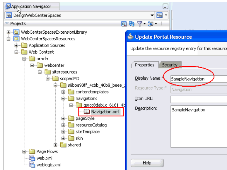
Figure 56–13 Checking Resource Display Names in JDeveloper
