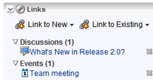
Figure 43–3 Links Dialog
