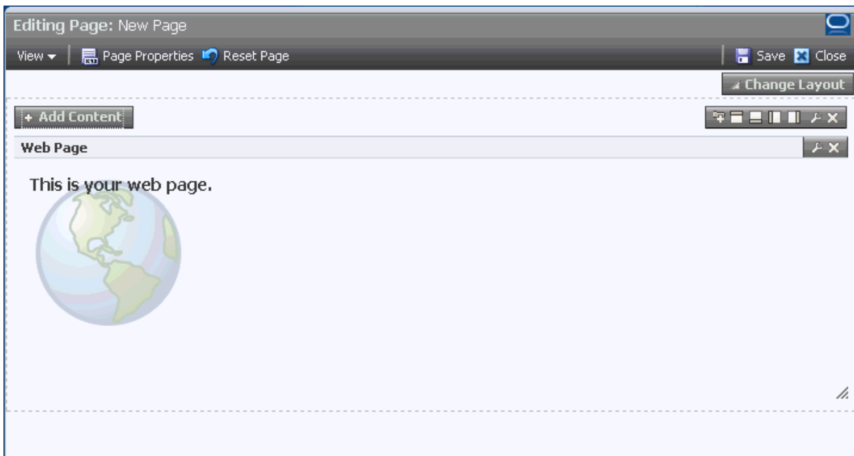
Figure 23–4 Customized Page
