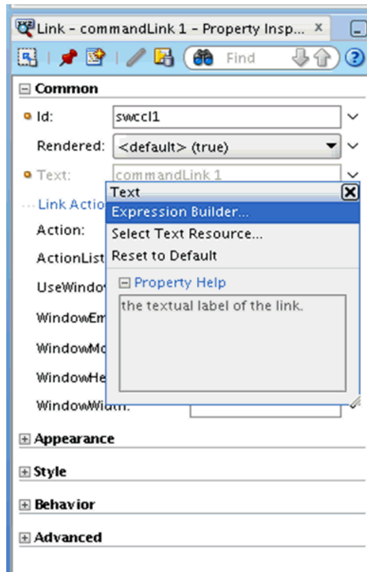
Figure 25–8 Property Inspector
