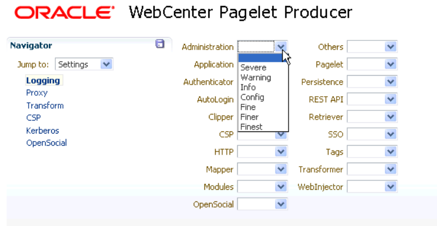
Figure 63–11 Pagelet Producer Console: Settings - Logging
