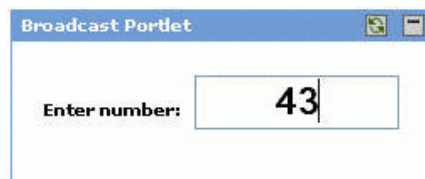
Figure 63–5 Broadcast Portlet
