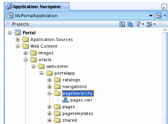
Figure 9-4 Contents of the pagehierarchy Folder
