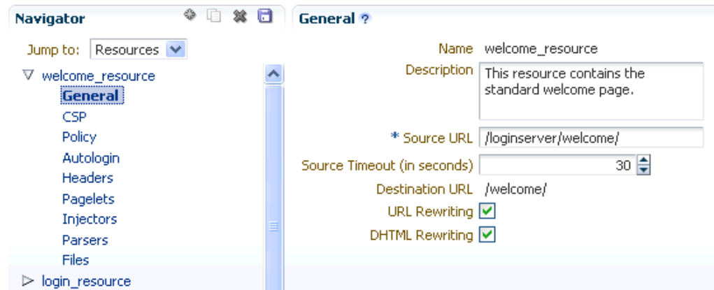
Figure 25–7 Pagelet Producer Console: Resource - General Page
