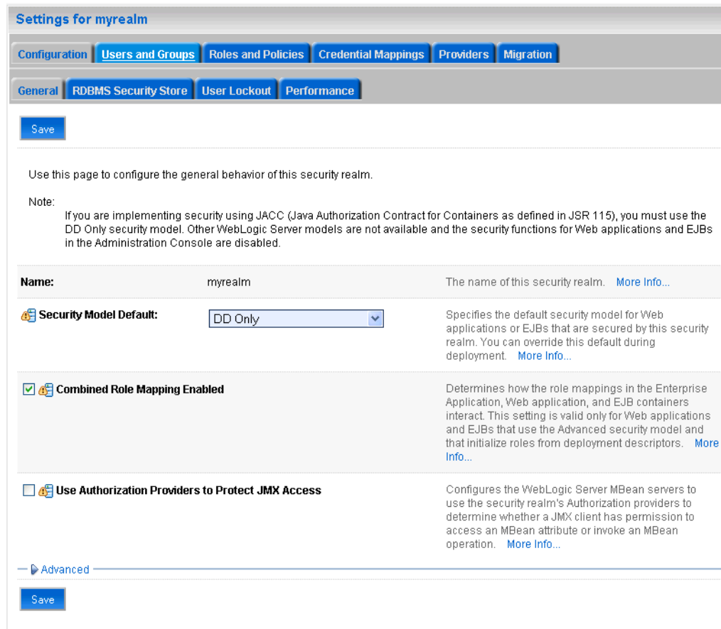
Figure 29–3 Realm Settings Pane
