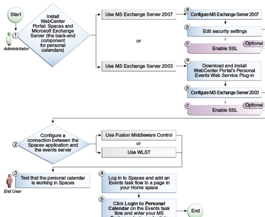
Figure 15–1 Configuring Personal Events for WebCenter Portal: Spaces
