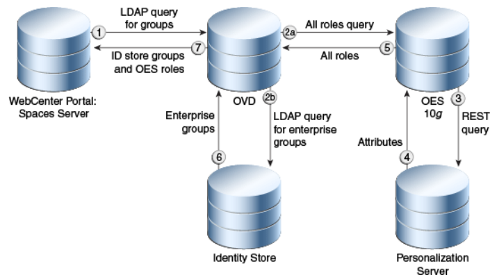
Figure 29-32 Group Query
