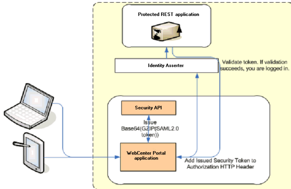
Figure 29–45 REST Identity Propagation and Assertion
