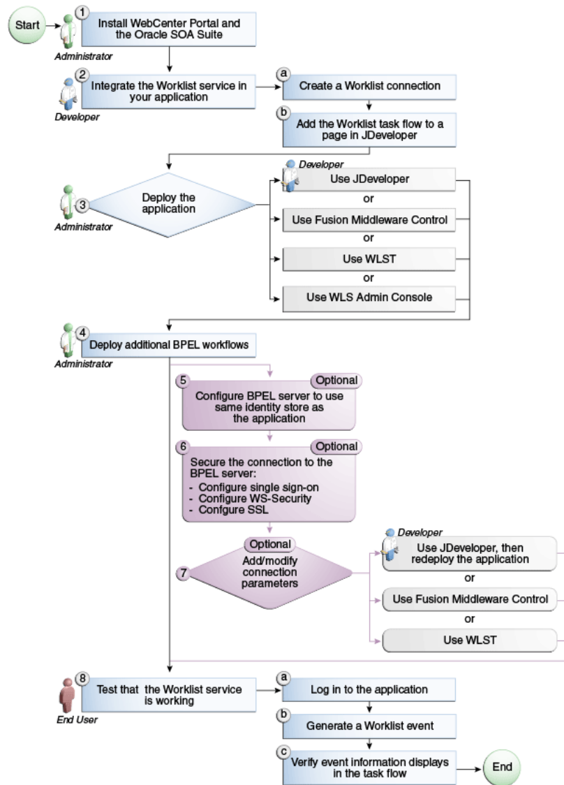
Figure 23–2 Configuring the Worklist Service for Framework applications
