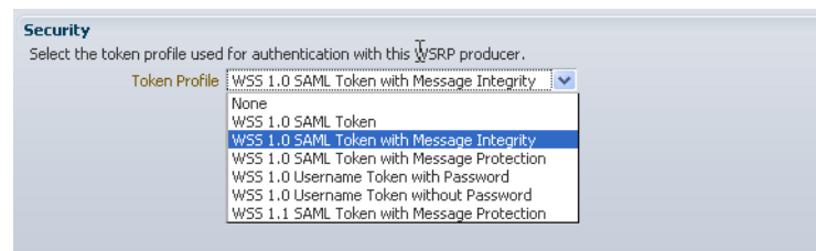
Figure 25–21 Pagelet Producer Console: Register Portlet Producer - WSRP Producer: Token Profile
