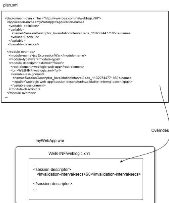
Figure 4–1 WebLogic Server Deployment Plan
