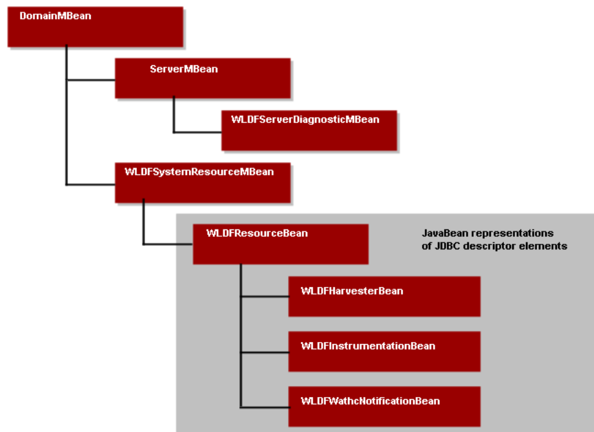
Figure 3–2 WLDF Configuration Bean Tree
