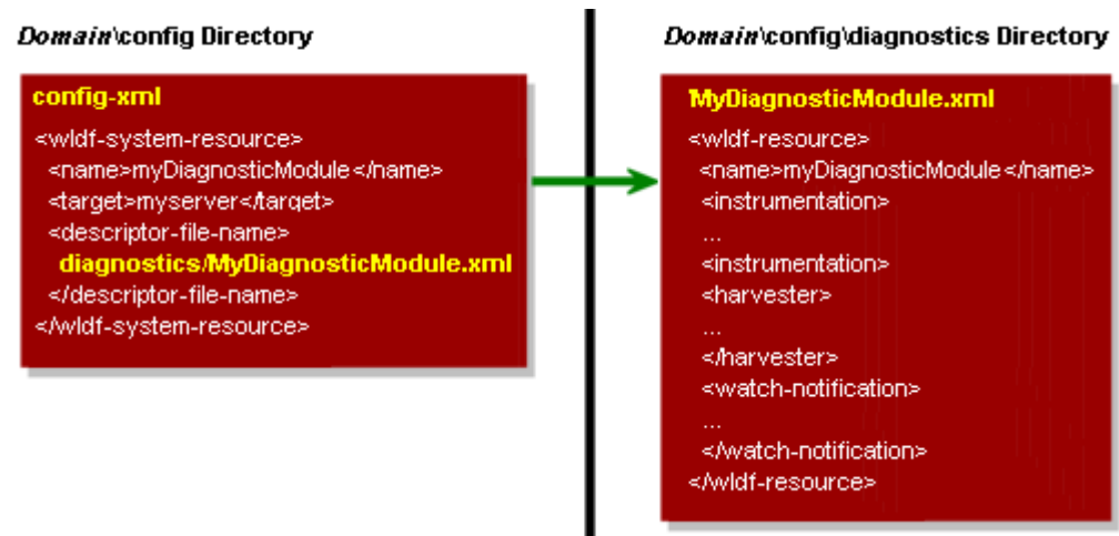
Figure 3–1 Relationship of config.xml to System Descriptor File
