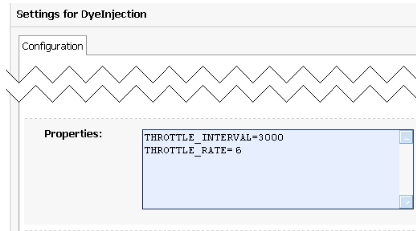
Figure 11–4 Configuring the THROTTLE Dye
