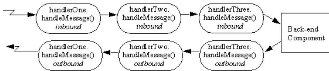
Figure 8–1 Order of Execution of Handler Methods
