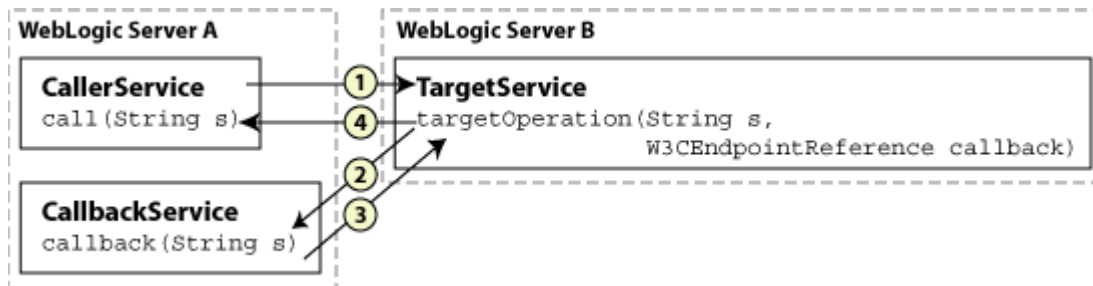
Figure 4–1 Example Callback Implementation
