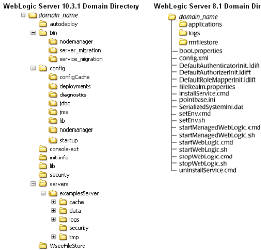
Figure C-1 WebLogic Server 10.3.1 and WebLogic Server 8.1 Directory Structures
