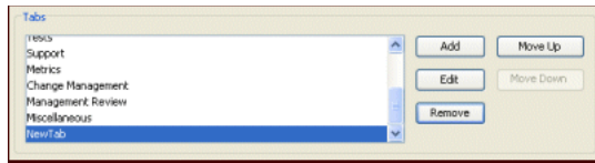
Figure 3–14 Tabs List
