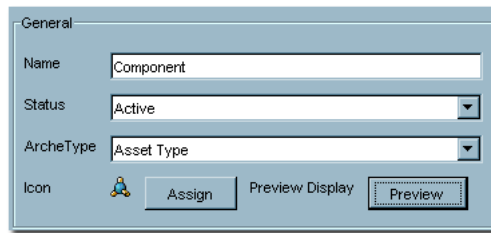
Figure 3–21 General Section
