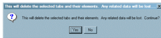
Figure 3–17 Confirmation Dialog
