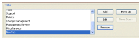
Figure 3–16 Tabs List
