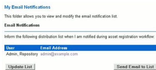
Figure 1-48 Email Notifications
