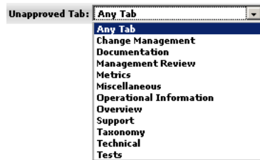
Figure 1–46 tab_type.gif
