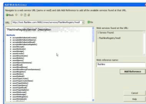
Figure 9-3 Add Web Reference Dialog
