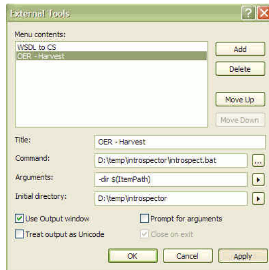
Figure 7–15 External Tools Dialog
