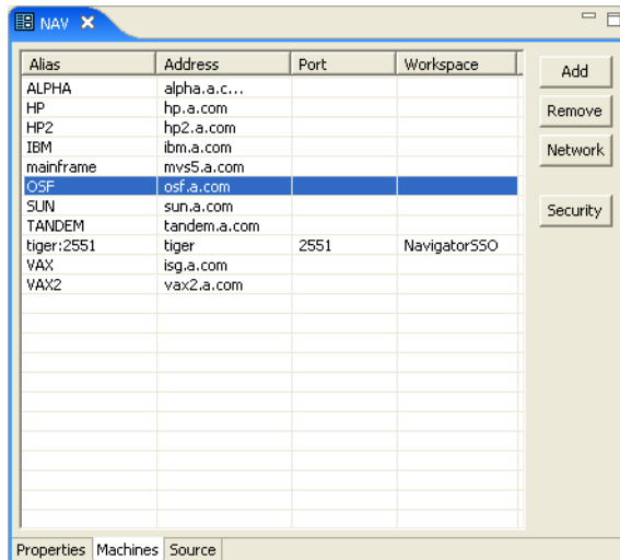
Figure 8–3 The Binding Editor Machines tab
