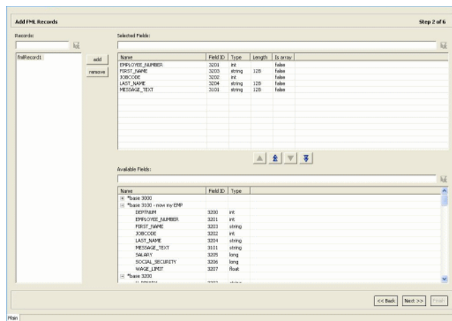
Figure 2–29 Get Tuxedo Records Step
