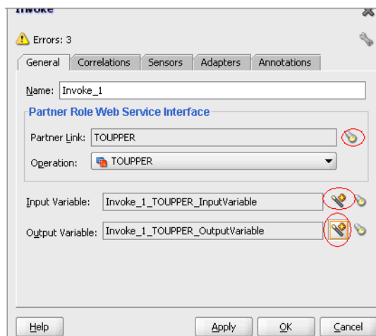
Figure 6–25 Invoke Dialog Box
