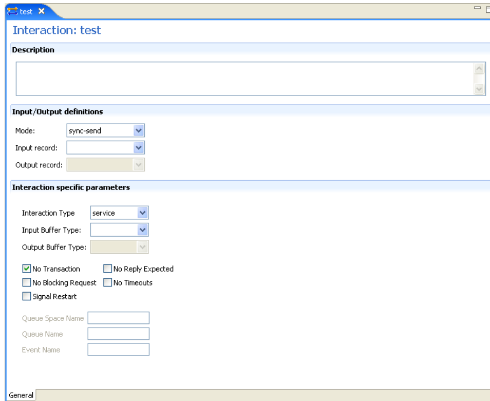
Figure A–2 Adapter Metadata Interactions for Tuxedo and Tuxedo Queue
