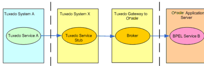
Figure 1–2 Tuxedo Gateway Adapter Flow
