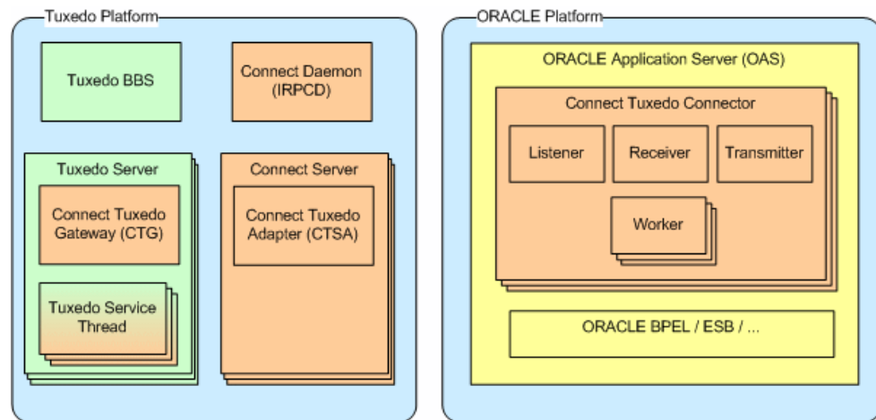
Figure 1–3 Tuxedo Gateway Adapter Components
