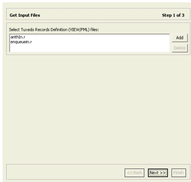
Figure 2–19 The Get Input Files screen
