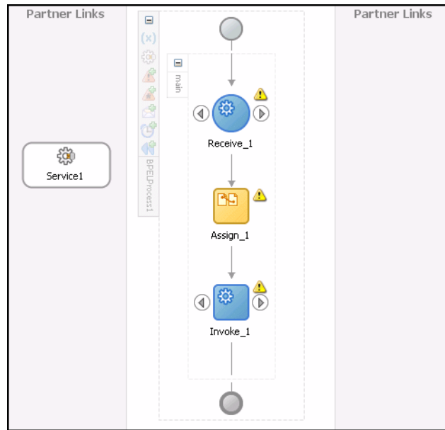
Figure 6–8 Inbound Process
