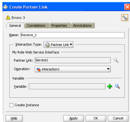
Figure 6–9 Receive Properties
