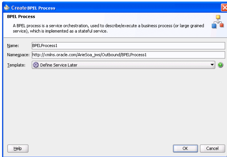
Figure 6–2 BPEL Process
