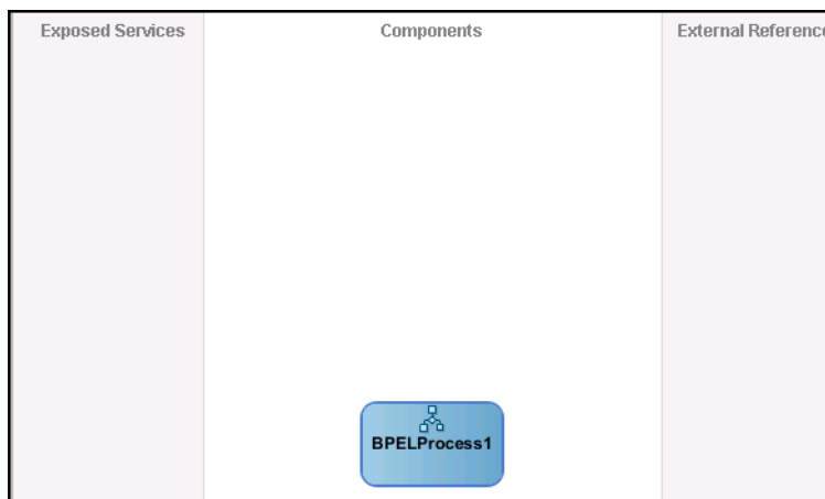
Figure 6–3 Composite View
