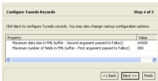
Figure 2–10 The Configure Tuxedo Records screen
