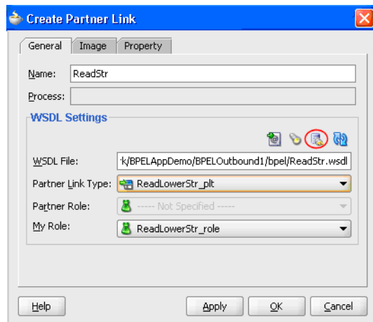
Figure 6–21 Partner Link for File Adapter
