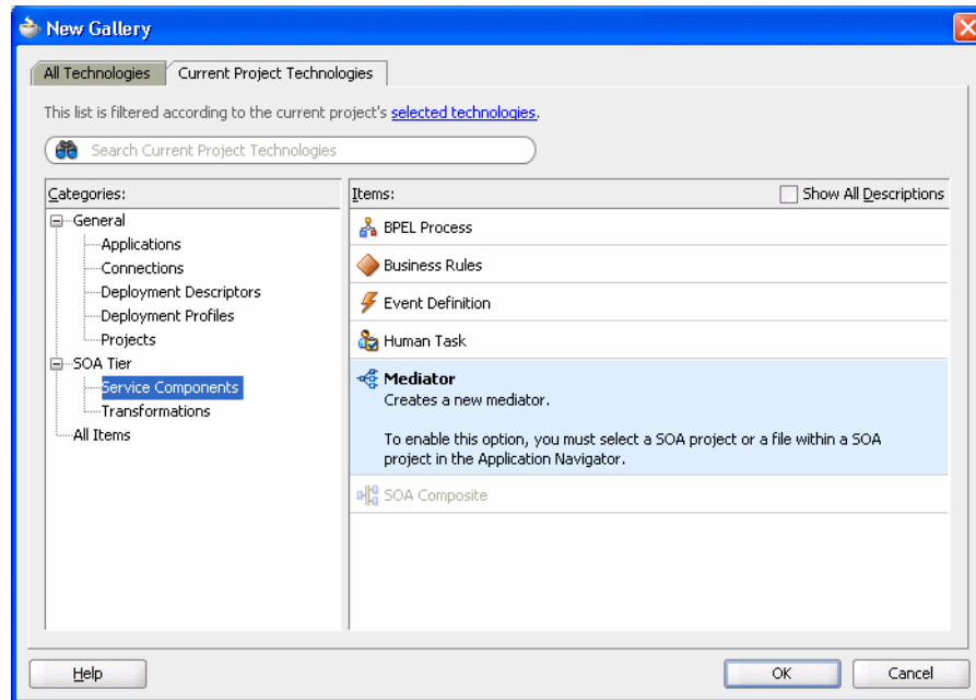
Figure 6–11 New Gallery
