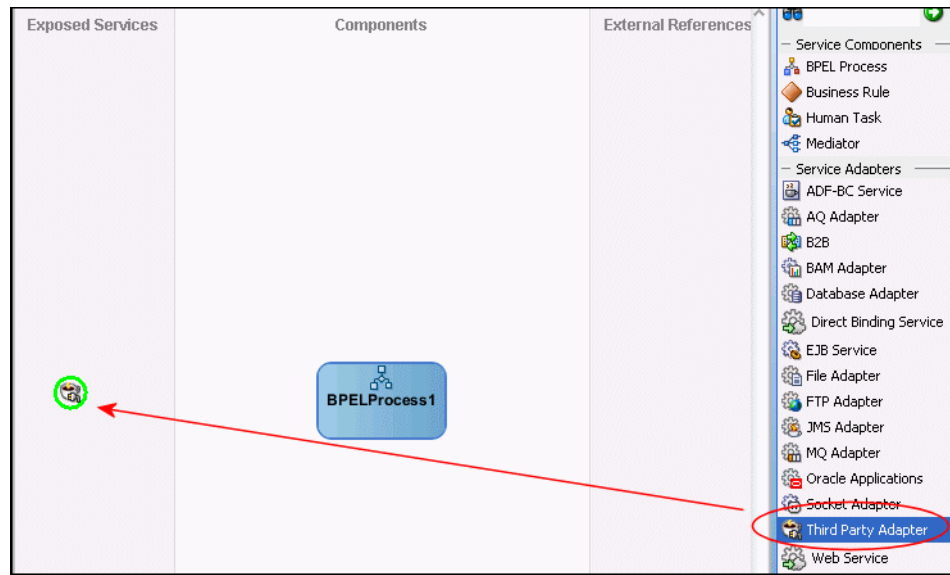
Figure 6–4 Third-Party Adapter
