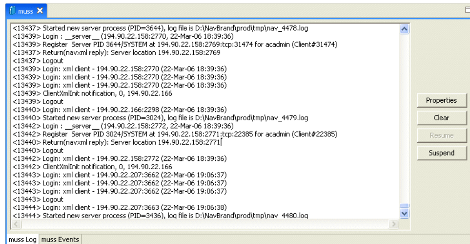
Figure 7-1 The Legacy System Log tab
