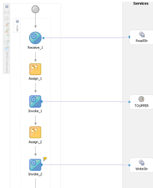
Figure 6–28 Final Outbound Process
