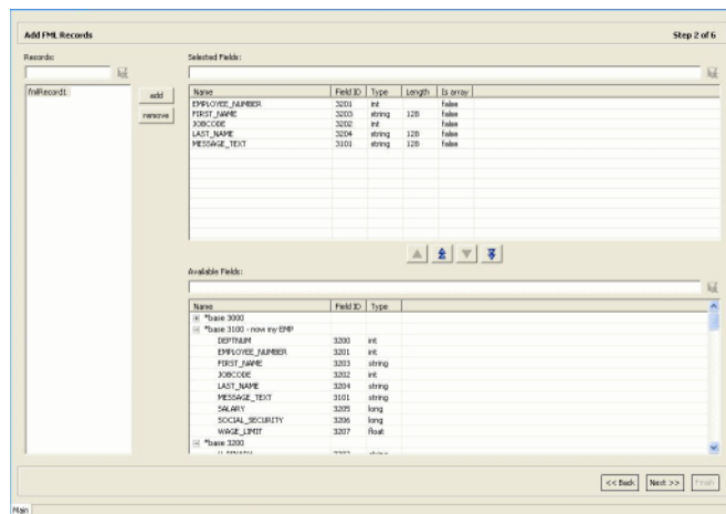
Figure 2–12 Get Tuxedo Records Step
