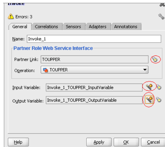
Figure 6–22 Outbound Process
