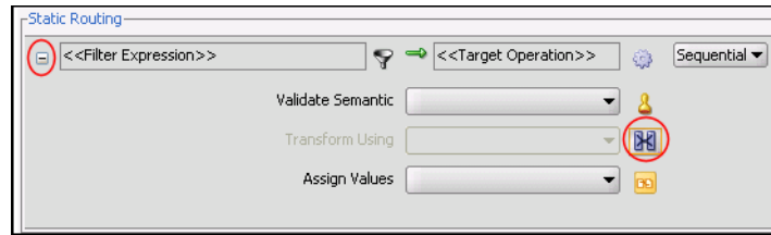
Figure 6–18 Filter Expression
