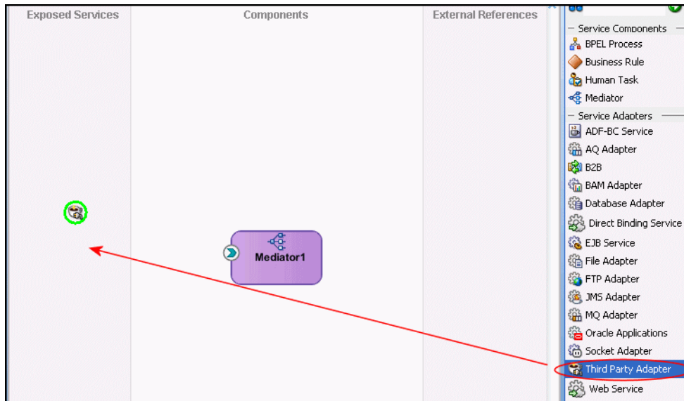
Figure 6–14 Third-Party Adapter
