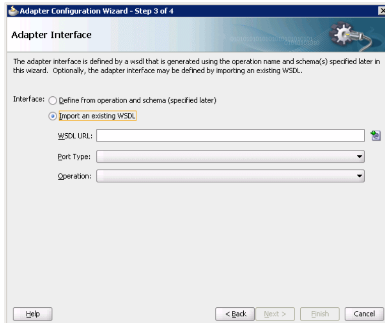
Figure 6–17 File Adapter
