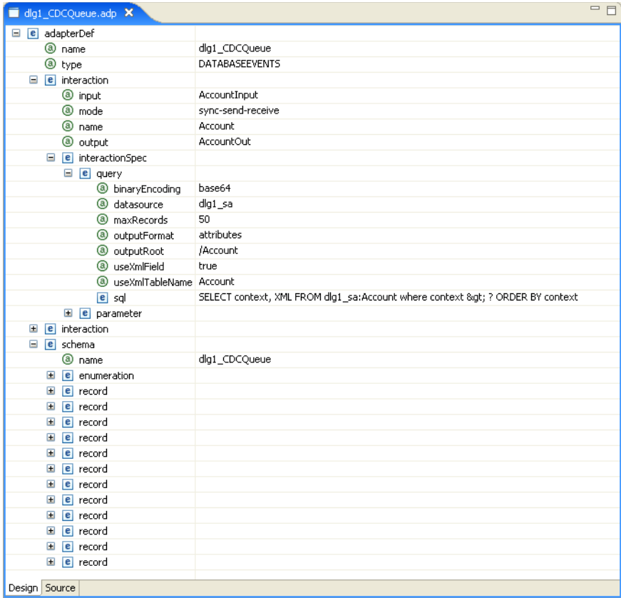
Figure A-5 Adapter Metadata XML Editor
