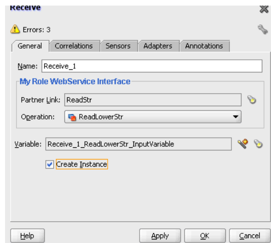
Figure 6–23 Outbound Receive Properties
