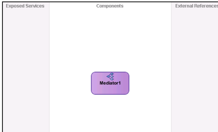
Figure 6–13 Composite View
