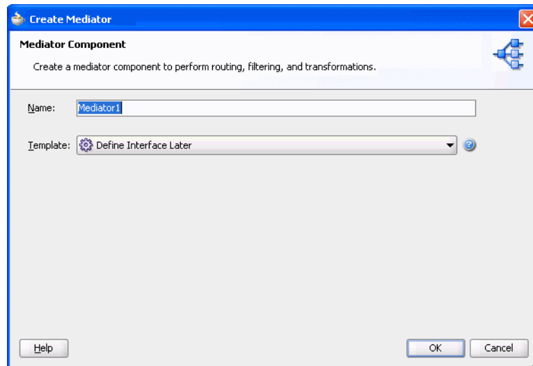
Figure 6–12 Mediator
