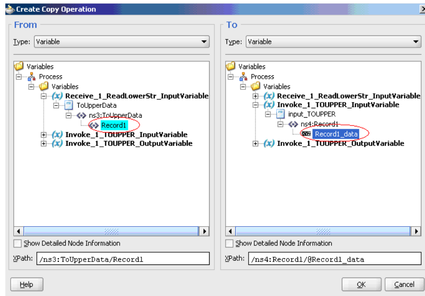
Figure 6–27 Create Copy
