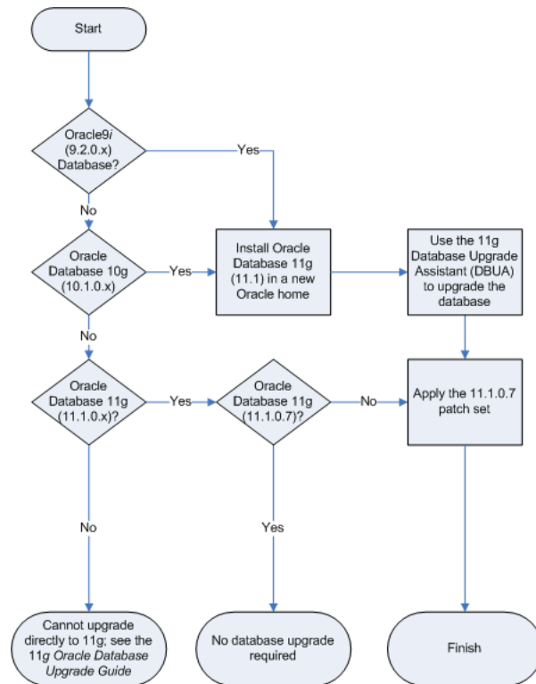
Figure 6–2 Typical Upgrade Path to Oracle Database 11g Release 1 (11.1.0.7)
