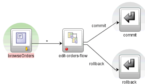
Figure 31–10 ADF Declarative Breakpoint on a Task Flow Activity
