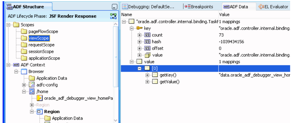
Figure 31–28 Child Scope Selected in the ADF Structure Window
