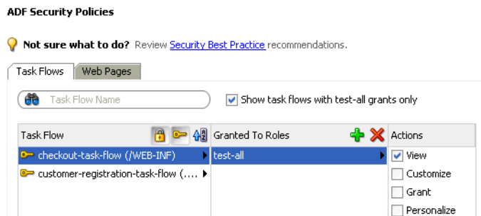
Figure 30–28 Showing Task Flows with test-all Grants in the ADF Policies Overview Editor
