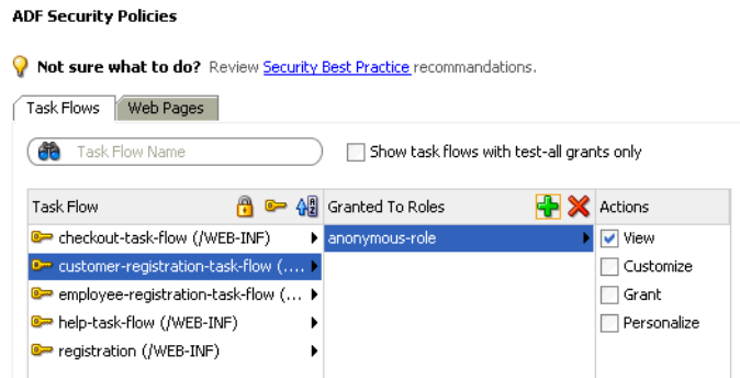
Figure 30–5 Granting to anonymous-role in the ADF Policies Overview Editor
