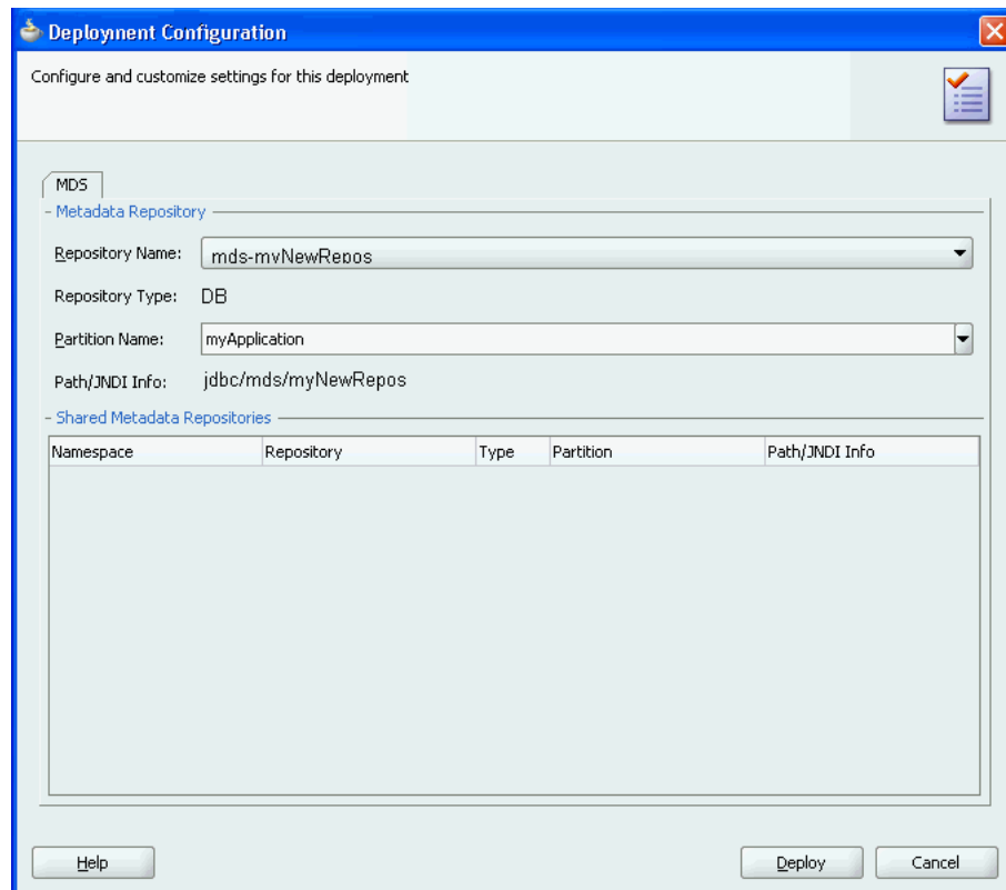
Figure 36–3 MDS Configuration and Customization for Deployment
