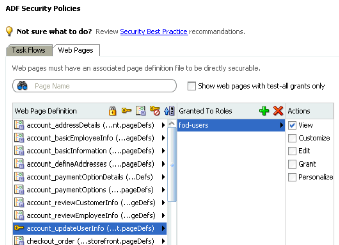
Figure 30–10 Granting to an Application Role for an ADF Page Definition in the ADF Policies Overview Editor
