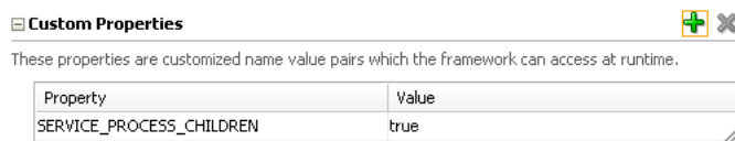
Figure 11–8 Custom Property to Support Nested Processing
