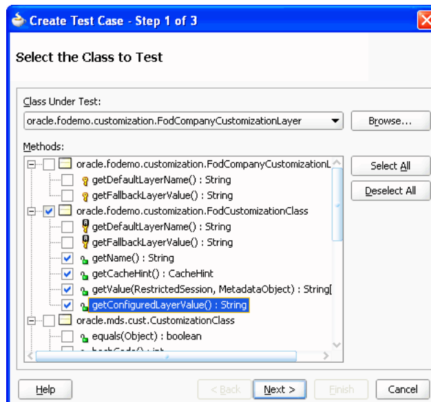
Figure 31–46 Create Test Case Dialog for Selecting Methods to Test
