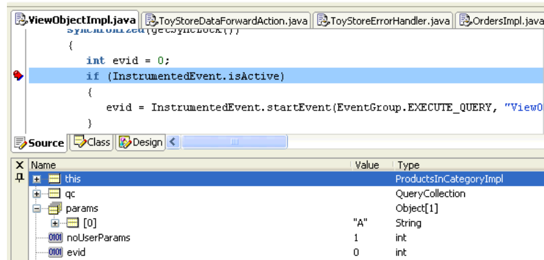
Figure 31-43 Symbol Information Displayed in the Debugger
