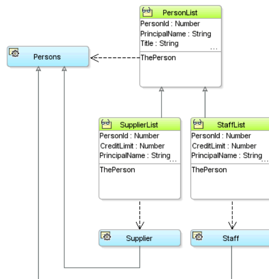
Figure 39–11 Hierarchy of View Object Subtypes Enables View Row Polymorphism
