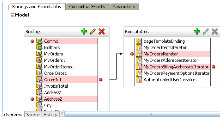
Figure 31-12 ADF Declarative Breakpoints in the Page Definition File
