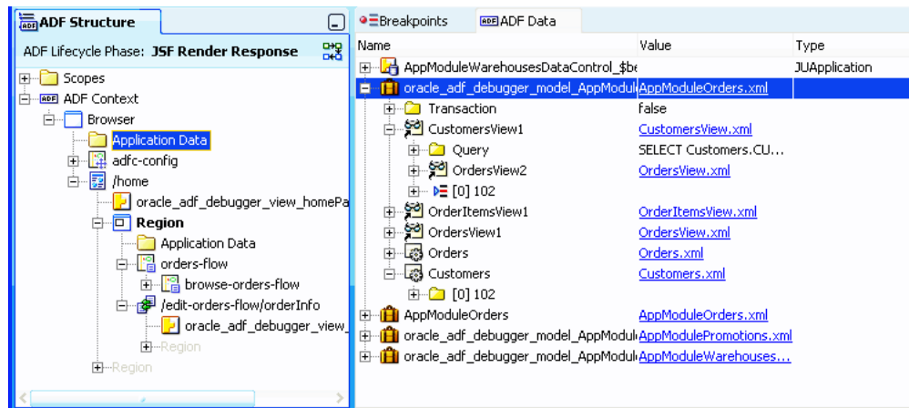
Figure 31–40 Application Data for ADF Business Components Business Services
