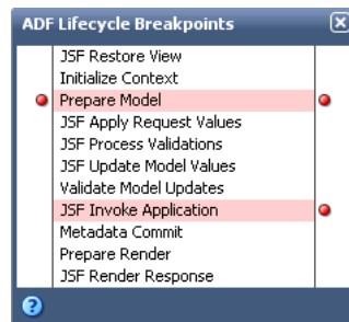
Figure 31–24 Setting Breakpoints in the ADF Lifecycle Breakpoints Window
