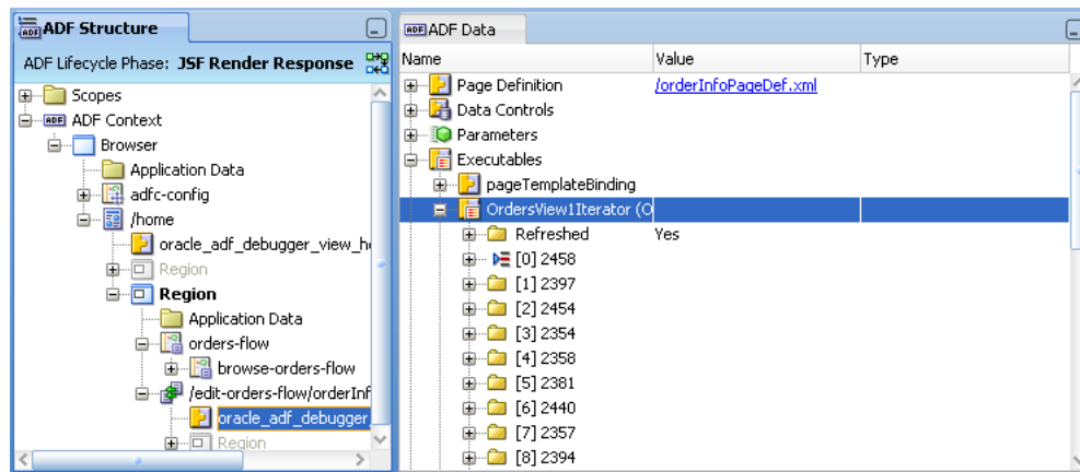
Figure 31–37 Executables Selected for the ADF Data Window
