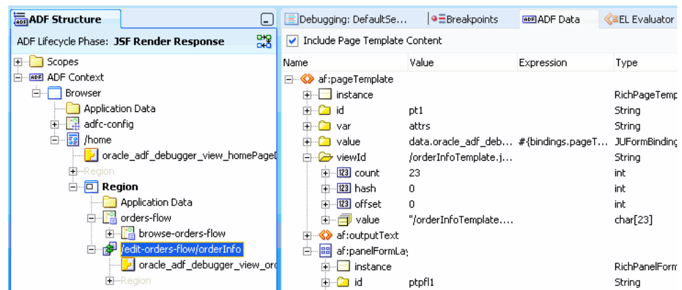
Figure 31–33 Page Selected for the ADF Data Window
