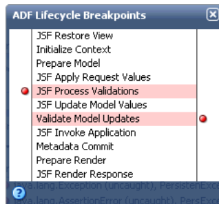
Figure 31–18 ADF Lifecycle Phase Breakpoints Enabled in the ADF Lifecycle Breakpoints Window
