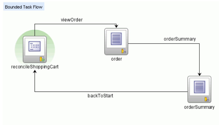
Figure 17–3 Checkout Bounded Task Flow Recycling to Beginning
