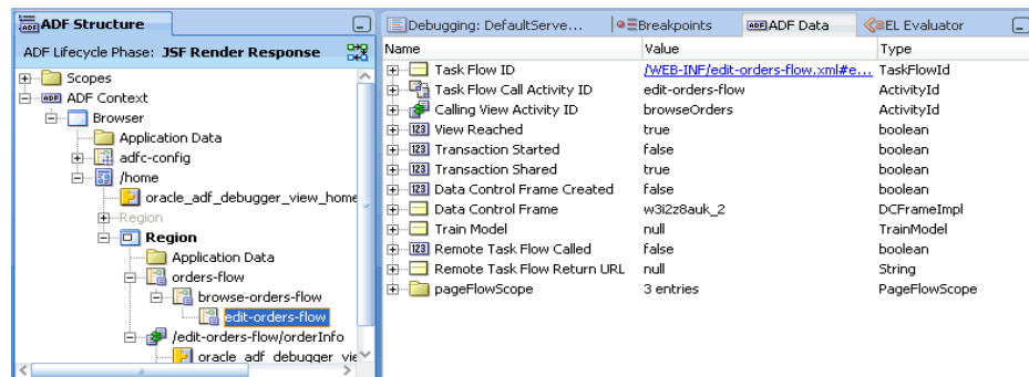
Figure 31-7 ADF Structure Window and ADF Data Window for a Task Flow Selection
