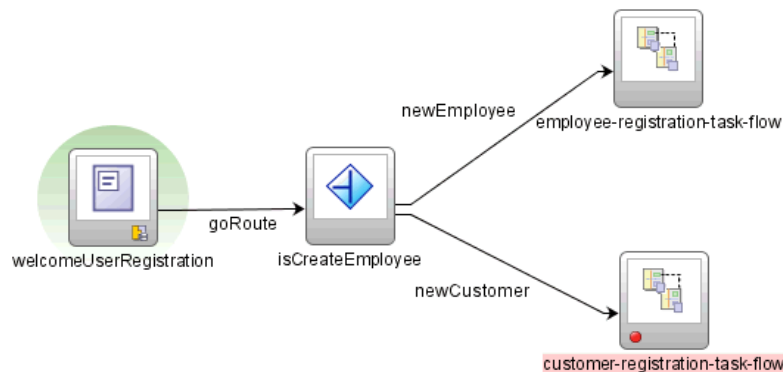
Figure 31–6 ADF Declarative Breakpoint on a Task Flow Activity
