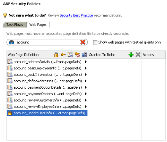
Figure 30–8 Matching Page Definitions by Name in the ADF Policies Overview Editor
