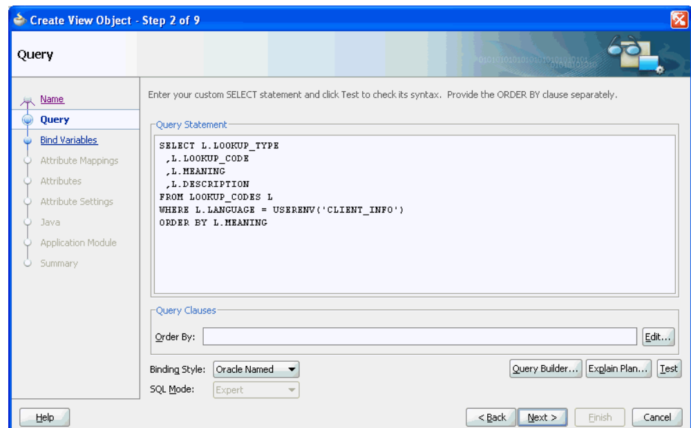
Figure 10-2 Create View Object Wizard, SQL Query for Lookup Table
