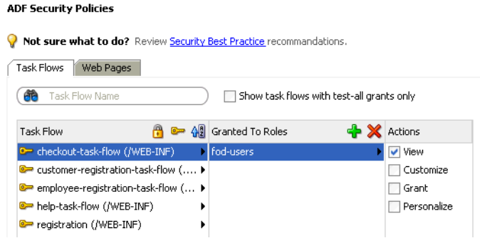
Figure 30–7 Granting to an Application Role for a Bounded Task Flow Definition in the ADF Policies Overview Editor
