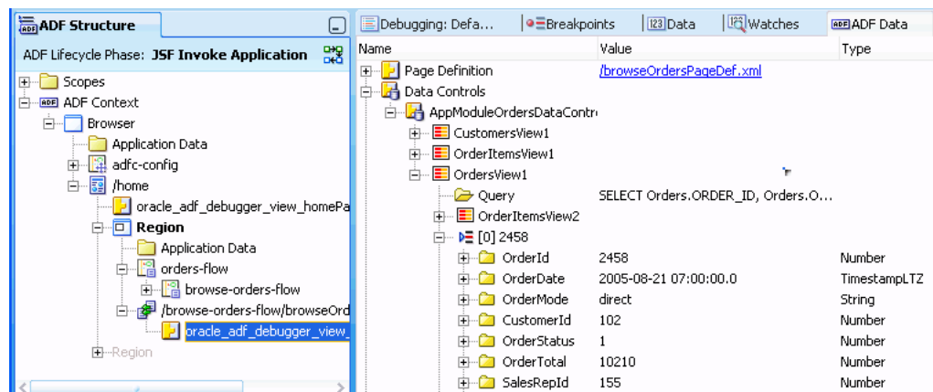
Figure 31-35 Binding Container (Business Components) Selected for the ADF Data Window
