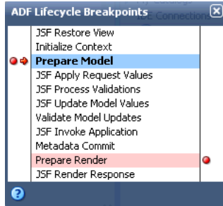
Figure 31–22 Application Paused at an Execution Point on an ADF Lifecycle Phase
