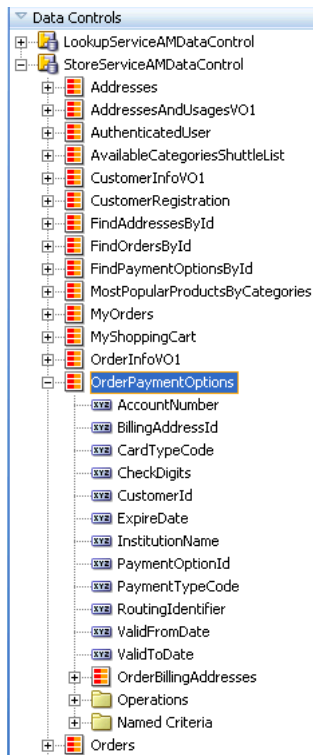
Figure 1–15 StoreFrontServiceAMDataControl
