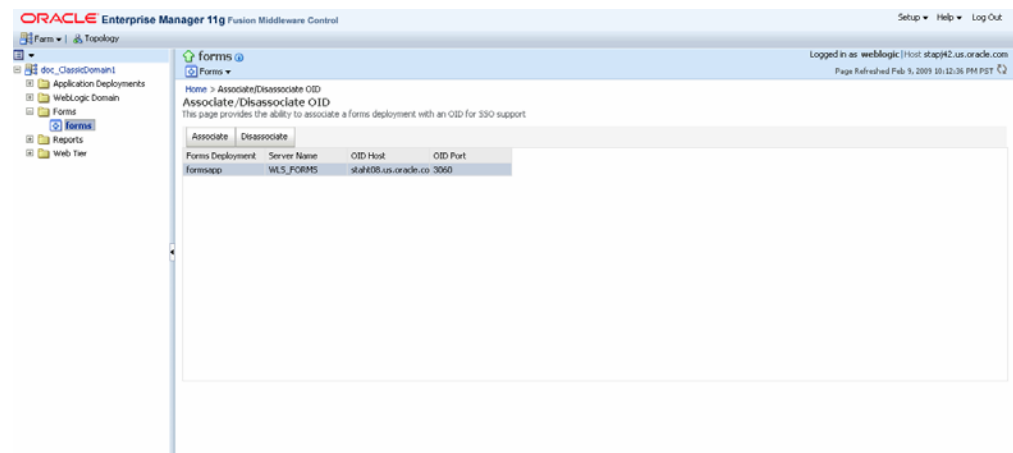
Figure 9–4 Associate/Disassociate OID
