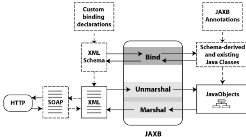
Figure 5–1 Data Binding With JAXB
