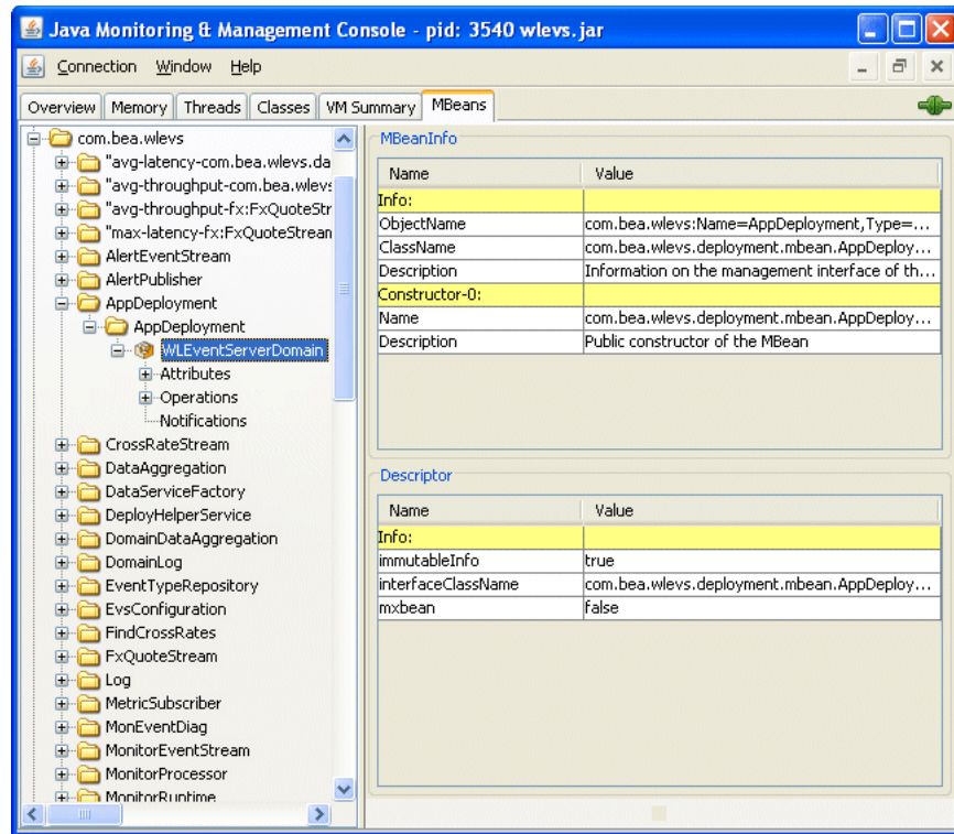
Figure 11-6 JConsole Browser
