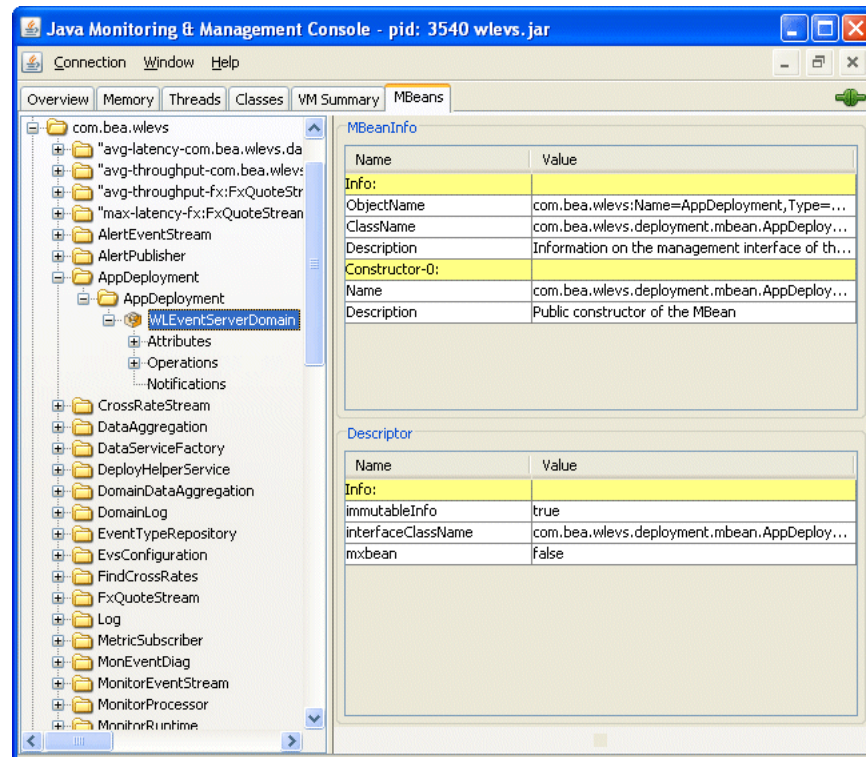
Figure 11–5 JConsole Browser
