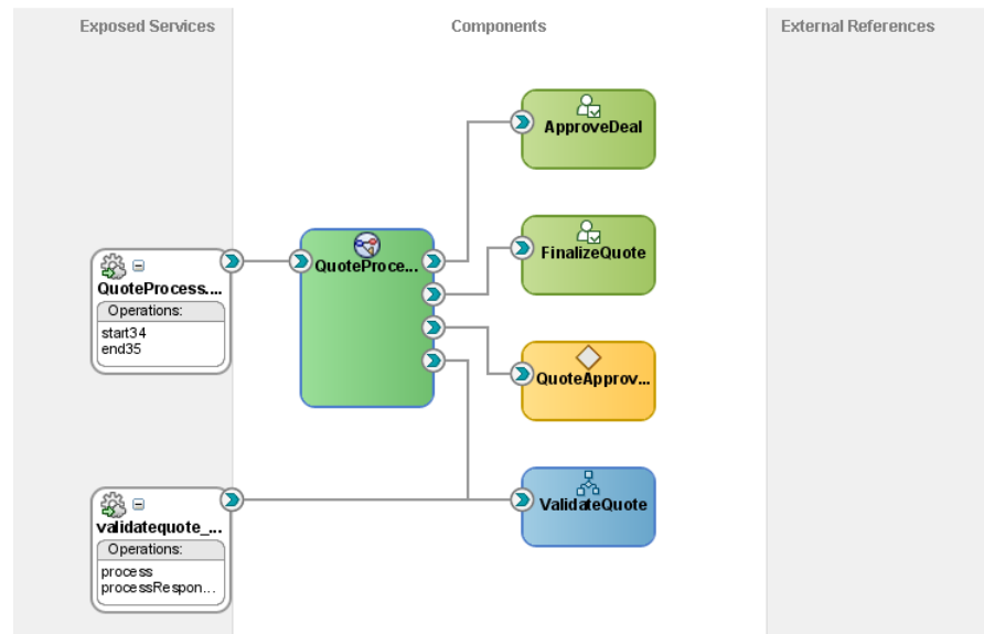
Figure 22–1 BPMN process in an SOA Composite
