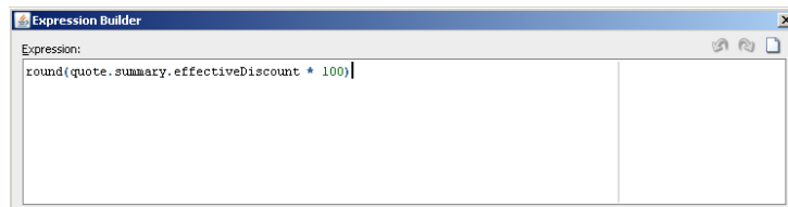
Figure 6–47 Expression Used to Change the Value of Discount Project Variable
