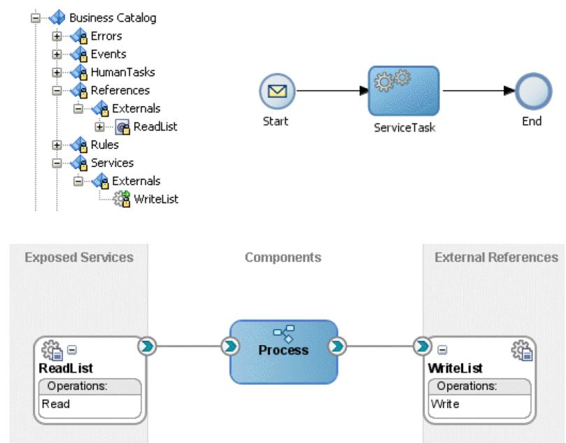
Figure 15–2 Adapter Services in Oracle BPM
