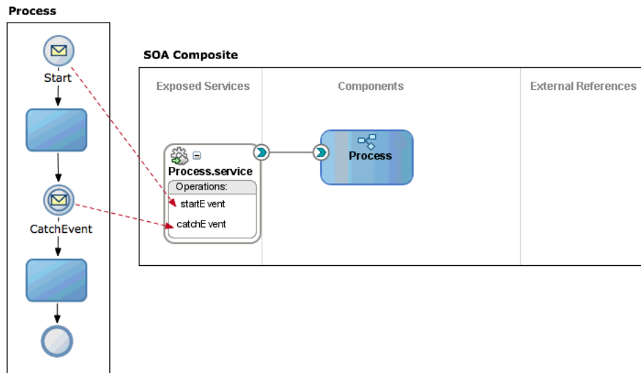
Figure 20–2 BPMN process that exposes a message start and a message catch event in its interface
