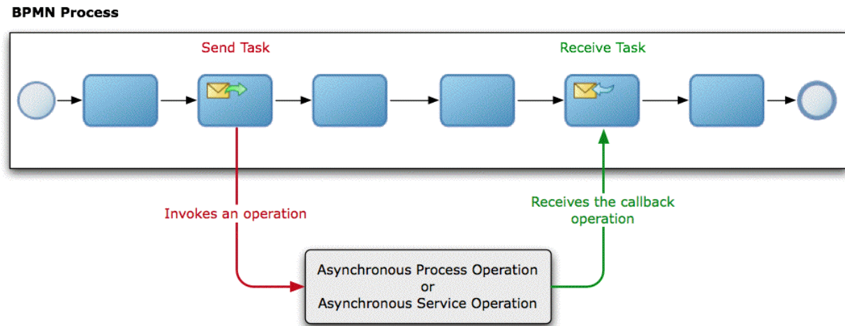
Figure 19–3 Invoking an asynchronous service or BPMN process using send and receive tasks
