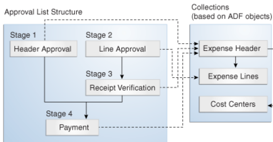
Figure 25–4 Mapping of Stages and Collections
