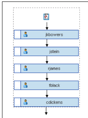
Figure 25–69 After Move
