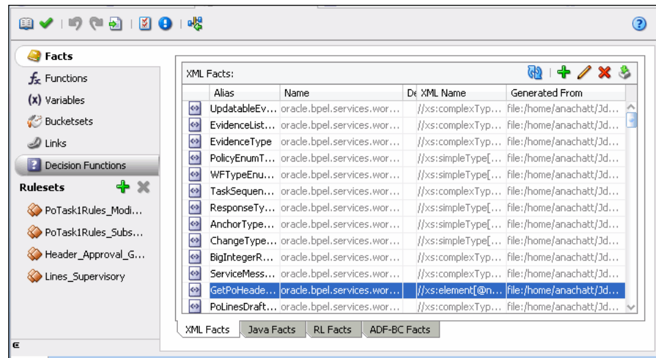
Figure 25–35 Facts List
