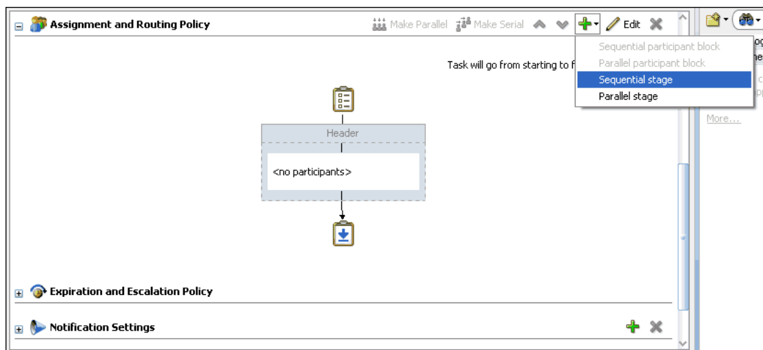
Figure 25-14 Create Stage
