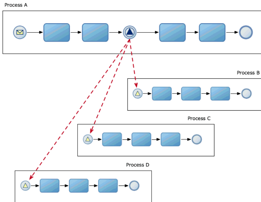
Figure 19–4 Signal Broadcast
