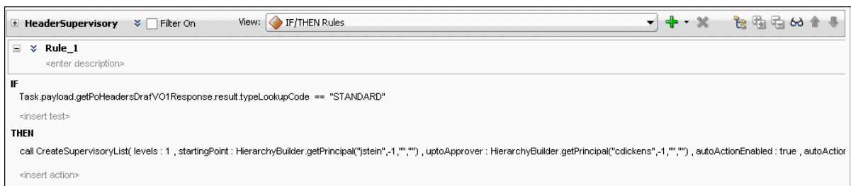
Figure 25–30 Example Rules (1)
