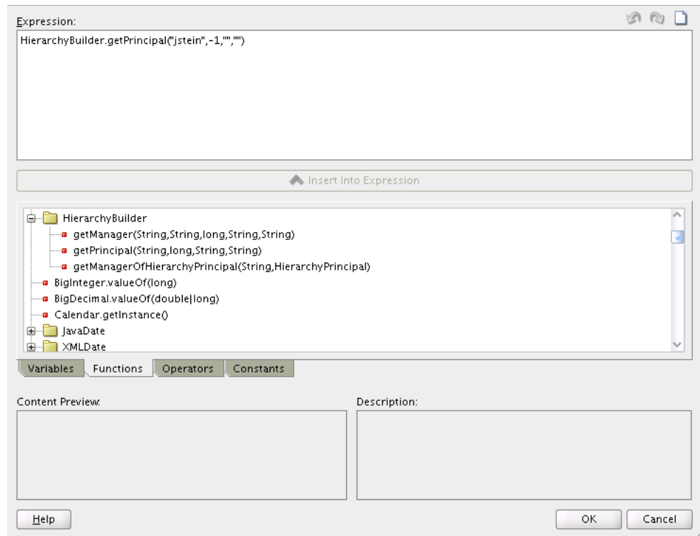
Figure 25–29 HierarchyBuilder Function
