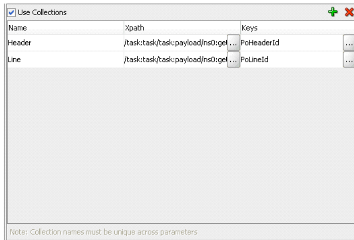
Figure 25–11 Defining Collections
