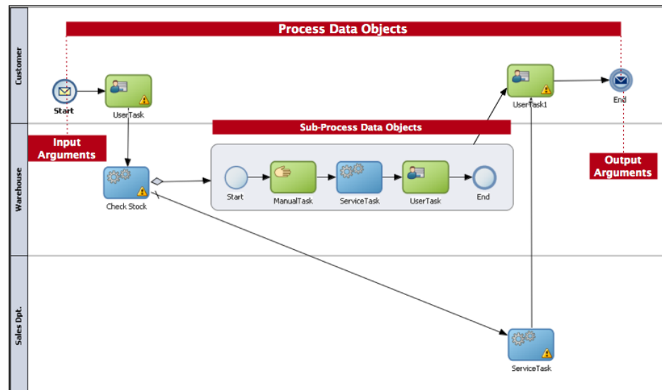
Figure 8-3 Scope of the Data Structures in a Process
