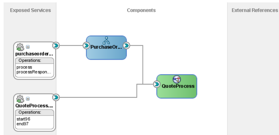
Figure 22–2 BPMN Process as a Partner Link in a BPEL Process
