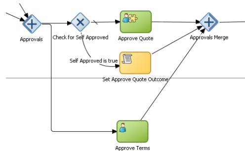
Figure 6–35 Example of a Parallel Gateway
