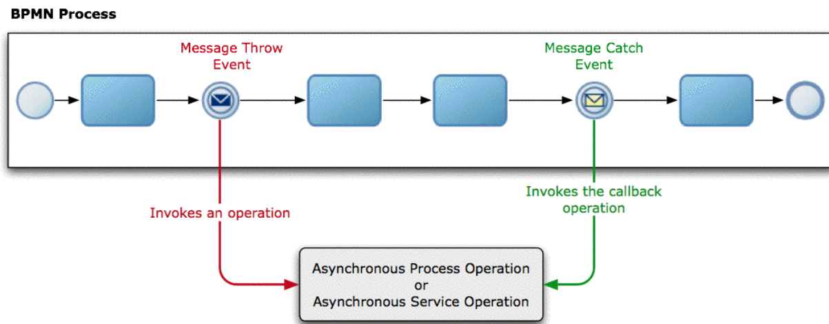
Figure 19–1 Invoking an Asynchronous Service or BPMN Process Using Message Events
