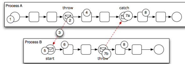
Figure 6–24 Using Message Throw and Catch Events Between Processes
