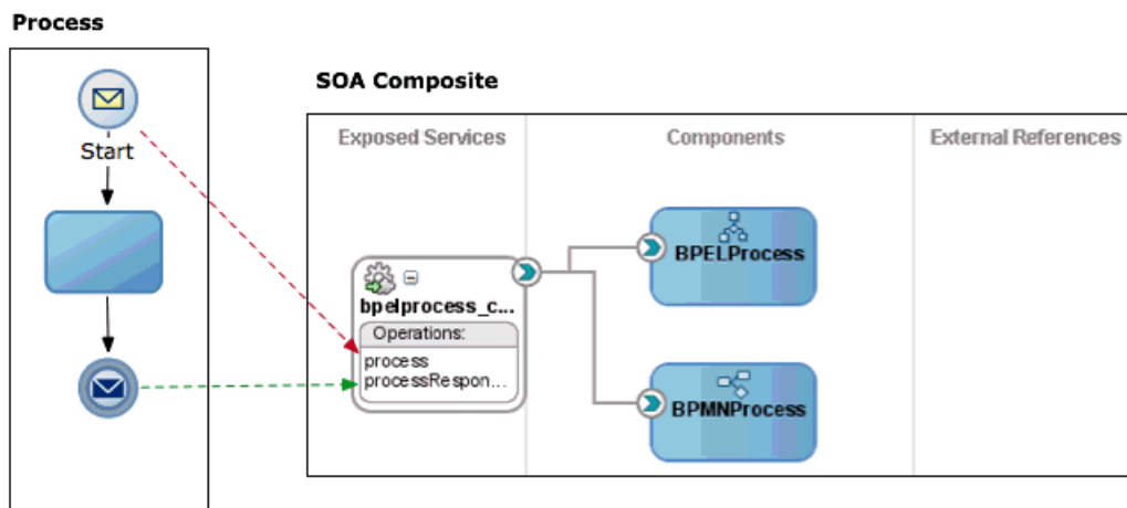
Figure 20–4 Process That Uses an Interface from the Business Catalog
