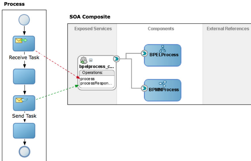
Figure 20–5 BPMN process that exposes an asynchronous operation defined using send and a receive task
