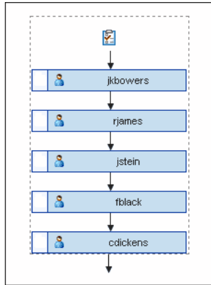
Figure 25–69 After Move
