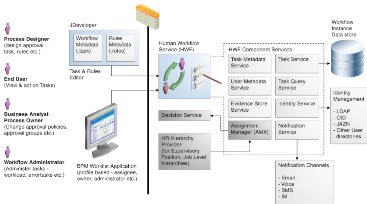
Figure 25–1 Overall Architecture
