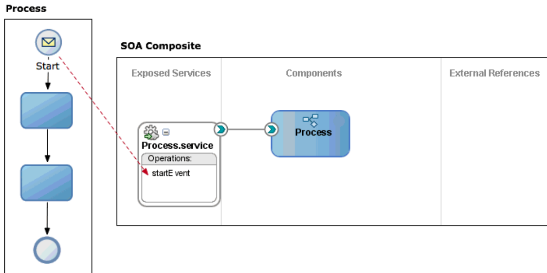
Figure 20–1 BPMN Process that exposes a message start event as an operation
