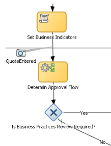
Figure 6–26 The Business Rules Task within the Sales Quote Example Process
