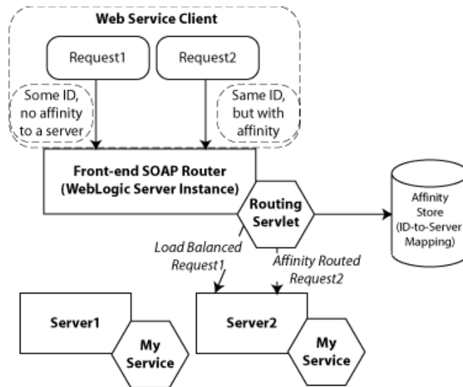
Figure 4-3 Routing Web Service Requests to a Single Server Using an ID
