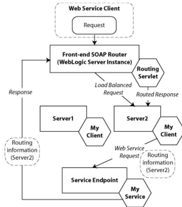
Figure 4–1 Routing a Web Service Response to a Single Server
