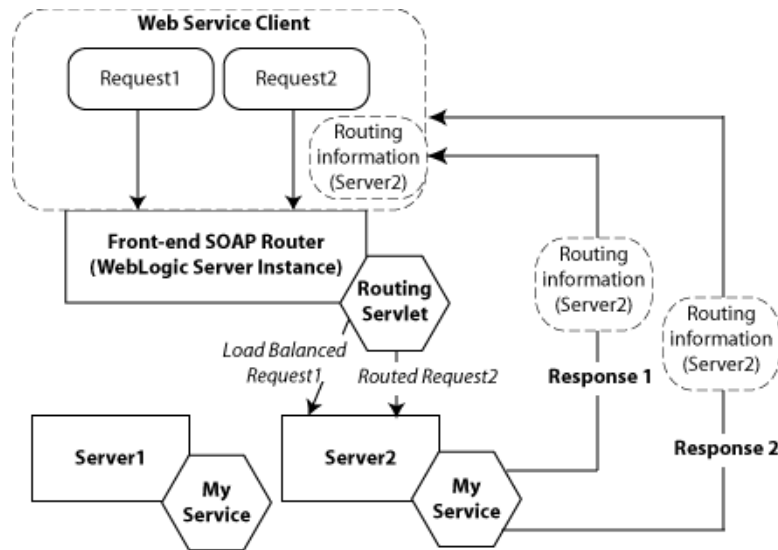
Figure 4–2 Routing Web Service Requests to a Single Server
