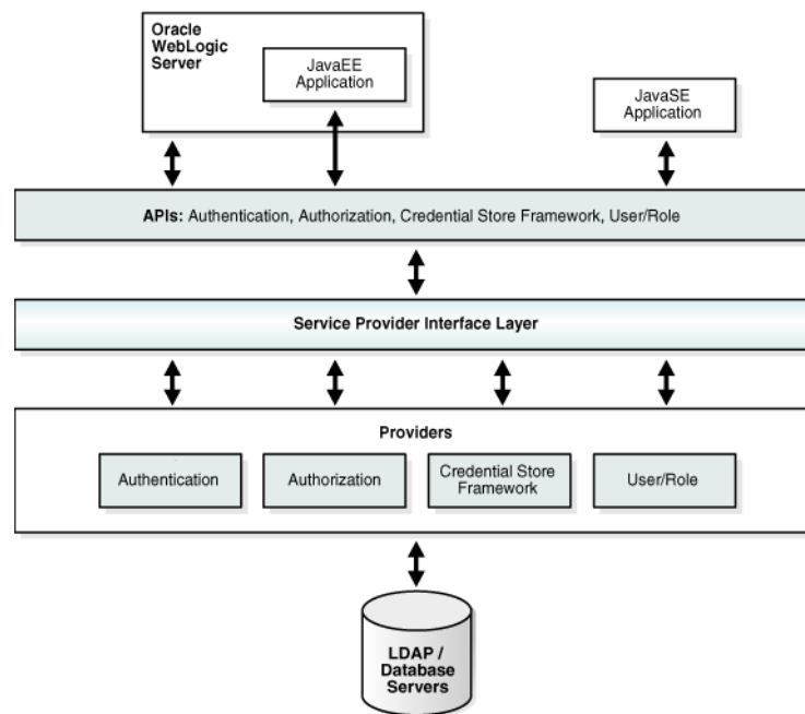
Figure 18–1 OPSS Architecture
