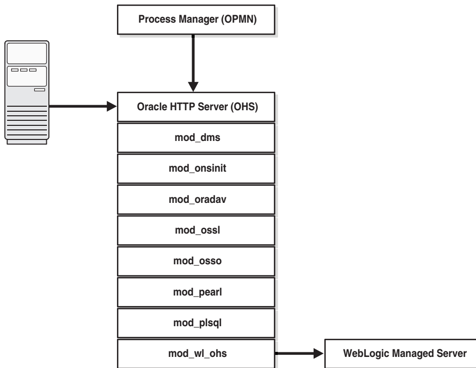
Figure 11–1 Oracle HTTP Server Architecture
