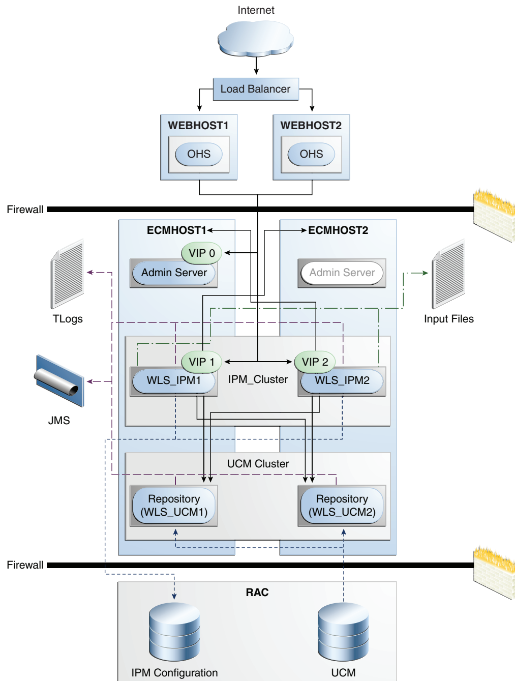
Figure 10–2 Oracle I/PM High Availability Architecture Diagram
