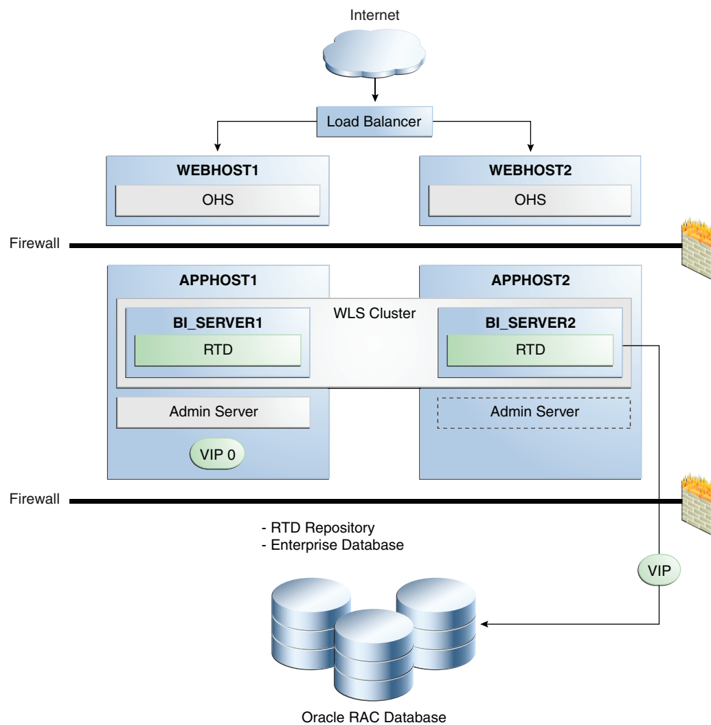
Figure 15-10 Oracle RTD High Availability Architecture
