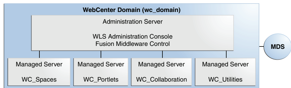
Figure 6-4 Basic Single-Node Oracle WebCenter Architecture
