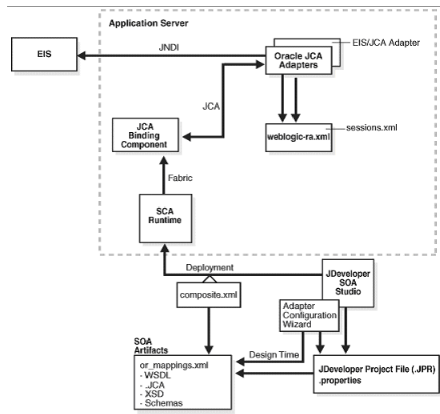
Figure 5–30 Oracle JCA Adapters Single-Instance Architecture
