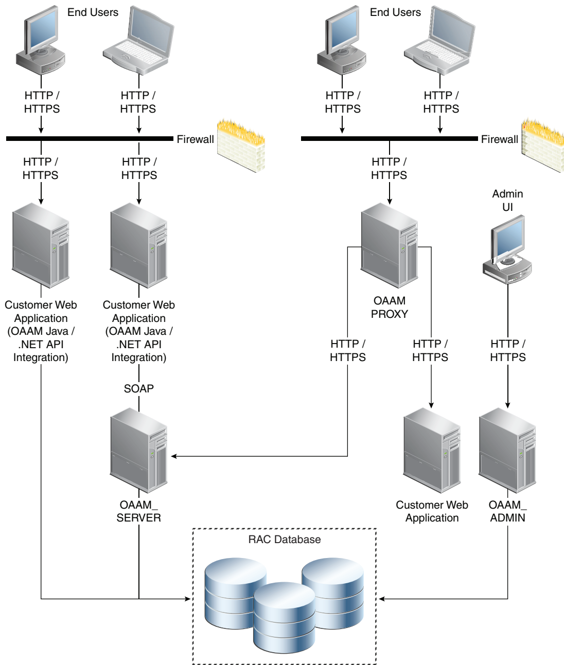
Figure 8–16 Oracle Adaptive Access Manager Single Instance Architecture
