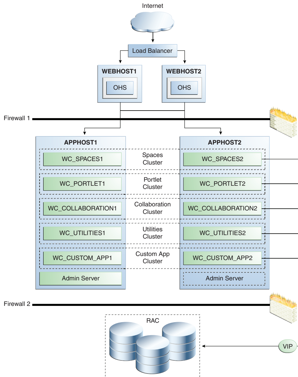
Figure 6–5 Oracle WebCenter Two-Node High Availability Architecture
