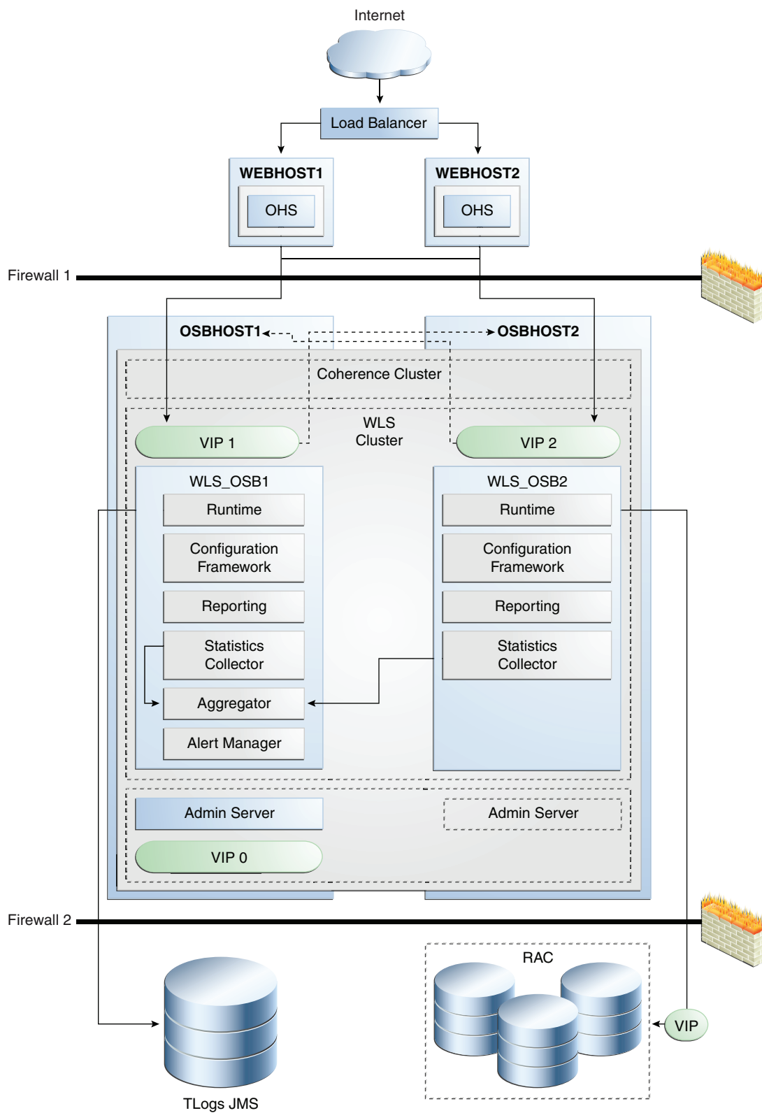
Figure 5–41 Oracle Service Bus High Availability Architecture
