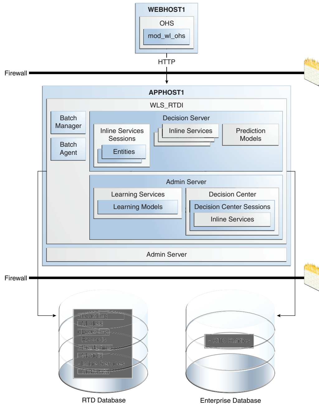
Figure 15–9 Oracle RTD Single Instance Architecture
