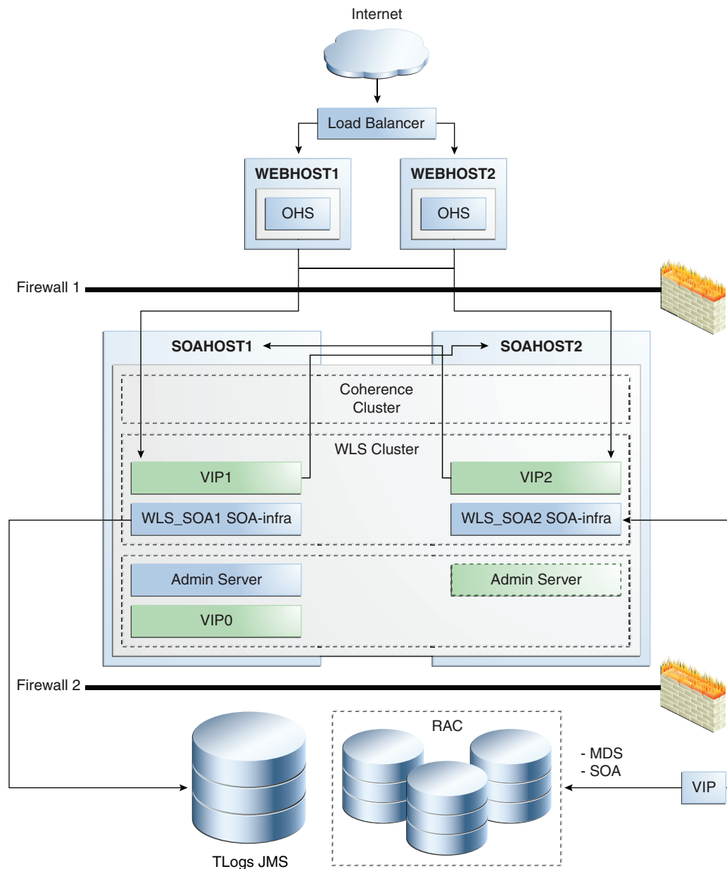
Figure 5–42 Oracle SOA Service Infrastructure High Availability Architecture
