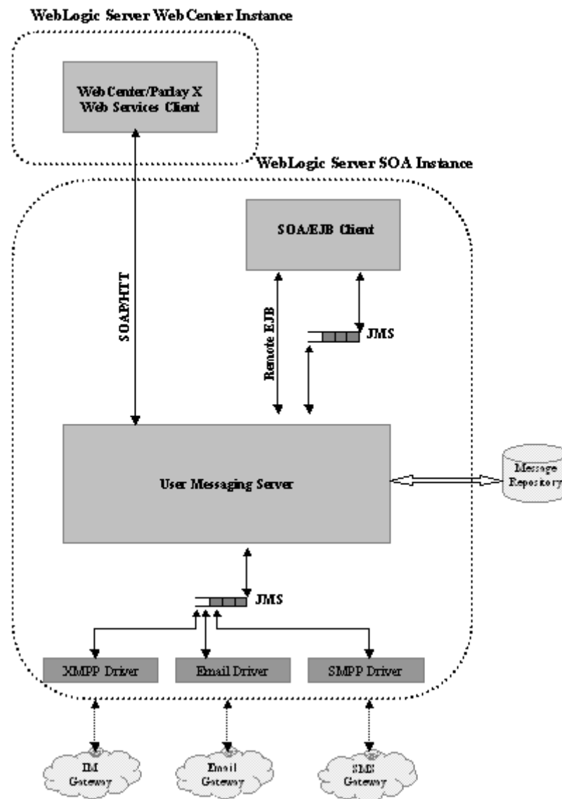
Figure 5–28 Oracle User Messaging Service Single-Instance Architecture
