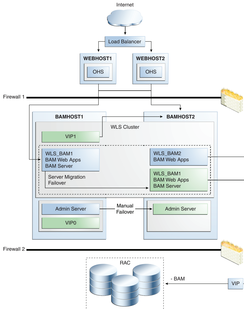
Figure 5–53 Oracle BAM High Availability Architecture
