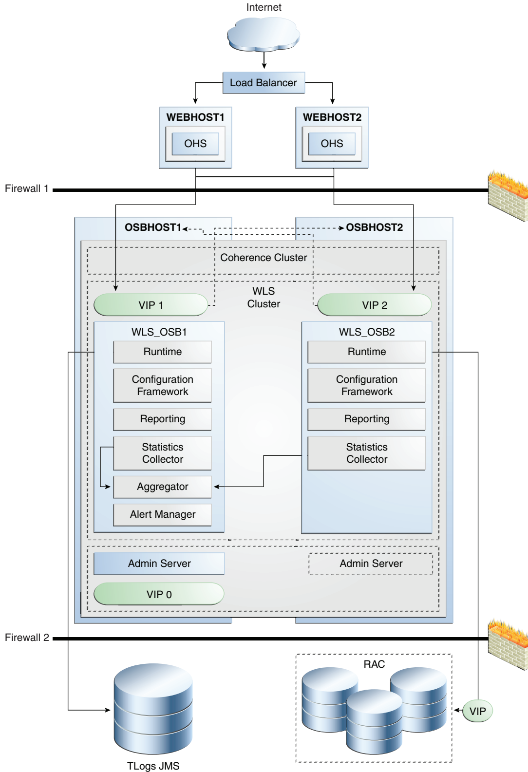
Figure 5–47 Oracle SOA Service Infrastructure, Component Services Engines, and Oracle Service Bus High Availability Architecture
