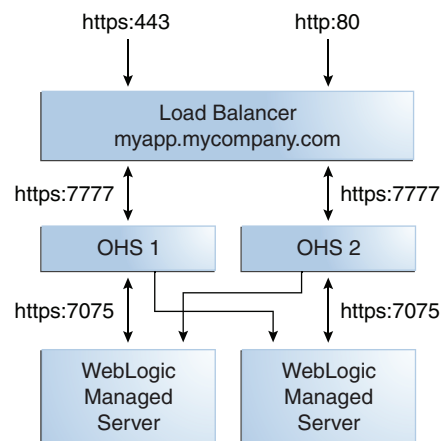
Figure 11–2 Oracle HTTP Server High Availability Architecture
