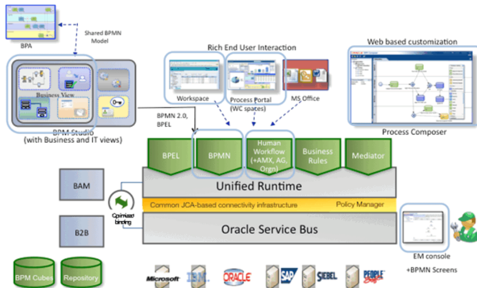
Figure 5–1 Oracle Fusion Middleware SOA Suite and Components
