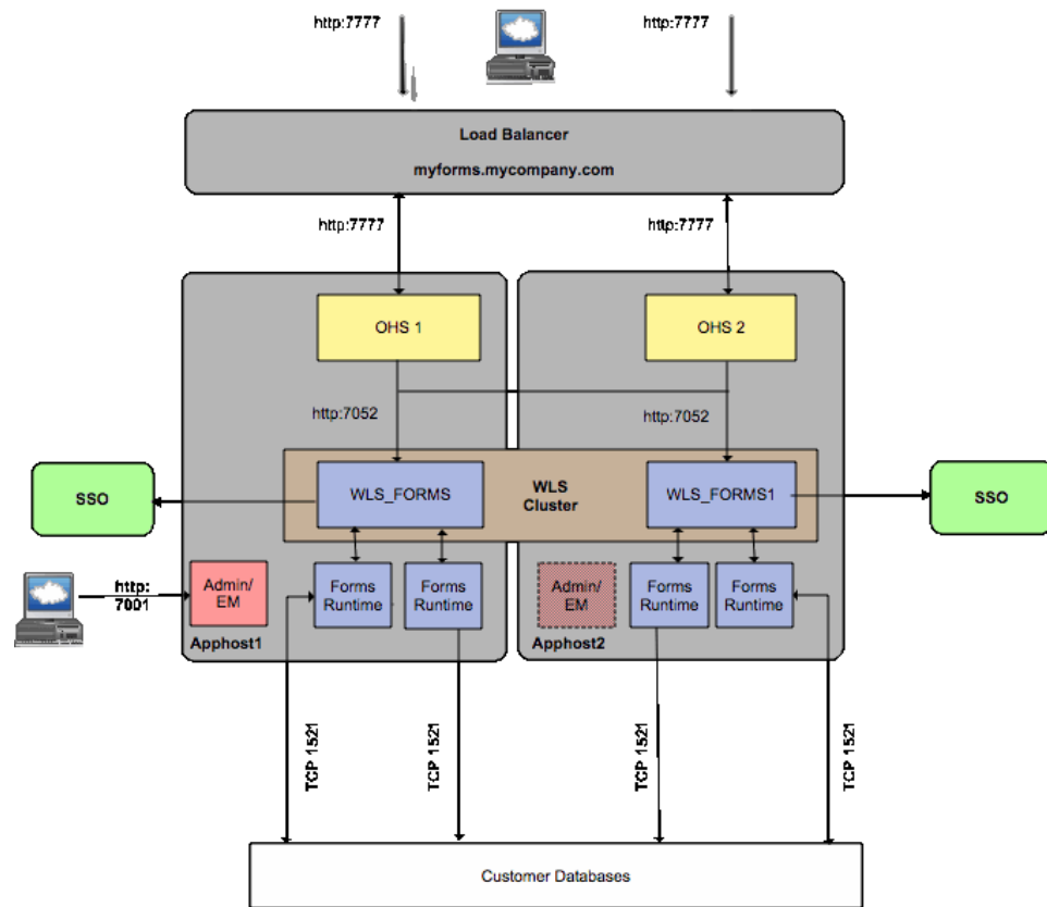
Figure 14–4 Oracle Forms High Availability Deployment
