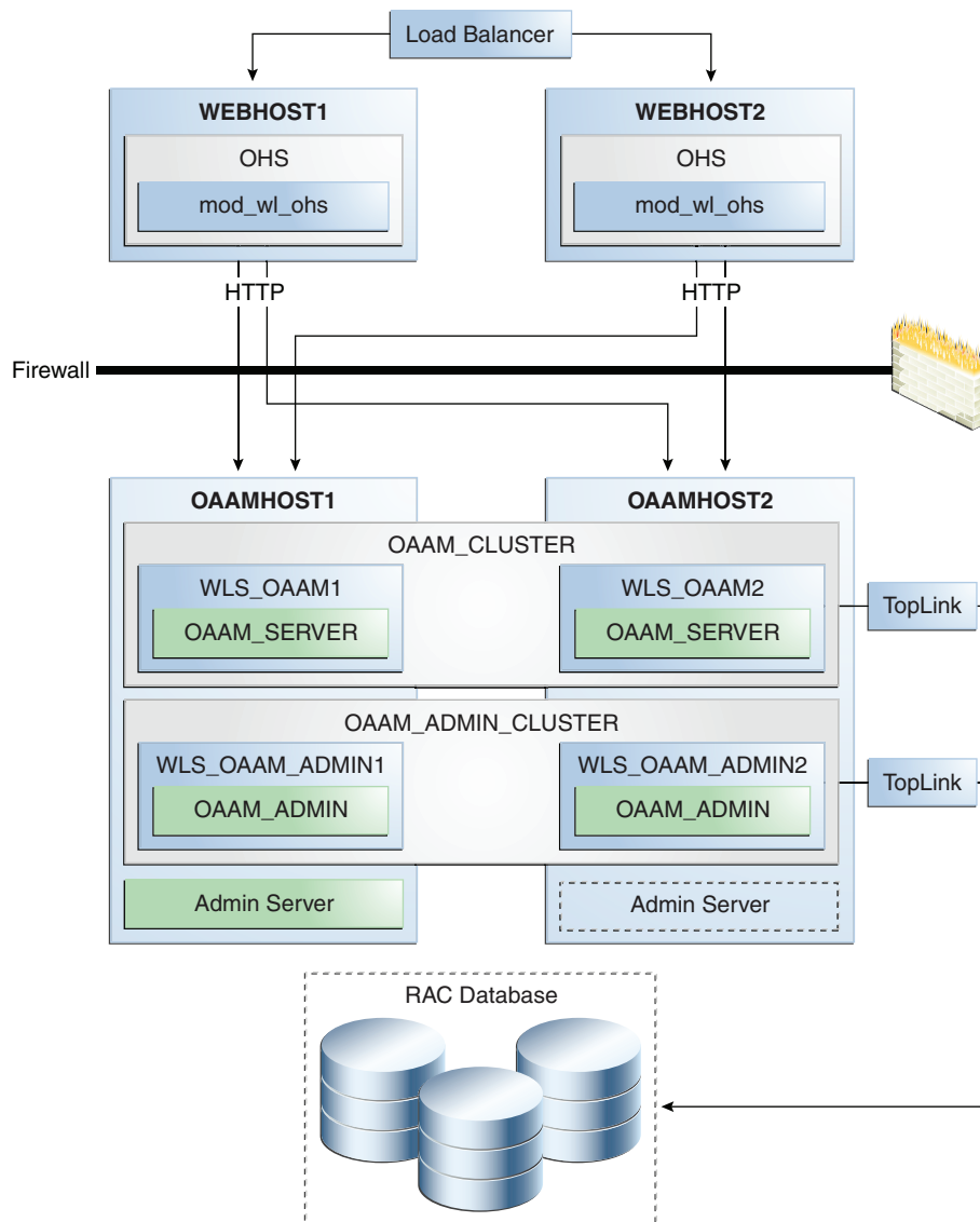
Figure 8–17 Oracle Adaptive Access Manager High Availability Architecture
