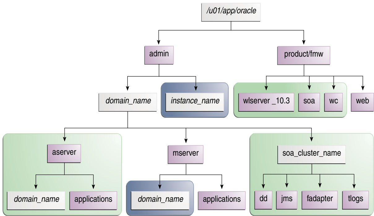
Figure 2–2 Directory Structure
