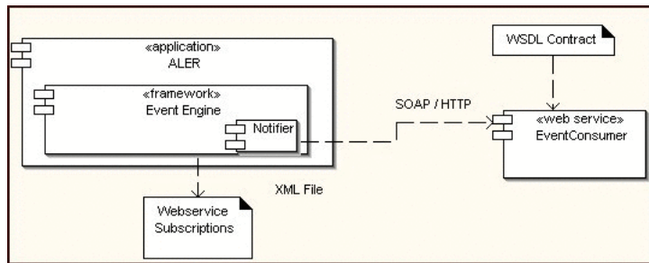
Figure 9–49 Web Service Endpoint Plug-in
