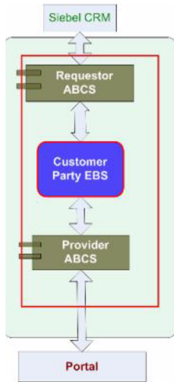
Figure 15–11 Transaction Boundary
