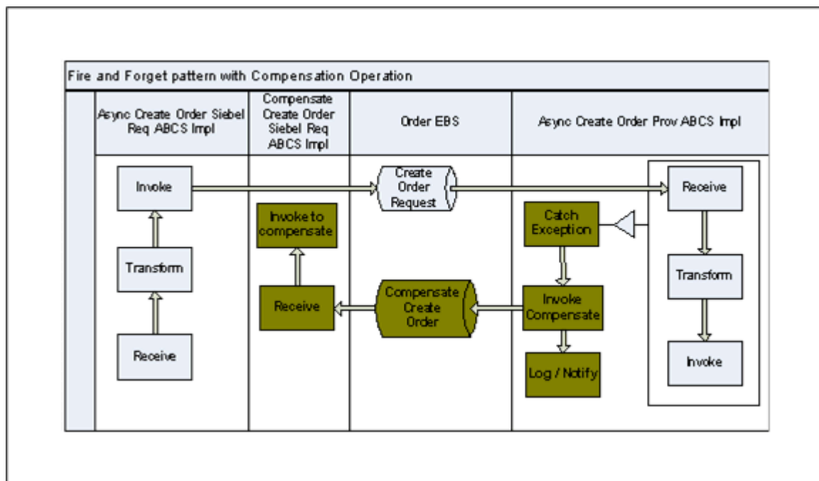
Figure 12-3 Fire-and-Forget Pattern with Compensation Operation
