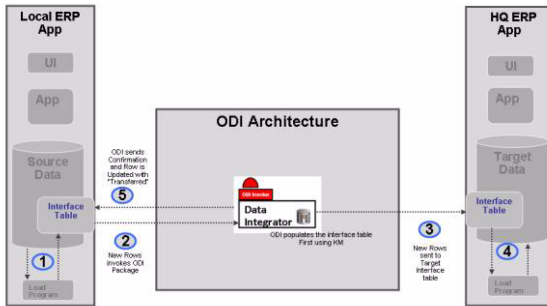
Figure 22–3 High-Volume Transactions
