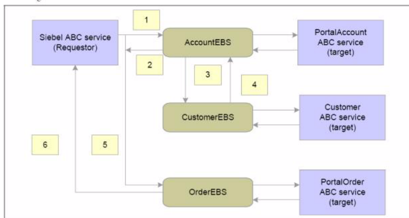
Figure 23–15 ProcessOrder flow
