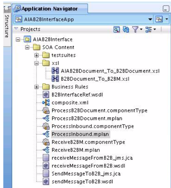
Figure 20–8 ProcessInbound.mplan
