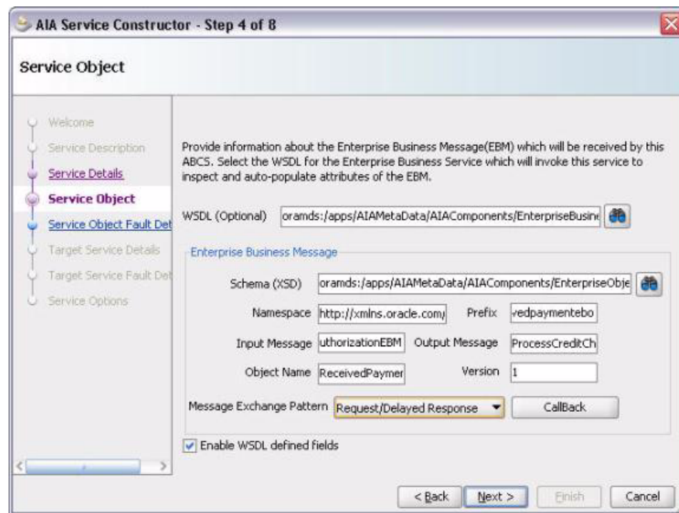
Figure 4–19 CallBack Button
