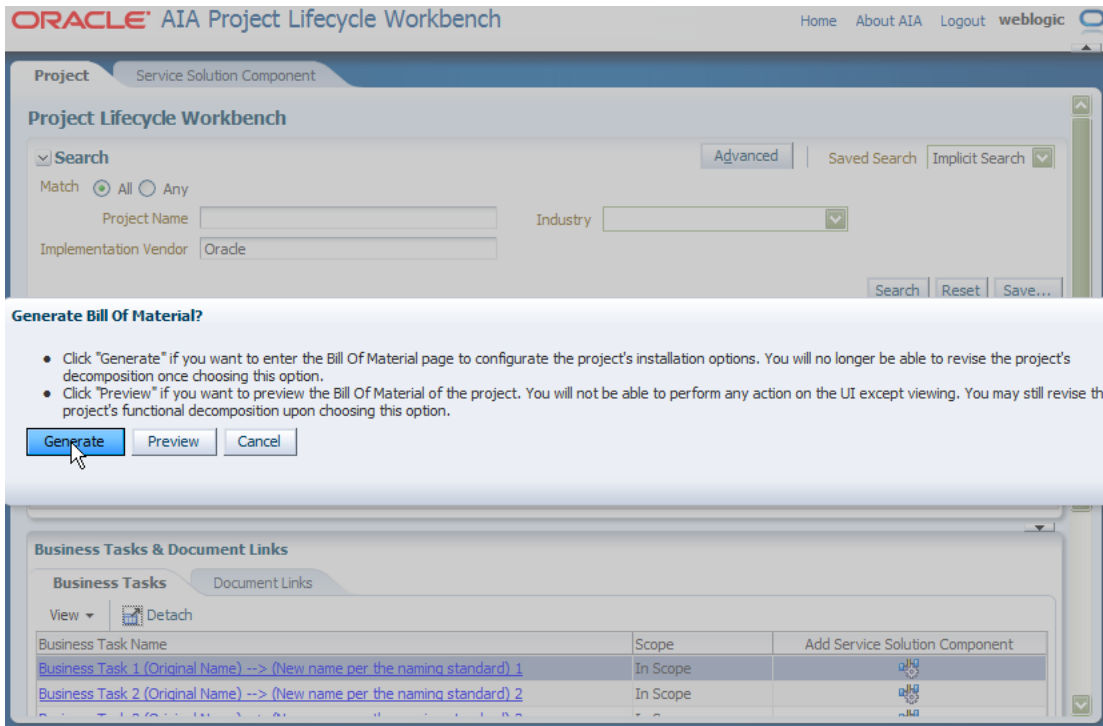
Figure 3–17 Click Generate
