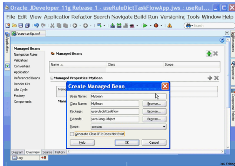
Figure 26–53 Specifying the Bean Name and Scope in the Task Flow Application
