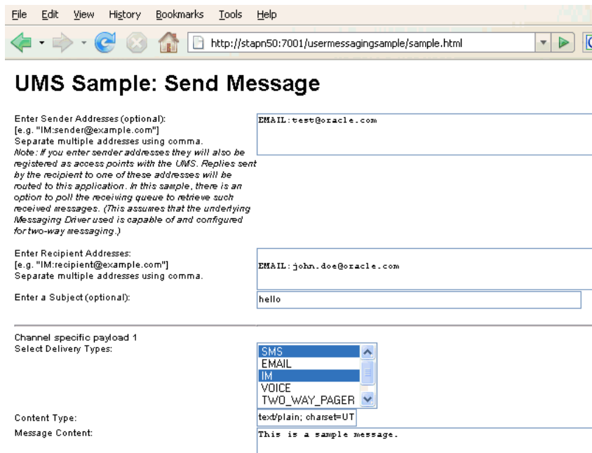
Figure 61–6 Addressing the Test Message
