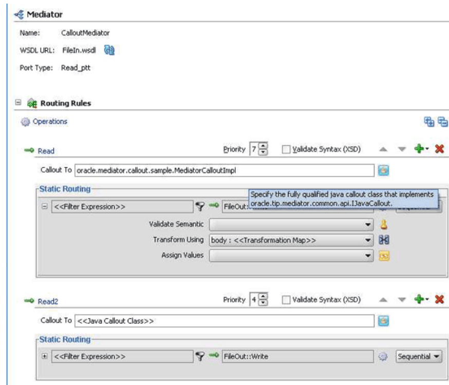
Figure 20–27 Sample Oracle Mediator Supporting Java Callout
