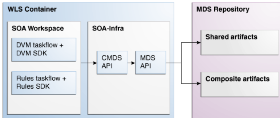
Figure 45-1 Oracle SOA Composer High-Level Deployment Topology
