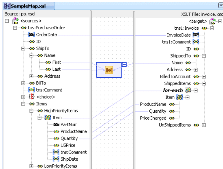
Figure 38–3 Design View Mapping
