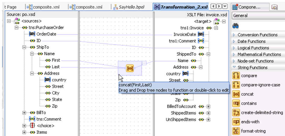
Figure 38–18 Using the Concat Function
