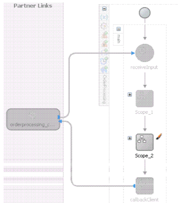
Figure 16–4 One Customizable Scope
