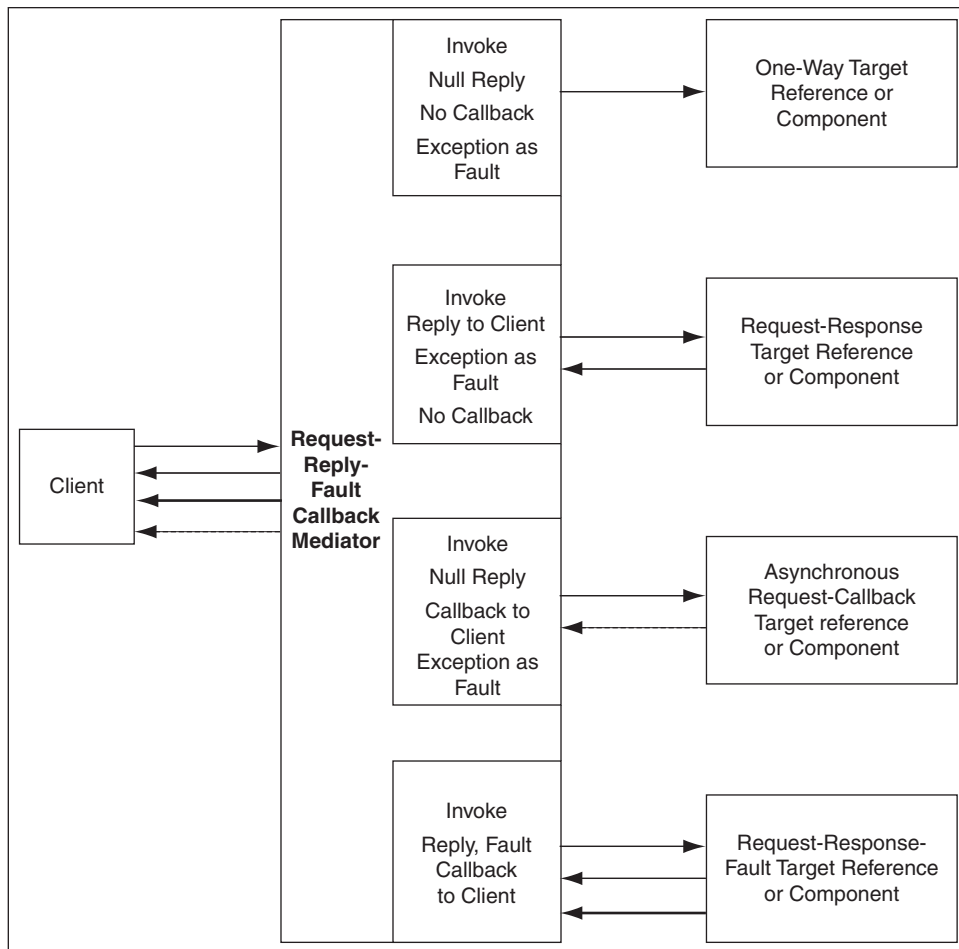
Figure 24–6 Request-Reply-Fault-Callback Message Exchange Pattern
