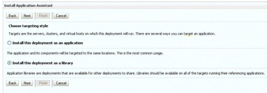
Figure 26–25 Deploying oracle.soa.rules_editor_dc.webapp Shared Library
