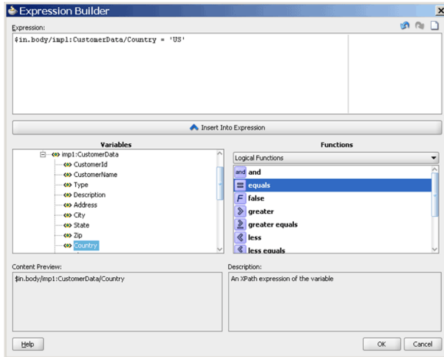
Figure 20–43 Expression Builder Dialog
