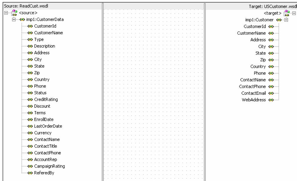
Figure 20-45 CustomerData_To_Customer.xml File – Initially
