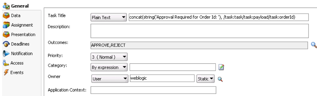
Figure 28–6 Human Task Editor — General Section
