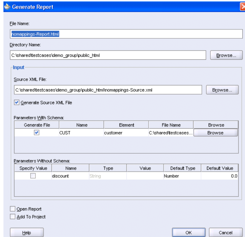
Figure 38–50 The Generate Report Dialog
