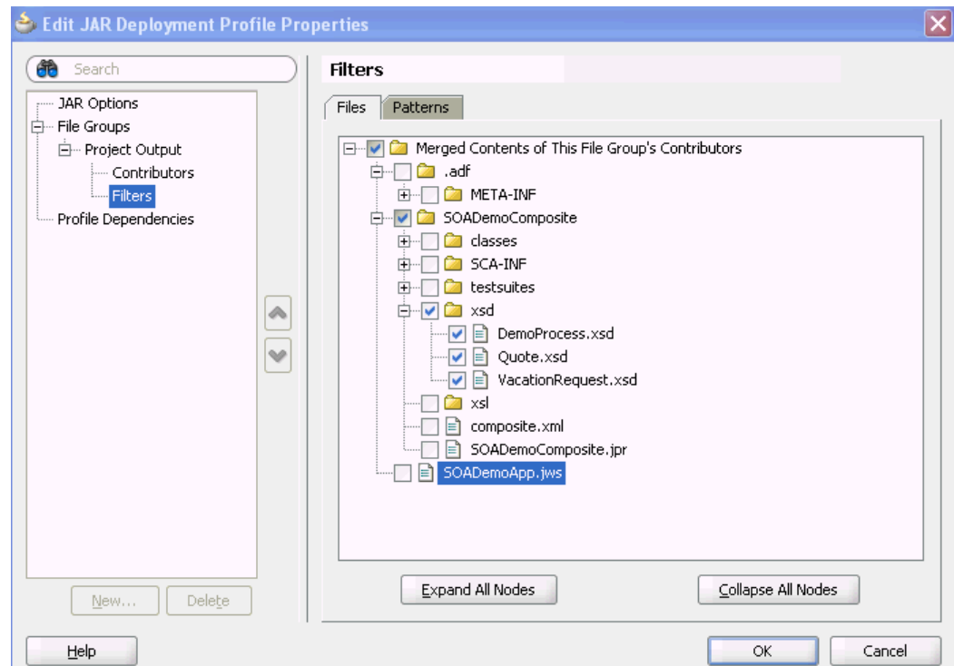
Figure 41–20 Artifacts to Include in the Archive
