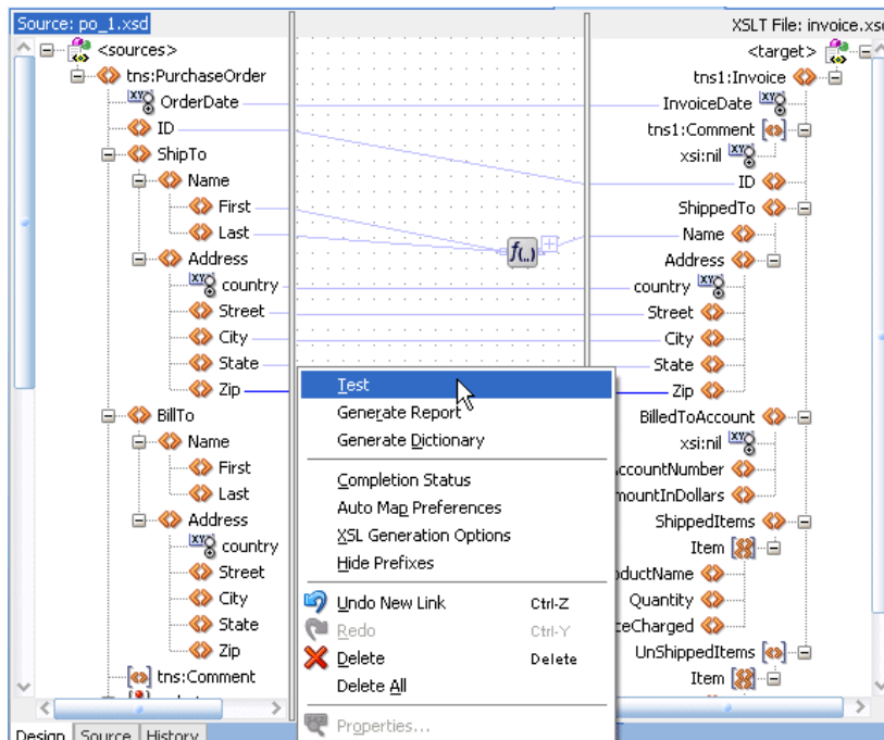
Figure 38–47 Invoking the Test Dialog
