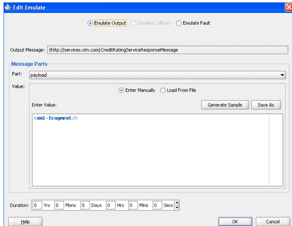
Figure 42–12 Emulate Dialog with Emulate Output Selected
