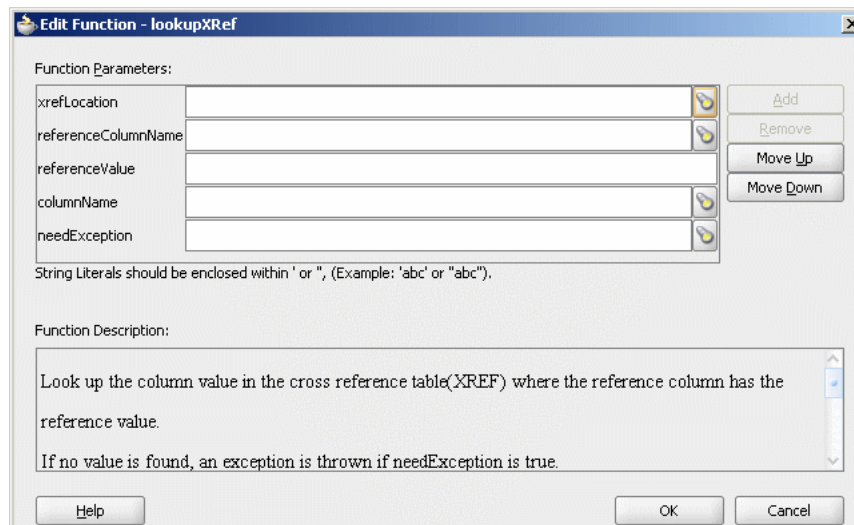
Figure 46–10 Edit Function – lookupXRef Dialog
