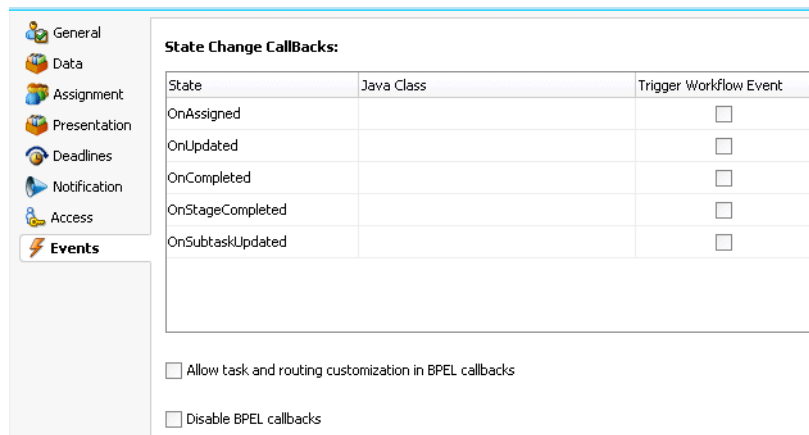
Figure 28–67 Callback Details Dialog with Java Selected
