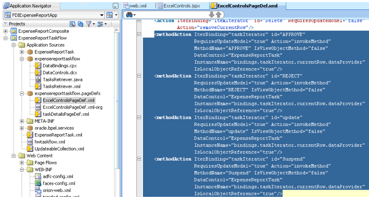
Figure 33–9 Oracle JDeveloper: Configuring the Page Definition File
