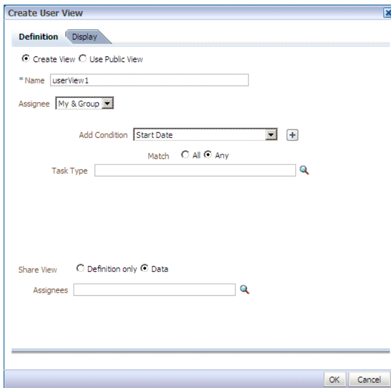
Figure 30–11 Creating a Worklist View
