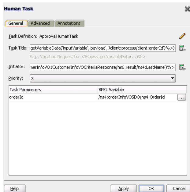
Figure 28–75 Human Task Dialog
