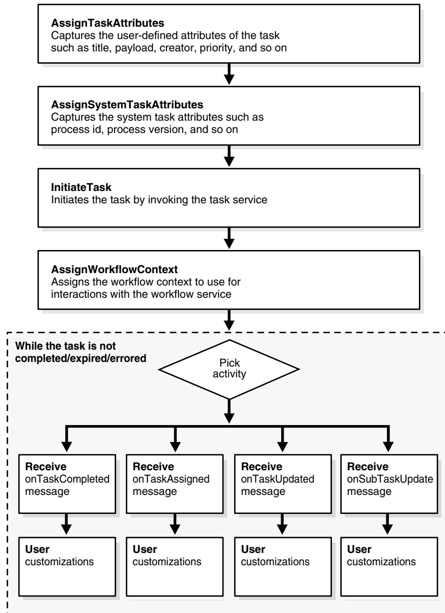
Figure 28–79 Workflow Interaction Modeling (with Callbacks)
