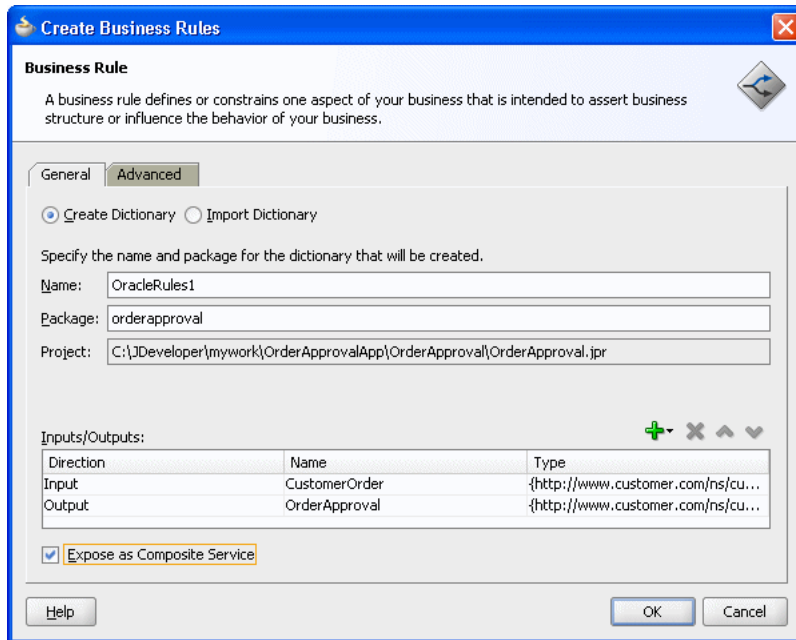
Figure 25–16 Create Business Rules Dialog with Input and Output
