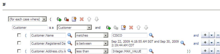
Figure 26–8 Nested Rules Support
