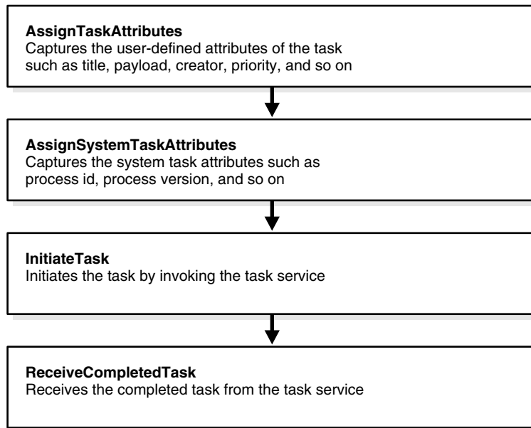
Figure 28–77 Workflow Interaction Modeling
