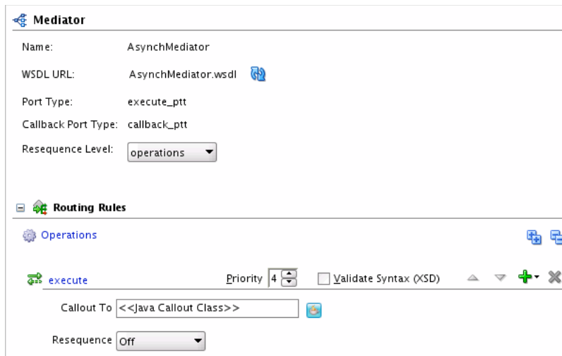
Figure 19–18 Asynchronous Oracle Mediator in the Mediator Editor
