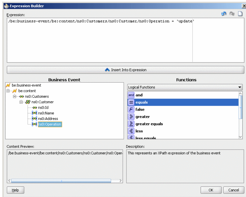
Figure 19–21 Business Event Filter
