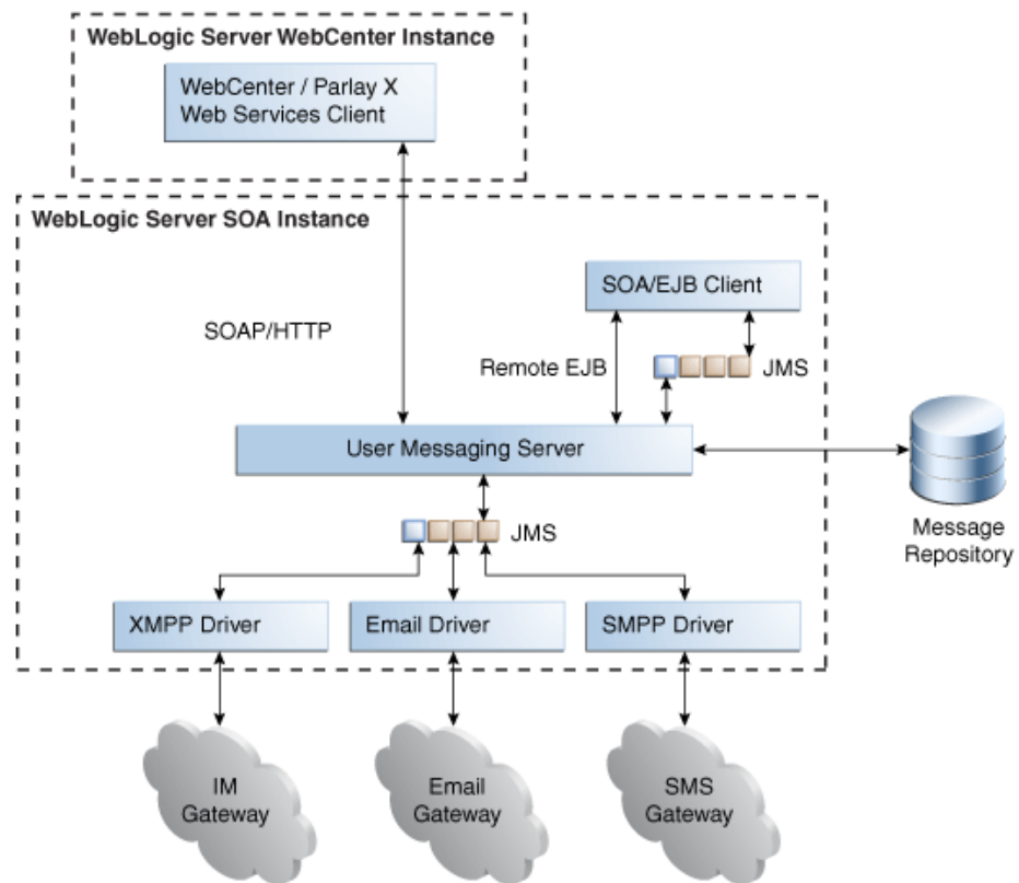
Figure 59-1 UMS architecture
