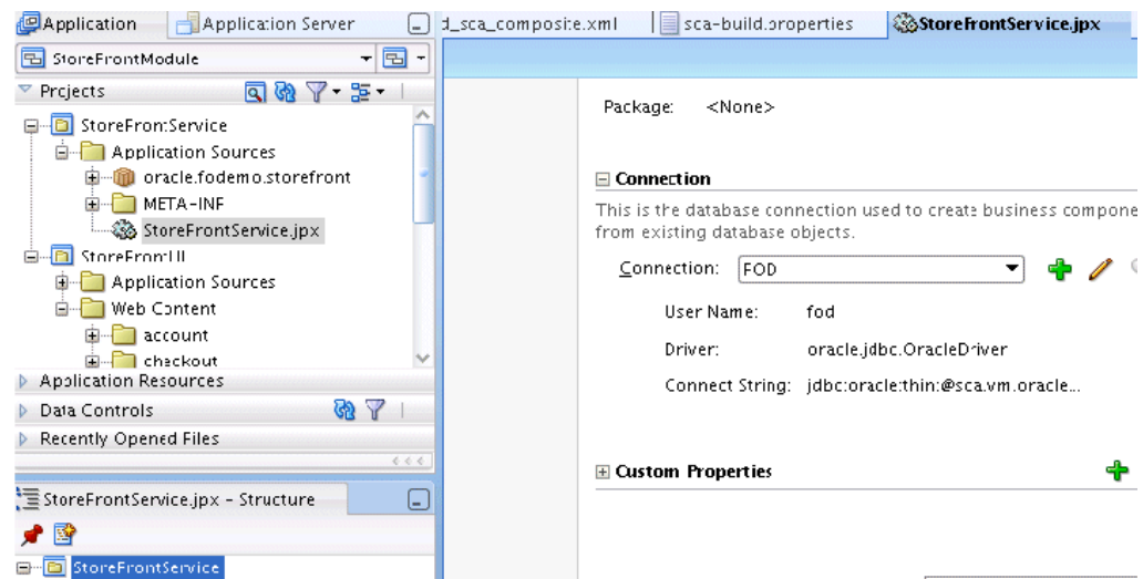
Figure 3–11 Connection
