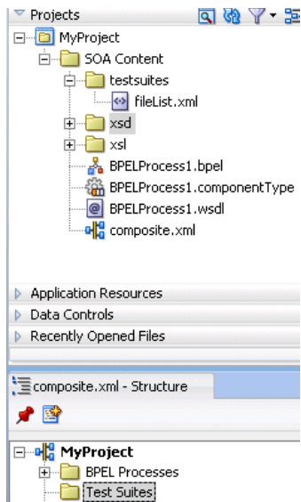
Figure 42–1 Structure Window
