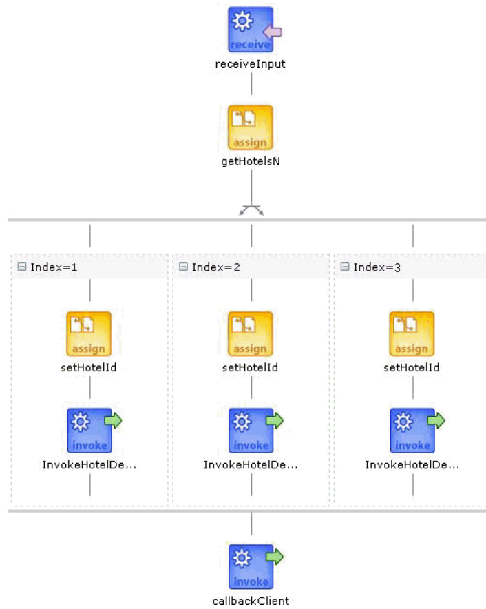
Figure 9–9 Oracle Enterprise Manager Fusion Middleware Control Console View of the Execution of a flowN activity
