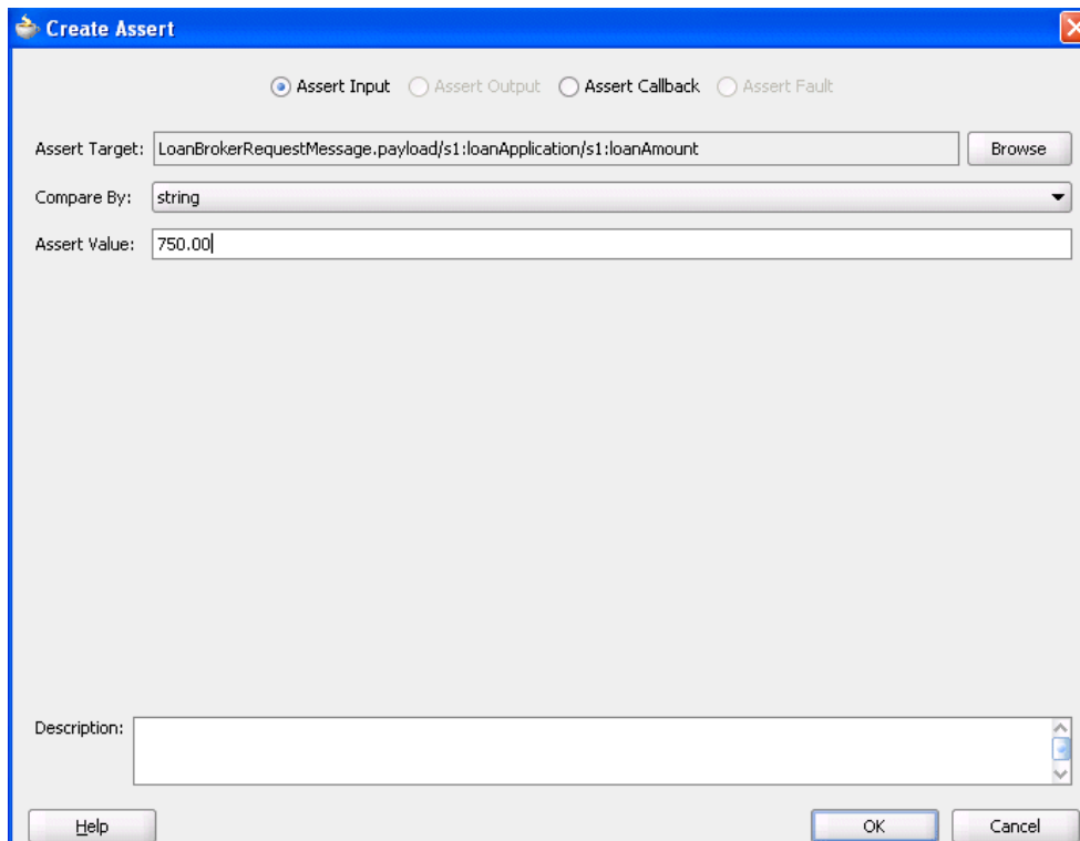
Figure 42–20 Create Assert Dialog
