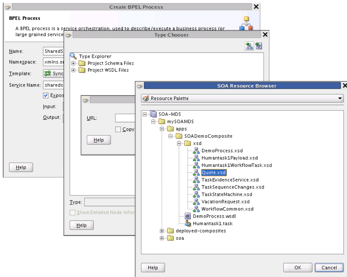
Figure 41–24 Shared Metadata in the SOA Resource Browser
