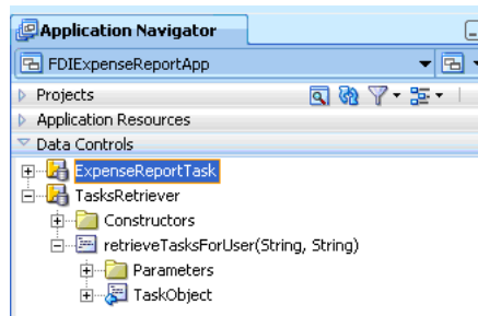
Figure 33–6 Oracle JDeveloper: Application Navigator with Data Control Palette Expanded
