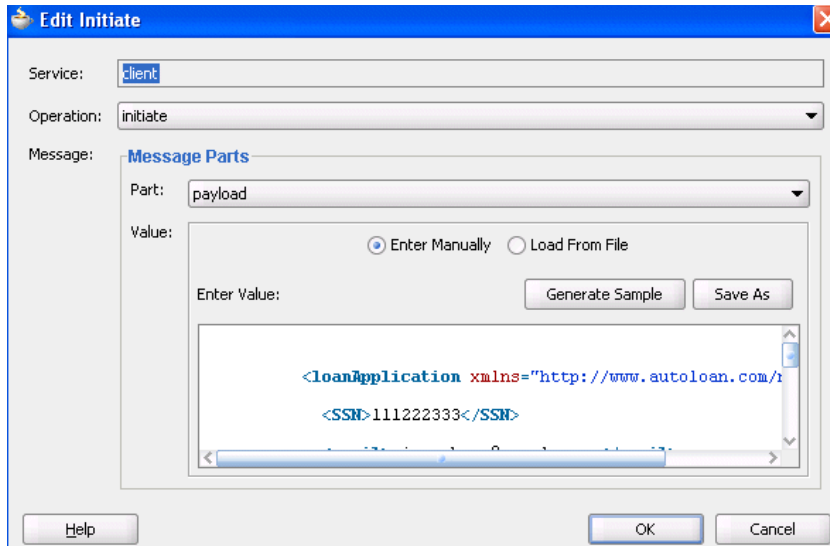
Figure 42–8 Edit Initiate Dialog
