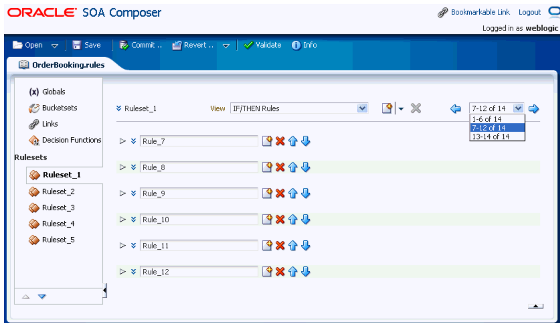
Figure 12–35 Rules Paging
