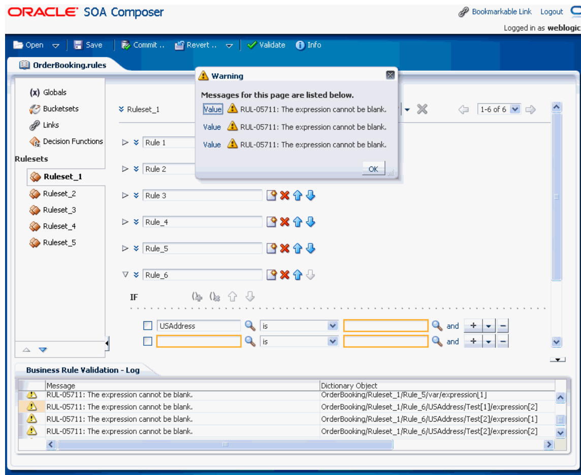
Figure 12–69 Rules Validation
