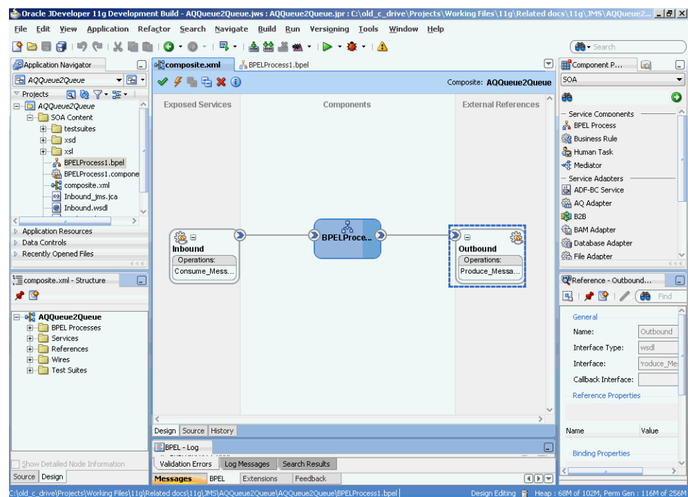
Figure 8–25 JDeveloper - Composite.xml
