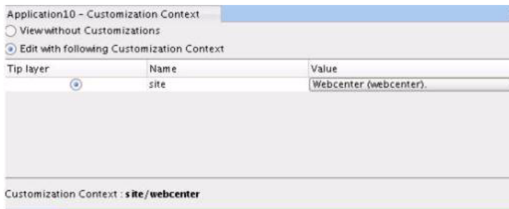
Figure 24–3 Customization Context
