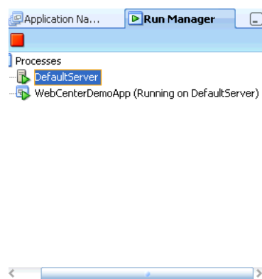
Figure 64-1 Run Manager
