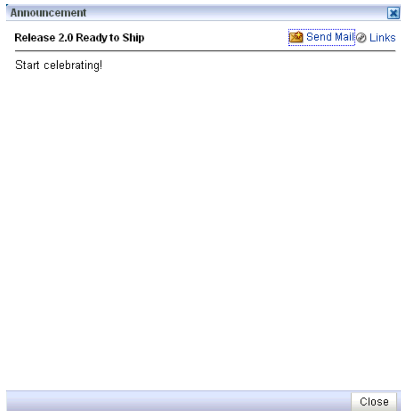
Figure 32–11 Announcement Popup
