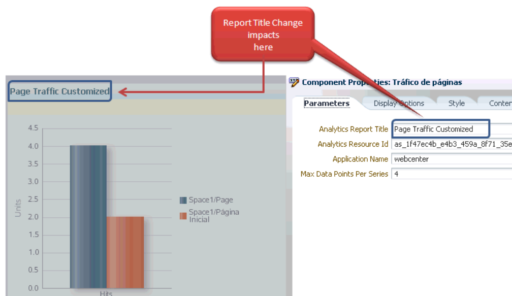
Figure 42–6 analyticsReportTitle - Example
