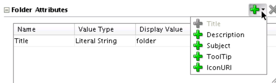
Figure 15-4 Folder Attributes
