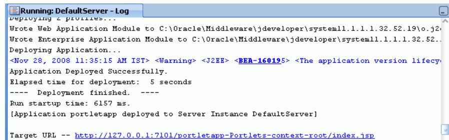
Figure 57-3 DefaultServer - Log
