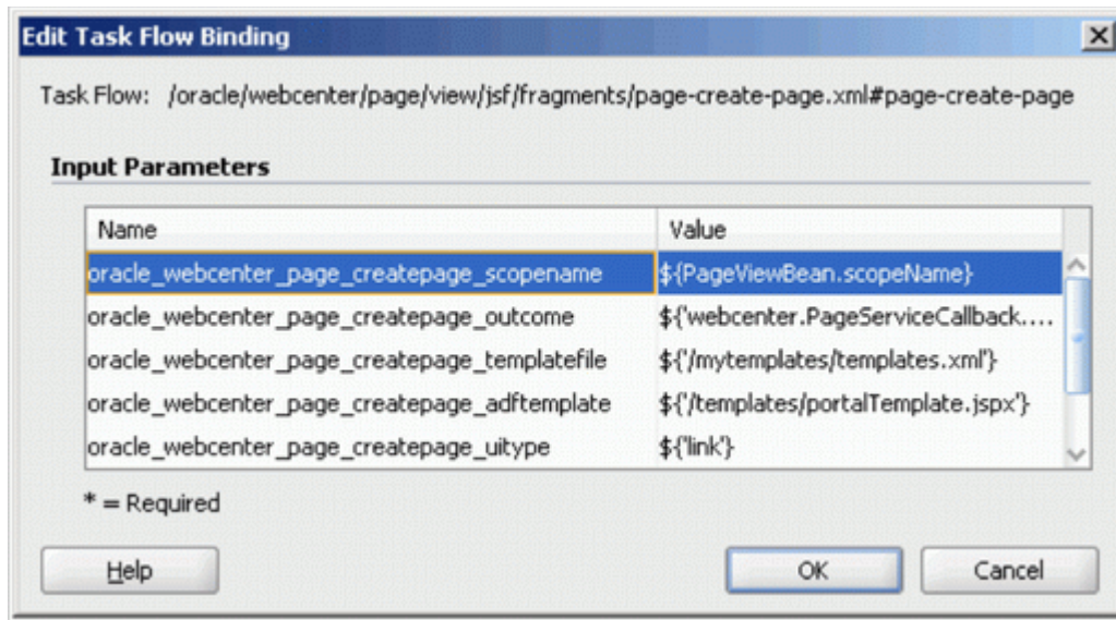
Figure 18–6 oracle_webcenter_page_createpage_scopename Parameter
