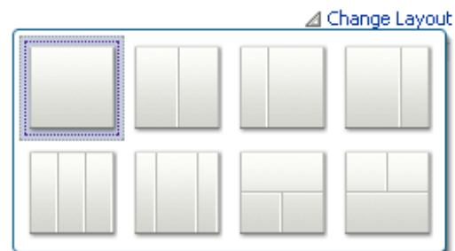
Figure 17-3 Layout Options
