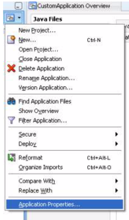
Figure 24–15 Application Properties
