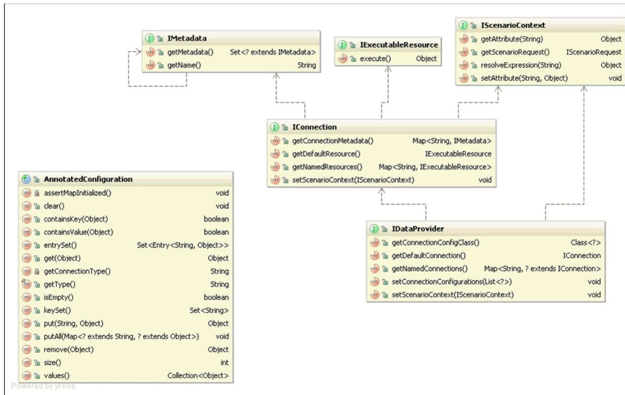
Figure 62–14 Class Interaction for Data Providers
