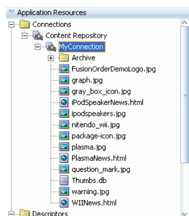
Figure 26–5 Application Resources
