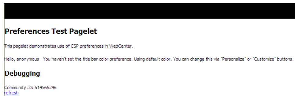
Figure 58–3 Sample Pagelet
