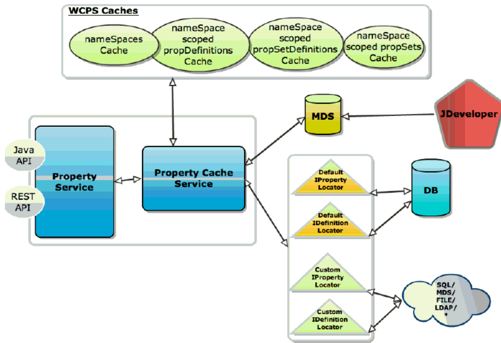
Figure 62–2 Property Service Architecture
